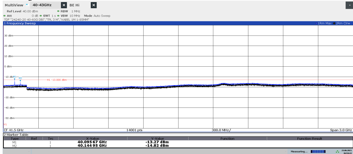
Diagram 2.12b: 40 – 43 GHz, QPSK, BL2 50 , EIRP Vertical polarization See diagram 2.12c for TRP result
