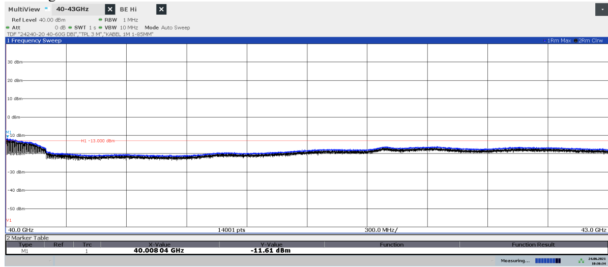
Diagram 2.11a: 40 – 43 GHz, QPSK, TH 8100 , EIRP Horizontal polarization See diagram 2.11e for TRP result
