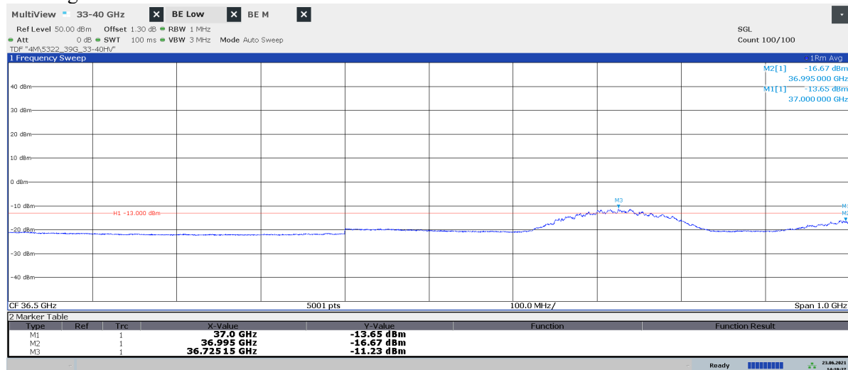
Diagram 2.7d: 36 – 37 GHz, QPSK, BTim6 50 , EIRP Vertical polarization See diagram 2.7e for TRP result
