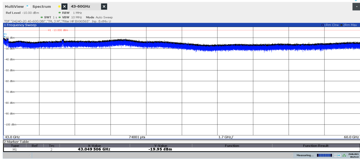
Diagram 2.13b: 43 – 60 GHz, QPSK, BL2 50 , EIRP Vertical polarization
