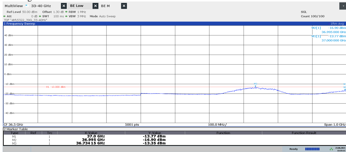
Diagram 2.7c: 36 – 37 GHz, QPSK, BTim6 50 , EIRP Horizontal polarization See diagram 2.7e for TRP result
