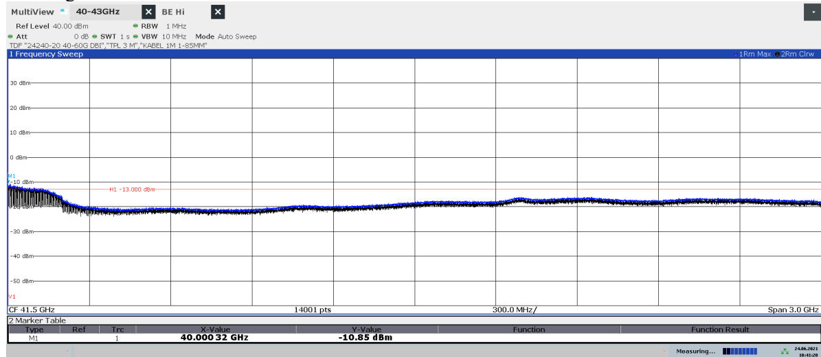
Diagram 2.11b: 40 – 43 GHz, QPSK, TH 8100 , EIRP Vertical polarization See diagram 2.11e for TRP result
