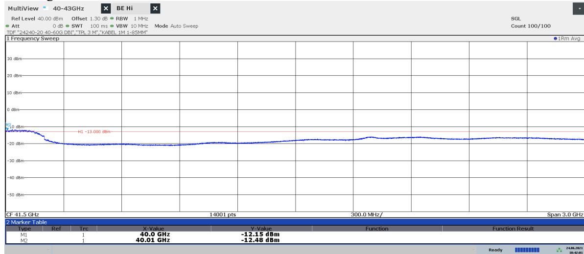
Diagram 2.11d: 40 – 43 GHz, QPSK, TH8 100 , EIRP Vertical polarization See diagram 2.11e for TRP result
