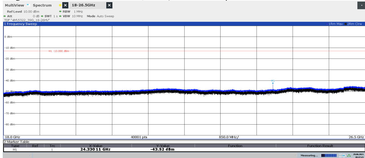
Diagram 2.3b: Pre scan 18 – 26.5 GHz, BL 250 , EIRP Vertical polarization
