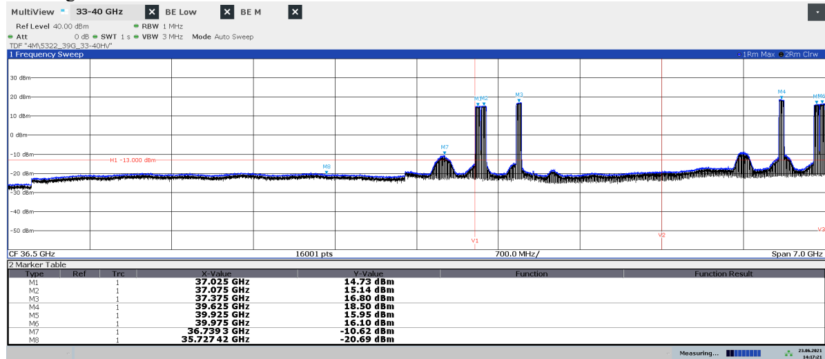
Diagram 2.7b: 33 – 40 GHz, QPSK, BTim6 50 , EIRP Vertical polarization See diagram 2.7e for TRP result
