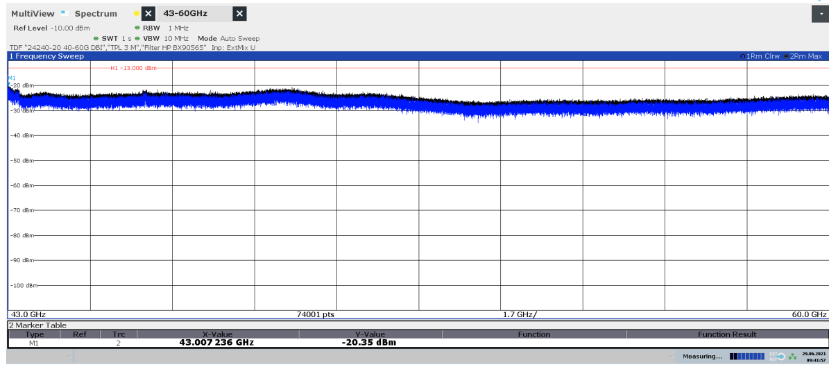
Diagram 2.13a: 43 – 60 GHz, QPSK, BL2 50 , EIRP Horizontal polarization
