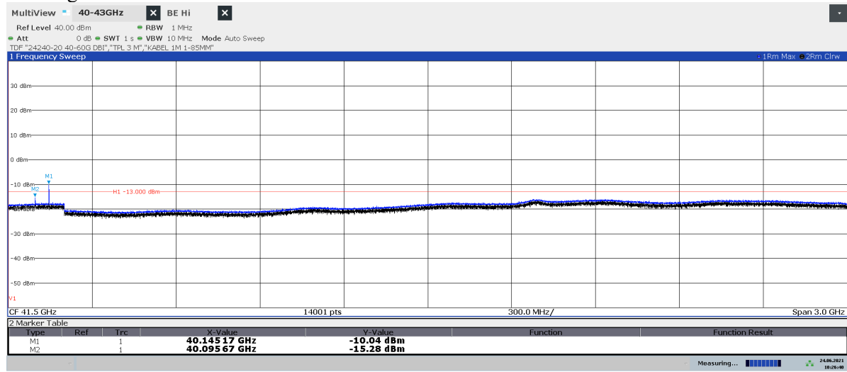
Diagram 2.12a: 40 – 43 GHz, QPSK, BL2 50 , EIRP Horizontal polarization See diagram 2.12c for TRP result
