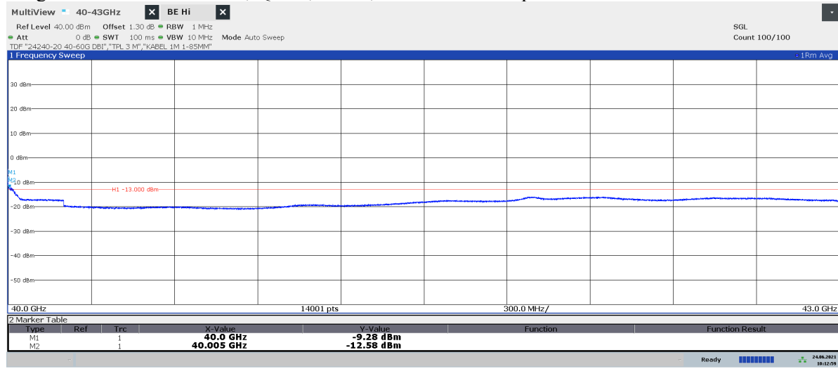
Diagram 2.10c: 40 – 43 GHz, QPSK, TH 250 , EIRP Horizontal polarization
