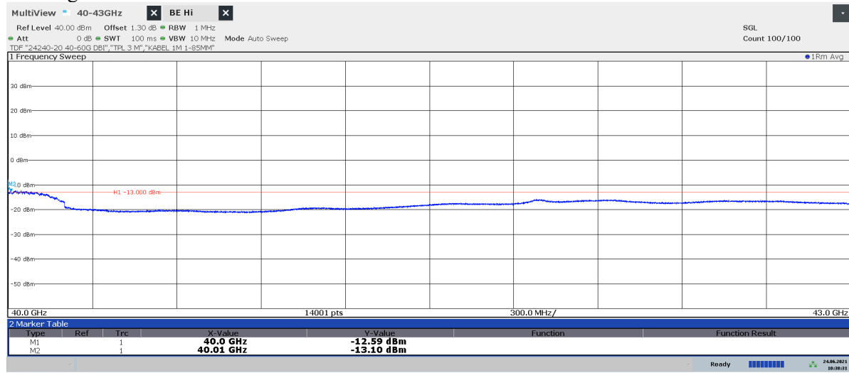
Diagram 2.11c: 40 – 43 GHz, QPSK, TH8 100 , EIRP Horizontal polarization See diagram 2.11e for TRP result
