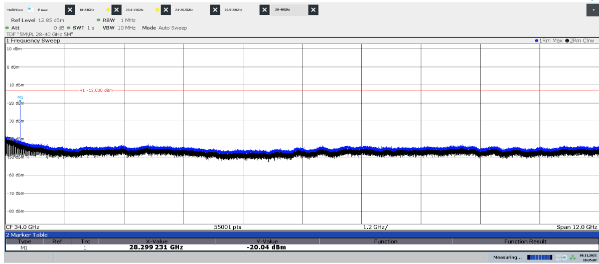
Diagram 2.13a: 28 – 40 GHz, QPSK, TH 50 , EIRP Horizontal polarization
