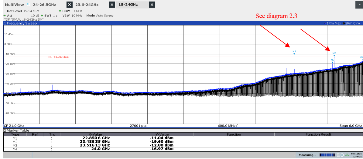
Diagram 2.19a: 18 – 24 GHz, QPSK, BT 850 , EIRP Horizontal polarization
