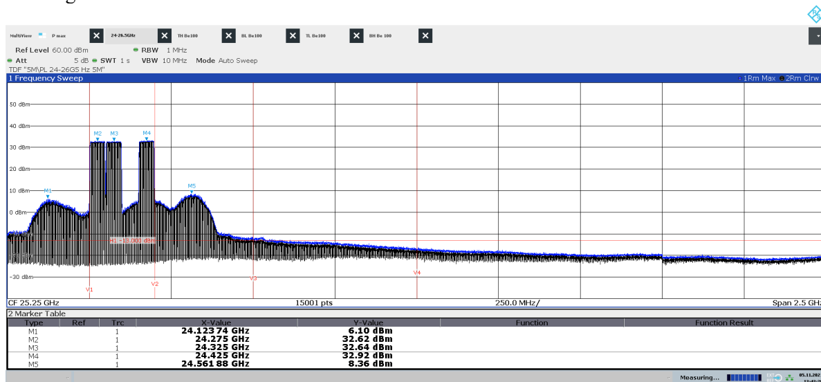
Diagram 2.7a: Pre scan 24 – 26.5 GHz, BimL 50 , EIRP Horizontal polarization See diagram 2.7e for TRP result
