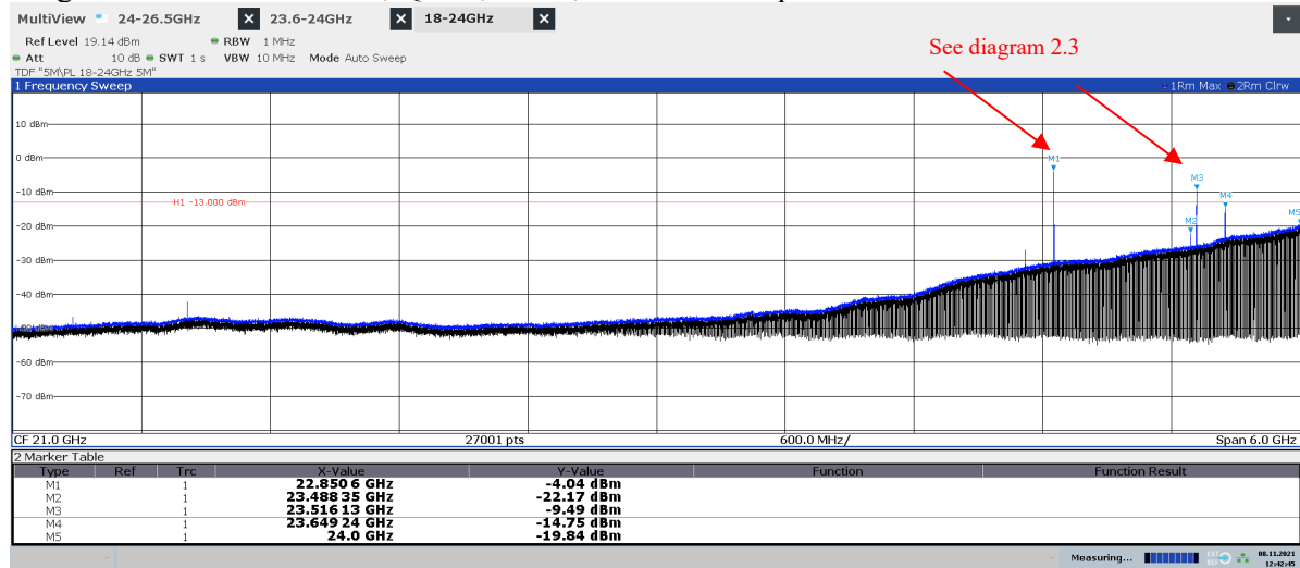
Diagram 2.19b: 18 – 24 GHz, QPSK, BT 850 , EIRP Vertical polarization
