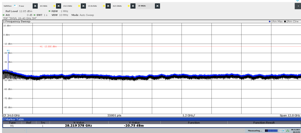
Diagram 2.22b: 28 – 40 GHz, QPSK, BT8 50 , EIRP Vertical polarization
