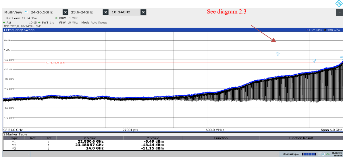
Diagram 2.4a: Pre scan 18 – 24 GHz, BimL 50 , EIRP Horizontal polarization See diagram 2.4c for TRP result
