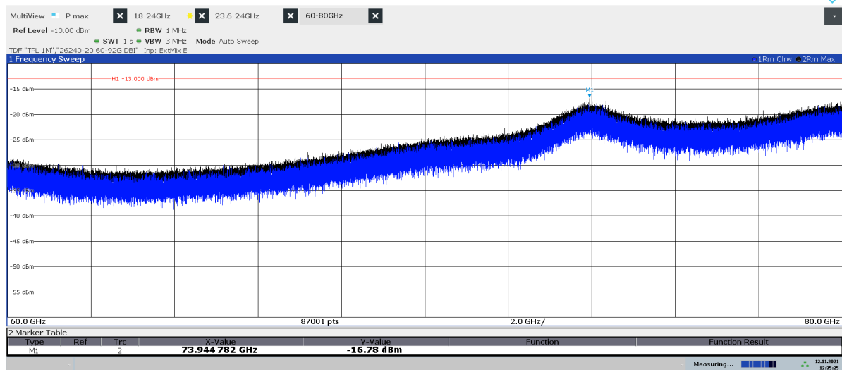
Diagram 2.15b: 60 – 80 GHz, QPSK, BH 50 , EIRP Vertical polarization
