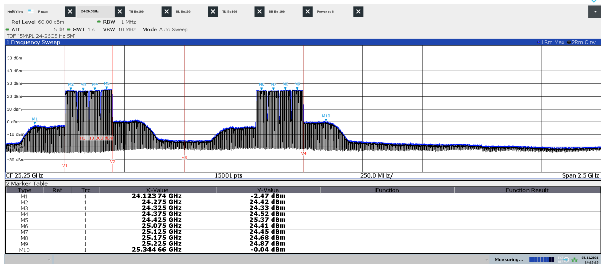
Diagram 2.20b: 24 – 26.5 GHz, QPSK, BT8 50 , EIRP Vertical polarization
