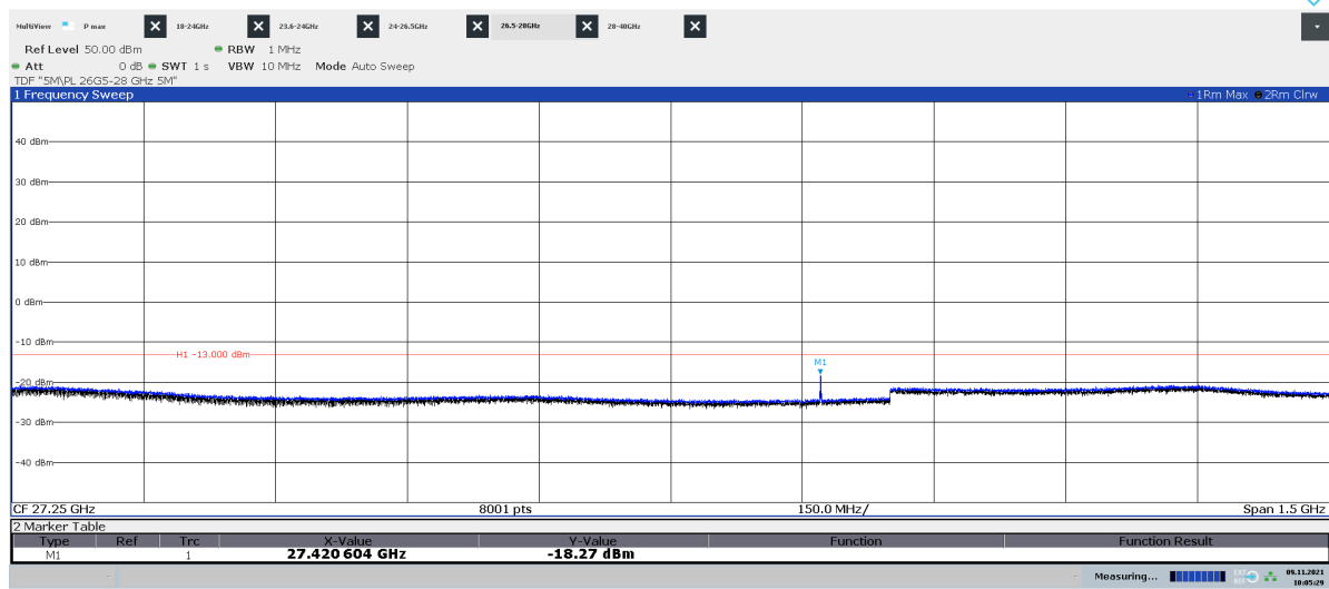
Diagram 2.21a: 26 – 28 GHz, QPSK, BT8 50 , EIRP Vertical polarization
