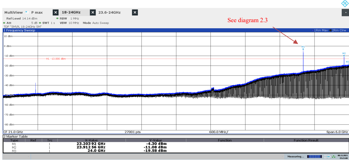
Diagram 2.5a: Pre scan 18 – 24 GHz, BimL 50 , EIRP Horizontal polarization See diagram 2.5c for TRP result
