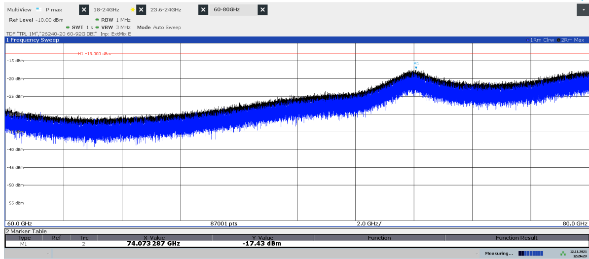
Diagram 2.24a: 60 – 80 GHz, QPSK, BT8 50 , EIRP Horizontal polarization
