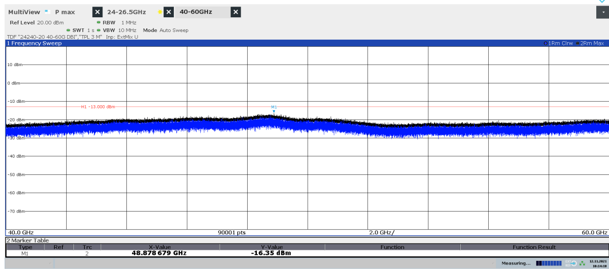
Diagram 2.23b: 40 – 60 GHz, QPSK, BT8 50 , EIRP Vertical polarization
