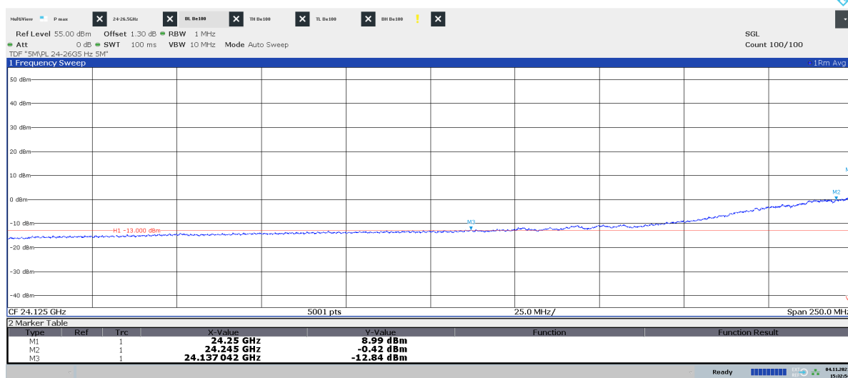
Diagram 2.6c: 24 – 24.25 GHz, QPSK, BL 50 , EIRP Horizontal polarization
