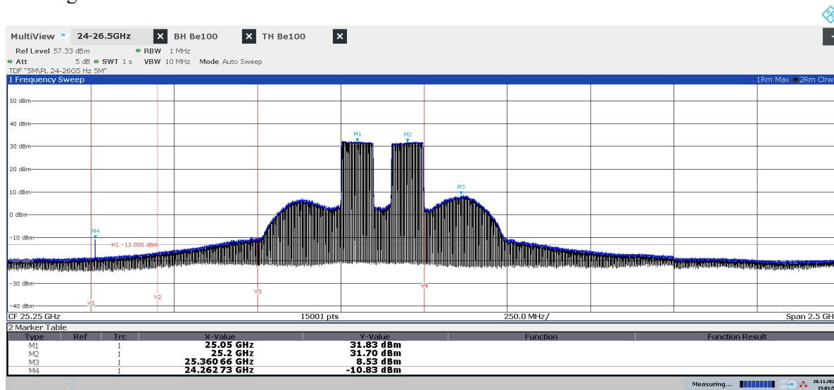
Diagram 2.11a: Pre scan 24 – 26.5 GHz, TH 2100 , EIRP Horizontal polarization See diagram 2.11e for TRP result
