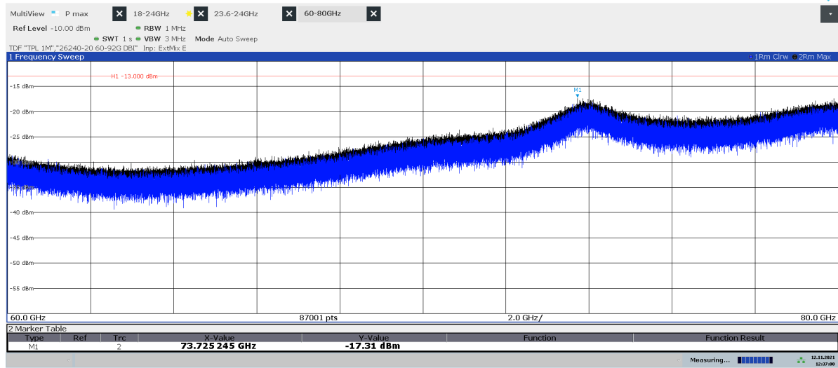
Diagram 2.15a: 60 – 80 GHz, QPSK, BH 50 , EIRP Horizontal polarization
