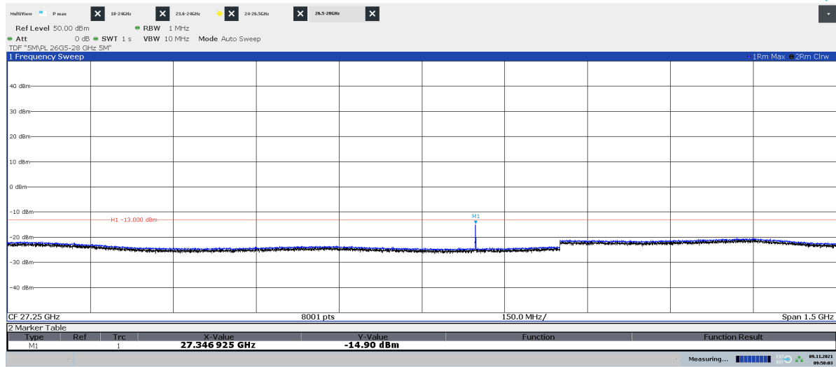
Diagram 2.12a: 26.5 – 28 GHz, QPSK, BL 50 , EIRP Horizontal polarization
