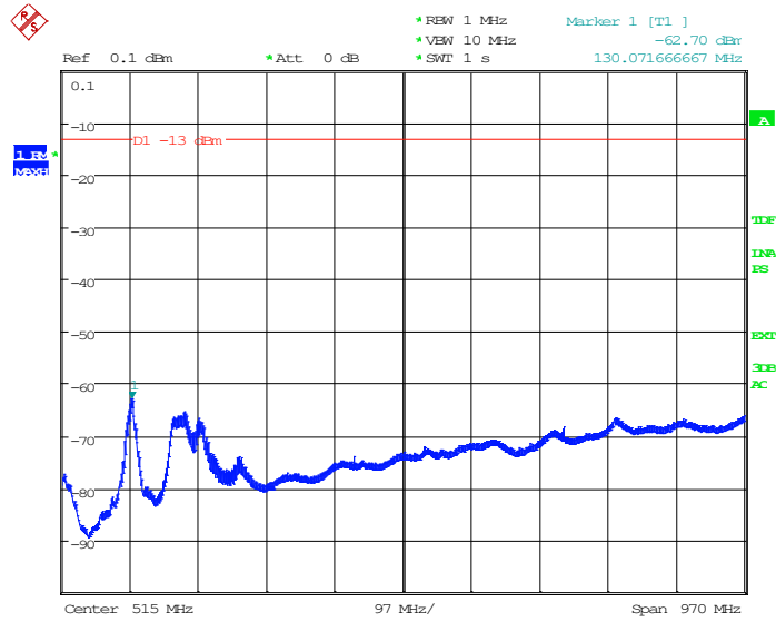
Diagram 2.17a: 30 – 1000 MHz, QPSK, BT8 50 , EIRP Horizontal polarization
