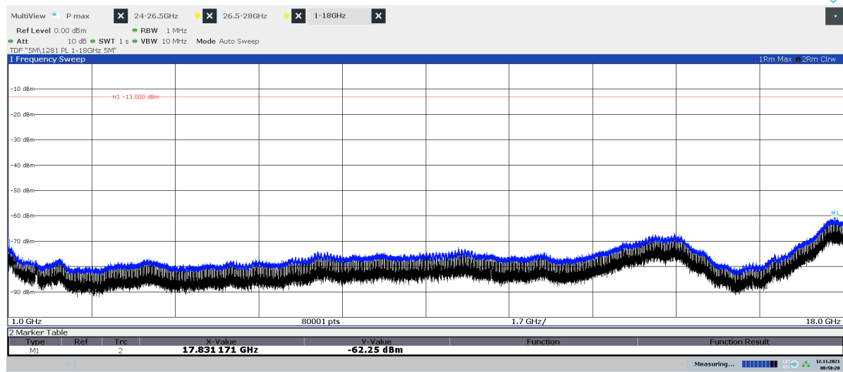
Diagram 2.2b: Pre scan 1 – 18 GHz, BH 50 , EIRP Vertical polarization
