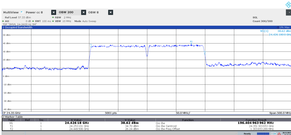
Diagram 1.10, Symbolic name: CA6 100 , QPSK, Vertical: Lower 200MHz
