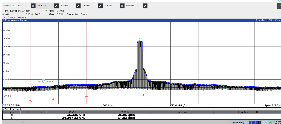
Diagram 2.10b: Pre scan 24 – 26.5 GHz, TH 50 , EIRP Vertical polarization
