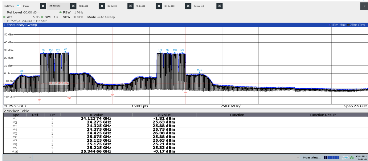
Diagram 2.20a: 24 – 26.5 GHz, QPSK, BT8 50 , EIRP Horizontal polarization
