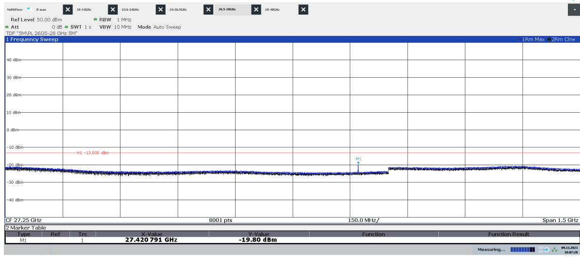
Diagram 2.21a: 26 – 28 GHz, QPSK, BT8 50 , EIRP Horizontal polarization
