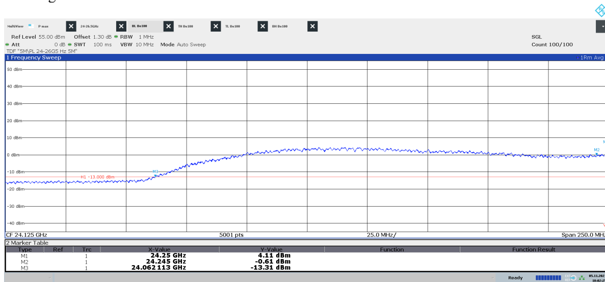
Diagram 2.7c: 24 – 24.25 GHz, QPSK, BimL 50 , EIRP Horizontal polarization See diagram 2.7e for TRP result
