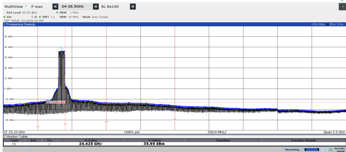
Diagram 2.8b: Pre scan 24 – 26.5 GHz, TL 50 , EIRP Vertical polarization
