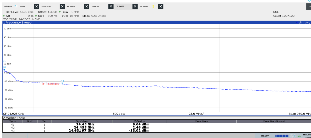
Diagram 2.8c: 24.45 – 25.4 GHz, QPSK, TL 50 , EIRP Horizontal polarization
