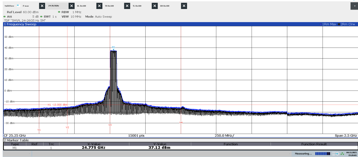
Diagram 2.9a: Pre scan 24 – 26.5 GHz, BH 50 , EIRP Horizontal polarization
