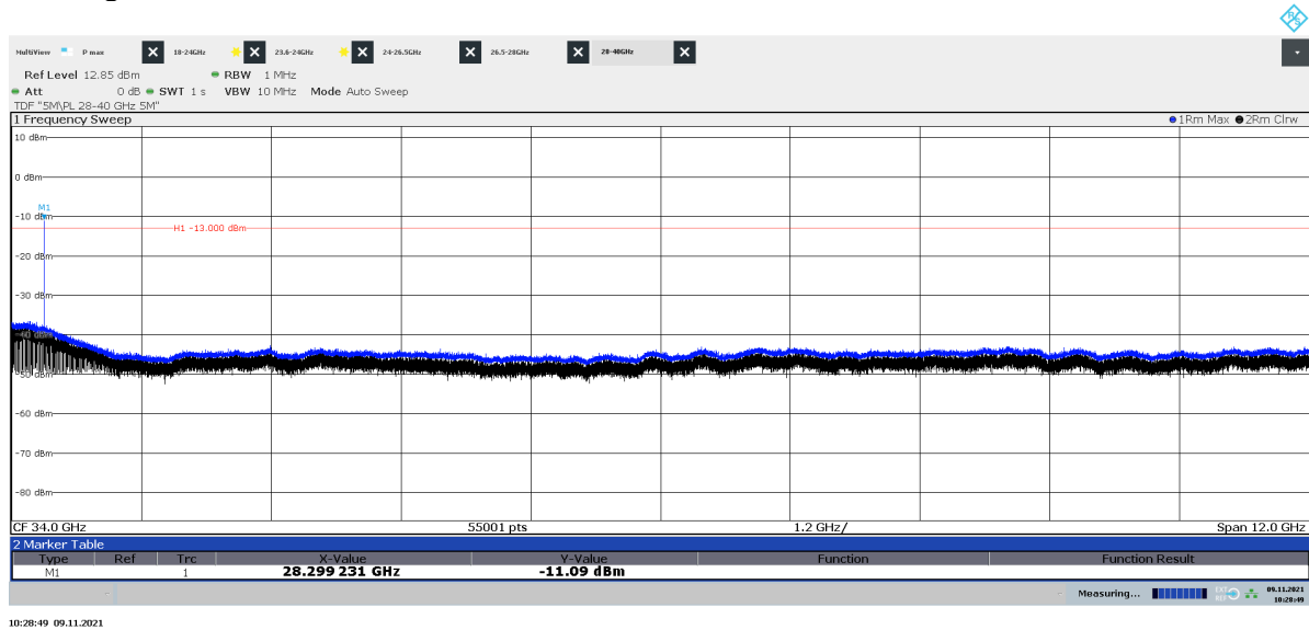
Diagram 2.13b: 28 – 40 GHz, QPSK, TH 50 , EIRP Vertical polarization See diagram 2.13c for TRP result
