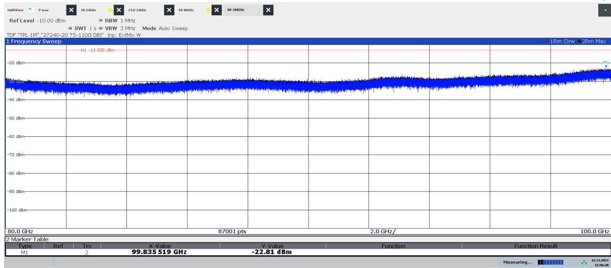
Diagram 2.25a: 80 – 100 GHz, QPSK, BT8 50 , EIRP Horizontal polarization
