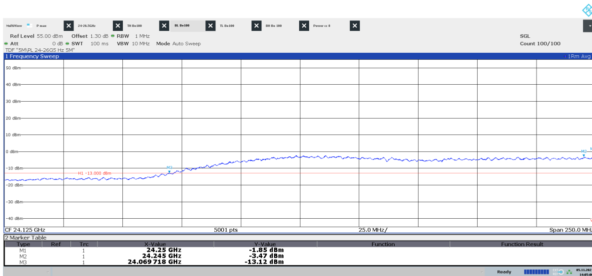
Diagram 2.20c: 24 – 24.25 GHz, QPSK, BT8 50 , EIRP Horizontal polarization
