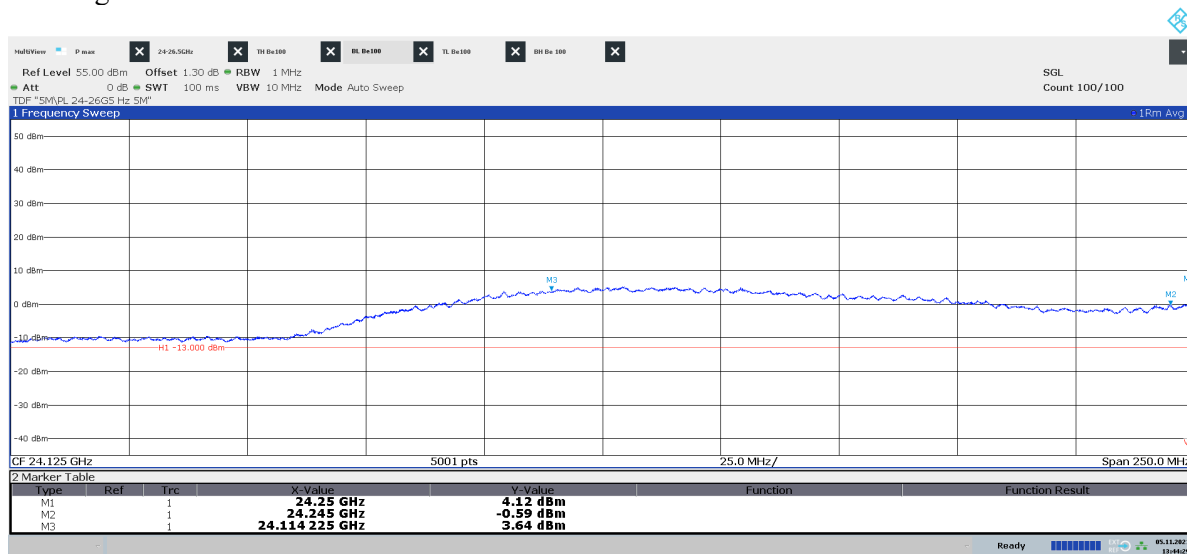
Diagram 2.7d: 24 – 24.25 GHz, QPSK, BimL 50 , EIRP Vertical polarization See diagram 2.7e for TRP result
