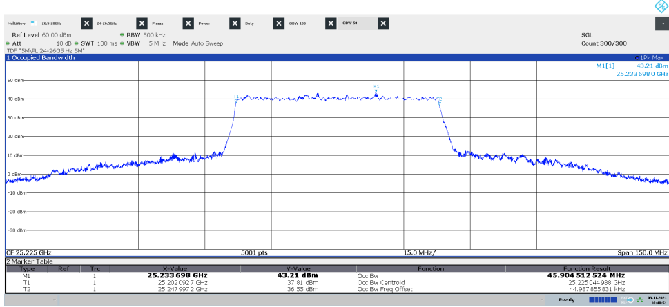
Diagram 1.2, Symbolic name: TH 50 , QPSK, Vertical:
