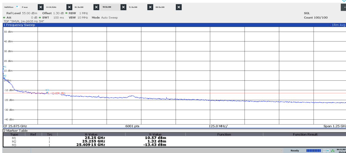
Diagram 2.10c: 25.25 – 26.5 GHz, QPSK, TH 50 , EIRP Horizontal polarization
