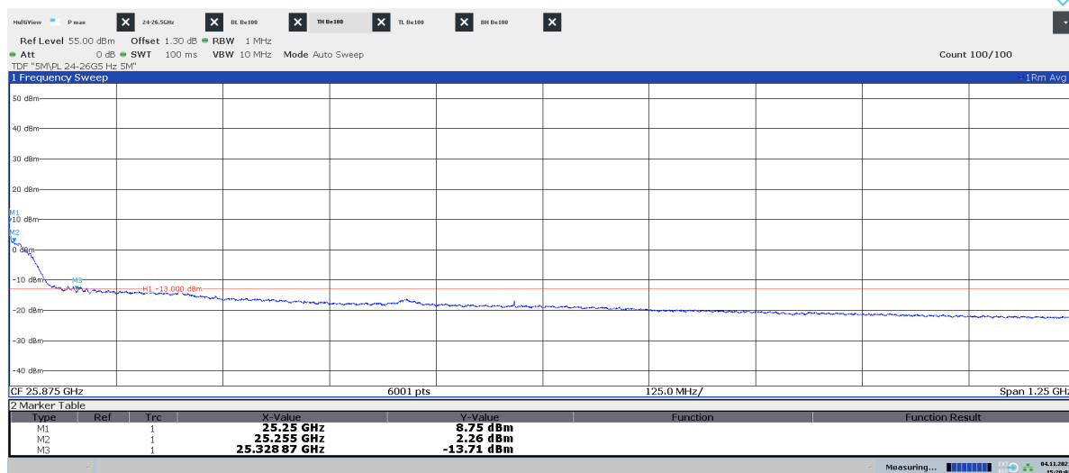
Diagram 2.10d: 25.25 – 26.5 GHz, QPSK, TH 50 , EIRP Vertical polarization
