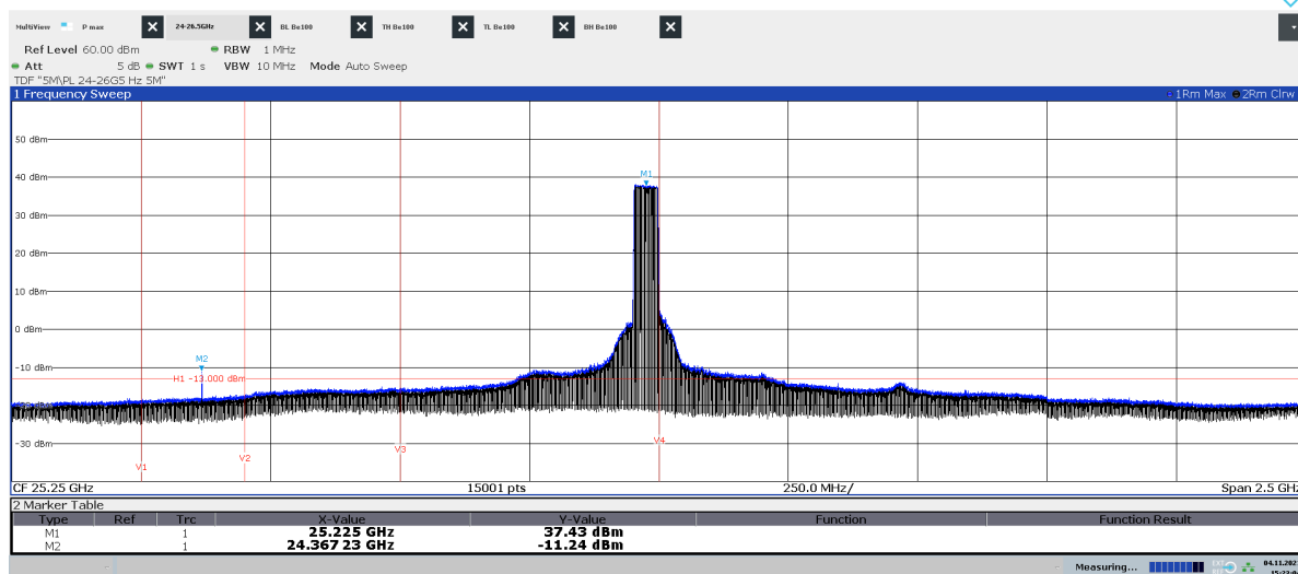
Diagram 2.10a: Pre scan 24 – 26.5 GHz, TH 50 , EIRP Horizontal polarization
