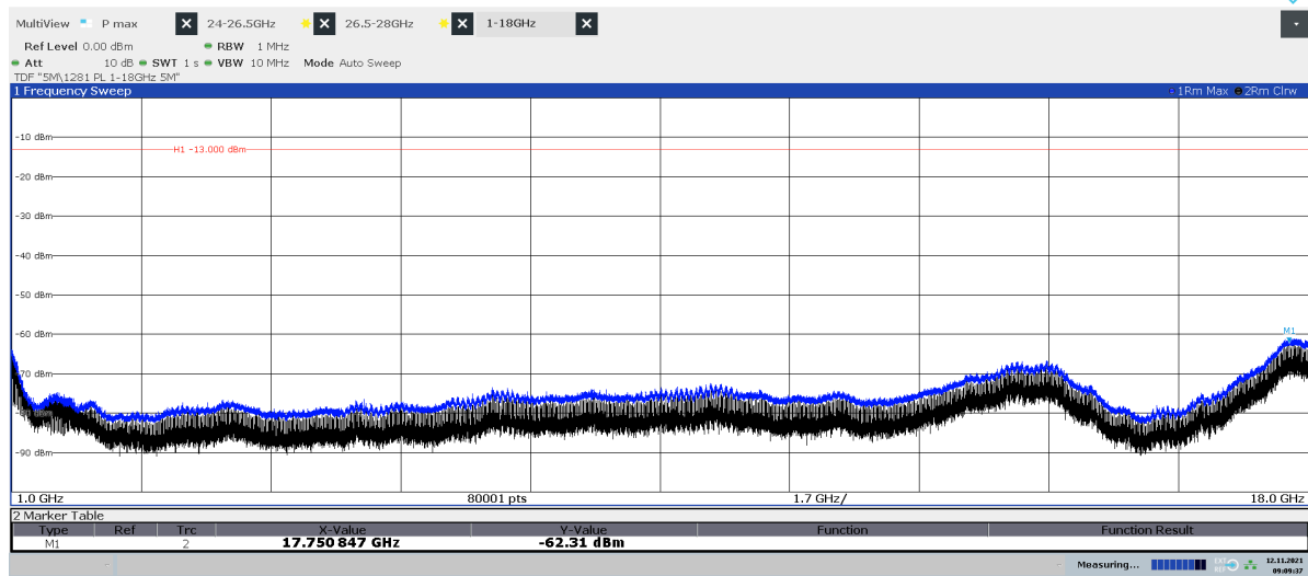
Diagram 2.18b: 1 – 18 GHz, QPSK, BT8 50 , EIRP Vertical polarization
