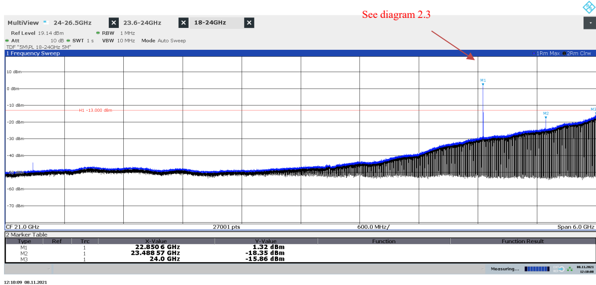
Diagram 2.4b: Pre scan 18 – 24 GHz, BimL 50 , EIRP Vertical polarization See diagram 2.4c for TRP result
