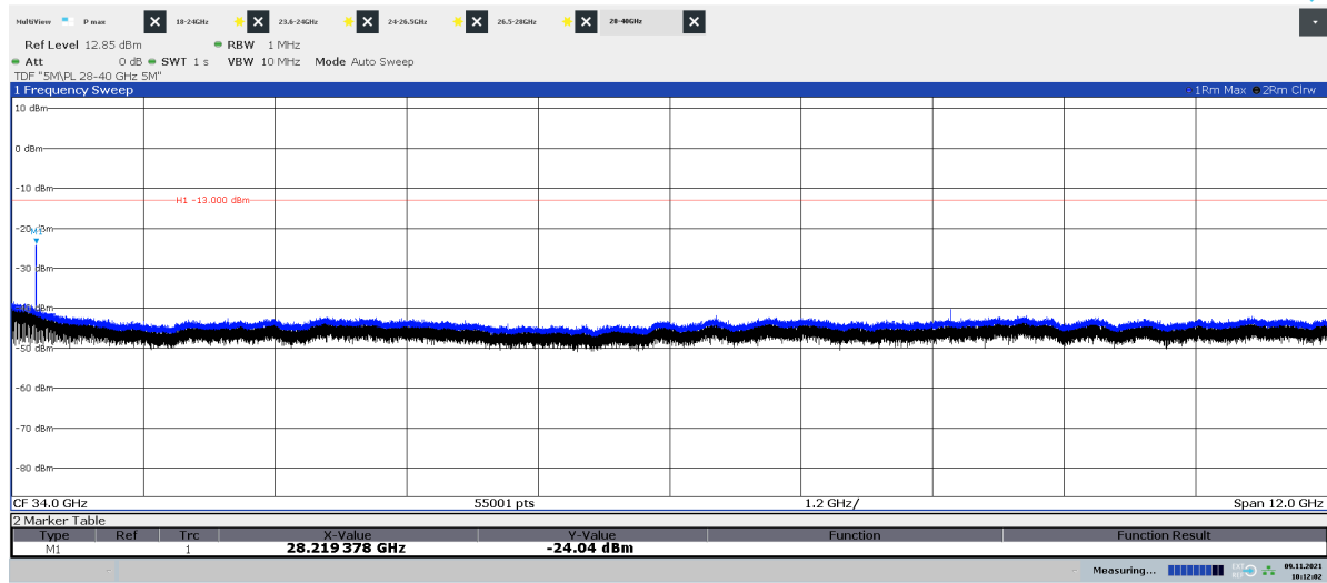
Diagram 2.22a: 28 – 40 GHz, QPSK, BT8 50 , EIRP Horizontal polarization
