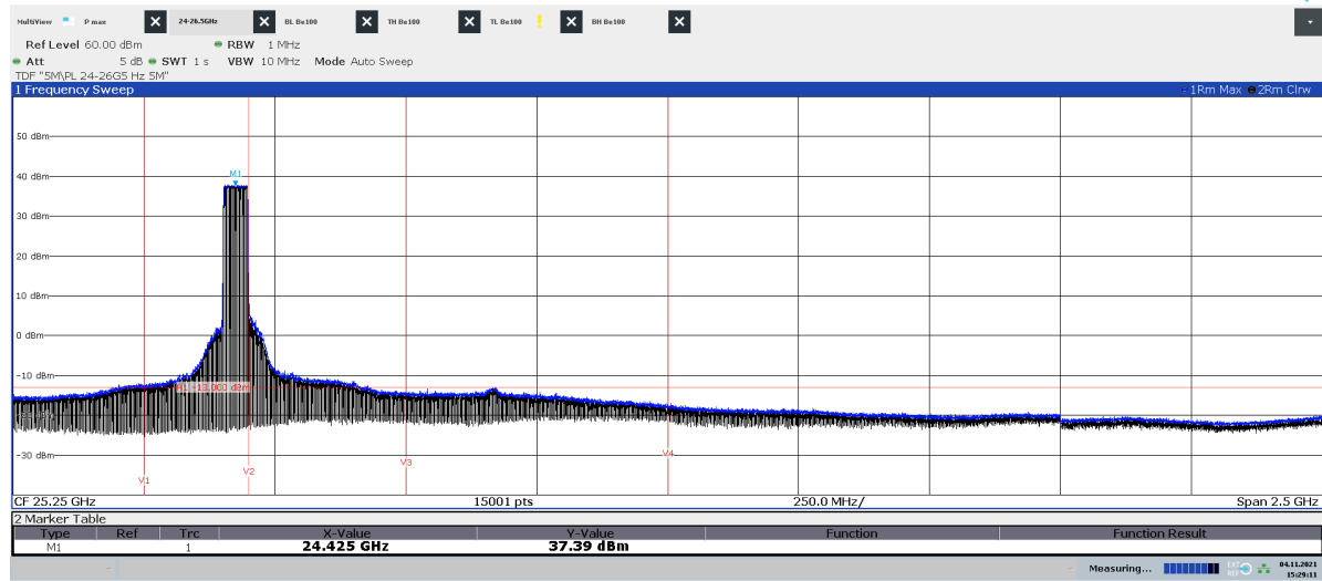
Diagram 2.8a: Pre scan 24 – 26.5 GHz, TL 50 , EIRP Horizontal polarization
