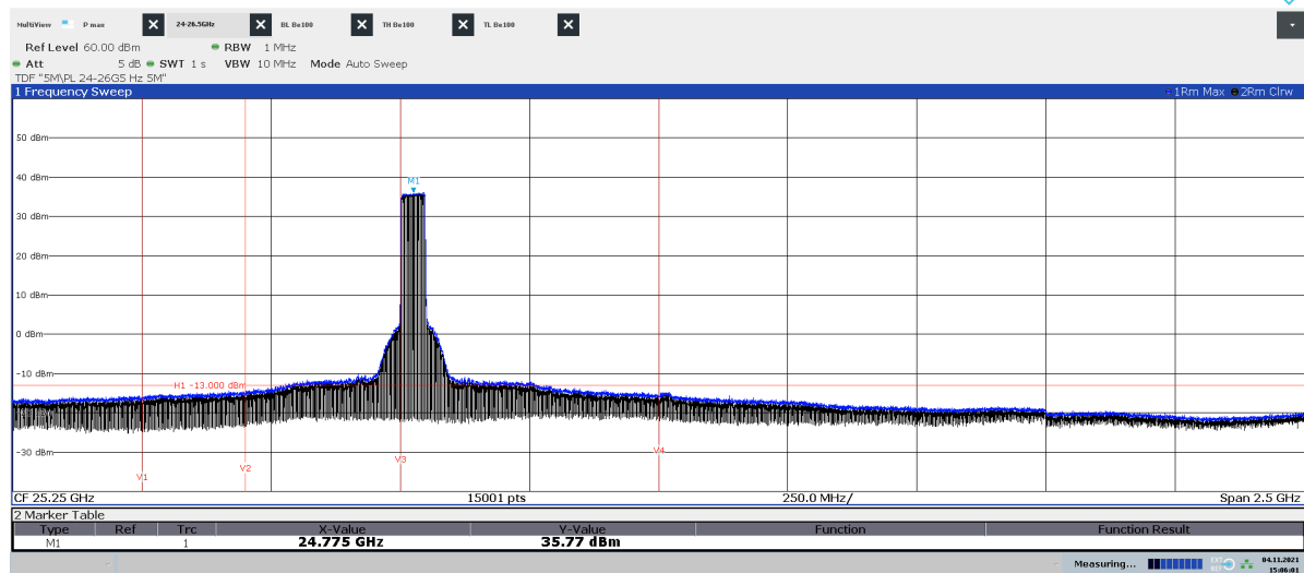
Diagram 2.9b: Pre scan 24 – 26.5 GHz, BH 50 , EIRP Vertical polarization
