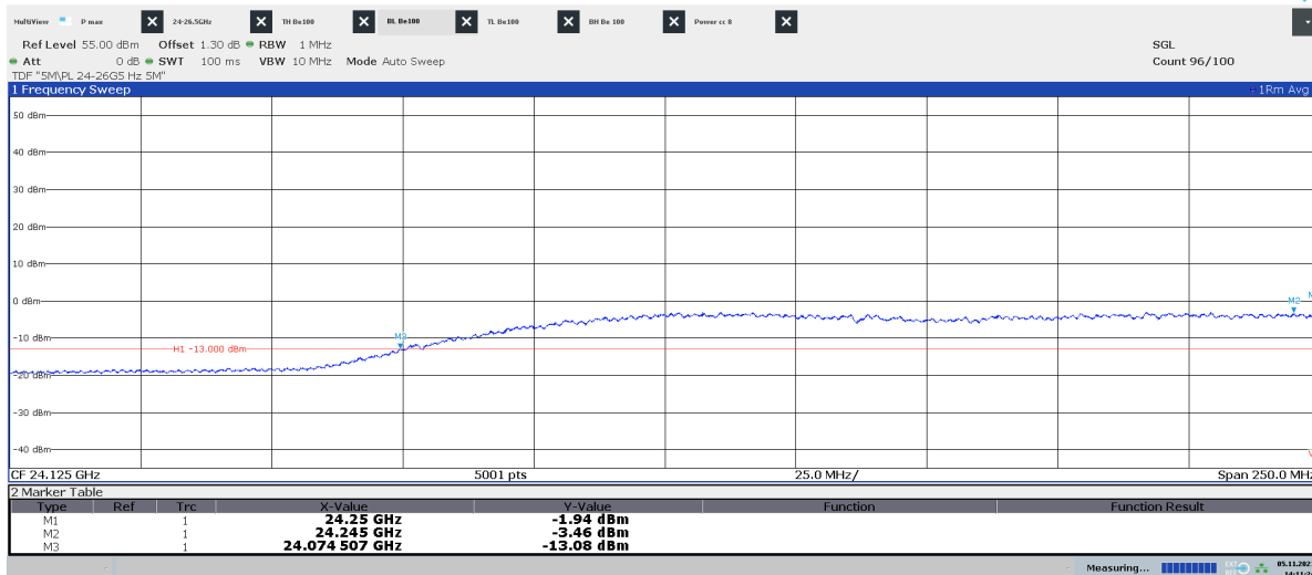
Diagram 2.20d: 24 – 24.25 GHz, QPSK, BT8 50 , EIRP Vertical polarization
