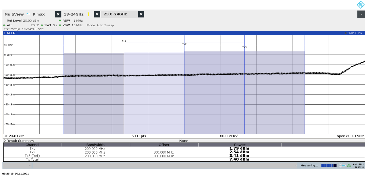
Diagram 2.4e: Pre scan Channel power 200MHz 23.6 – 24 GHz, BimL 50 , EIRP Vertical polarization See diagram 2.4f for TRP result
