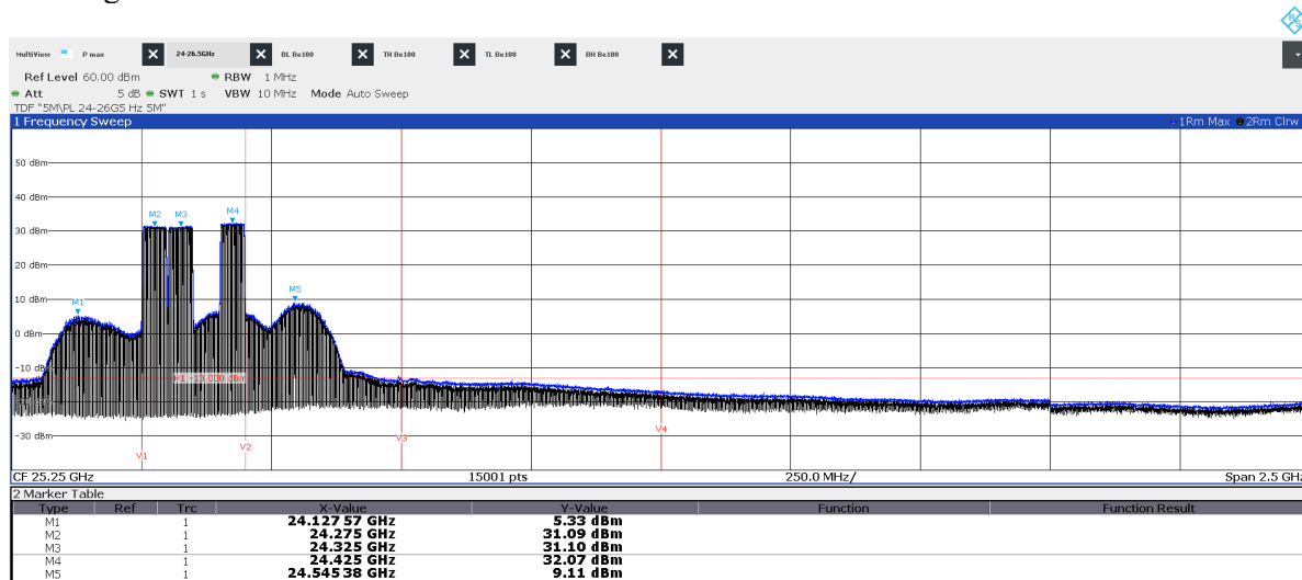
Diagram 2.7b: Pre scan 24 – 26.5 GHz, BimL 50 , EIRP Vertical polarization See diagram 2.7e for TRP result
