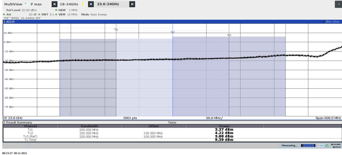
Diagram 2.4d: Pre scan Channel power 200MHz 23.6 – 24 GHz, BimL 50 , EIRP Horizontal polarization See diagram 2.4f for TRP result
