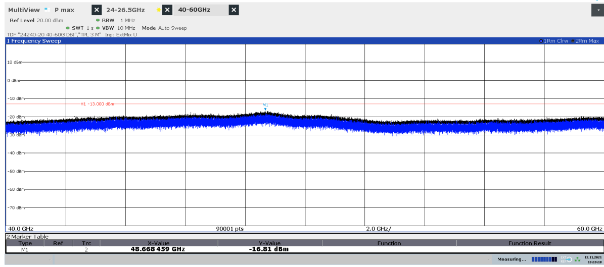
Diagram 2.23a: 40 – 60 GHz, QPSK, BT8 50 , EIRP Horizontal polarization
