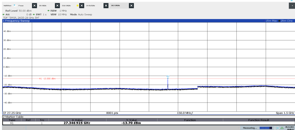
Diagram 2.12b: 26.5 – 28 GHz, QPSK, BL 50 , EIRP Vertical polarization
