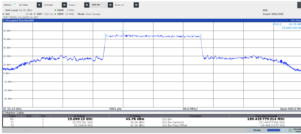
Diagram 1.5, Symbolic name: TH 200 , QPSK, Horizontal:
