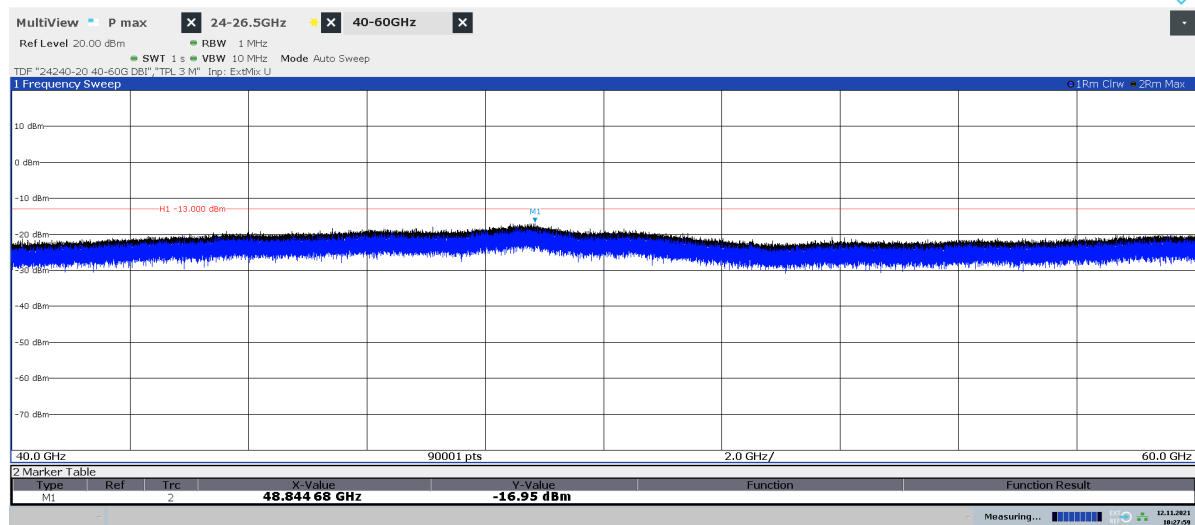
Diagram 2.14b: 40 – 60 GHz, QPSK, BH 50 , EIRP Vertical polarization
