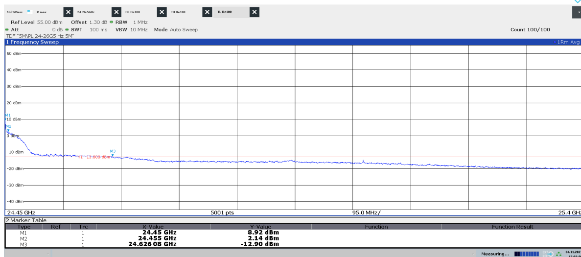
Diagram 2.8d: 24.45 – 25.4 GHz, QPSK, TL 50 , EIRP Vertical polarization
