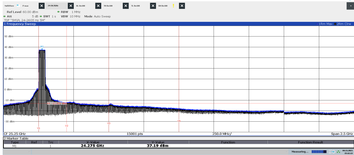
Diagram 2.6a: Pre scan 24 – 26.5 GHz, BL 50 , EIRP Horizontal polarization
