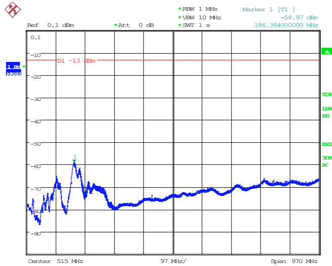
Diagram 2.17b: 30 – 1000 MHz, QPSK, BT8 50 , EIRP Vertical polarization
