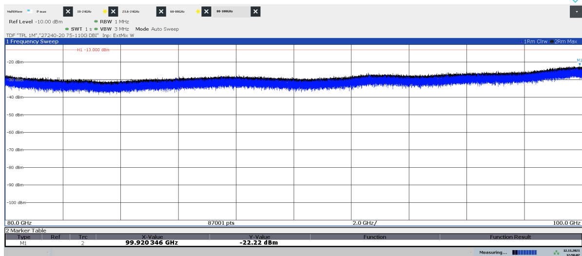
Diagram 2.25b: 80 – 100 GHz, QPSK, BT8 50 , EIRP Vertical polarization
