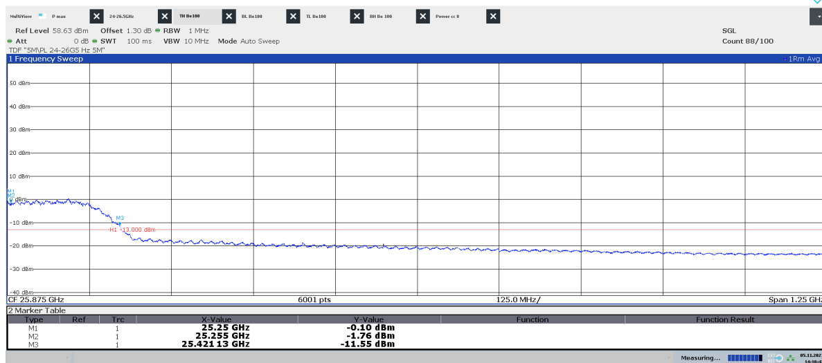
Diagram 2.20f: 25.25 – 26.5 GHz, QPSK, BT8 50 , EIRP Vertical polarization
