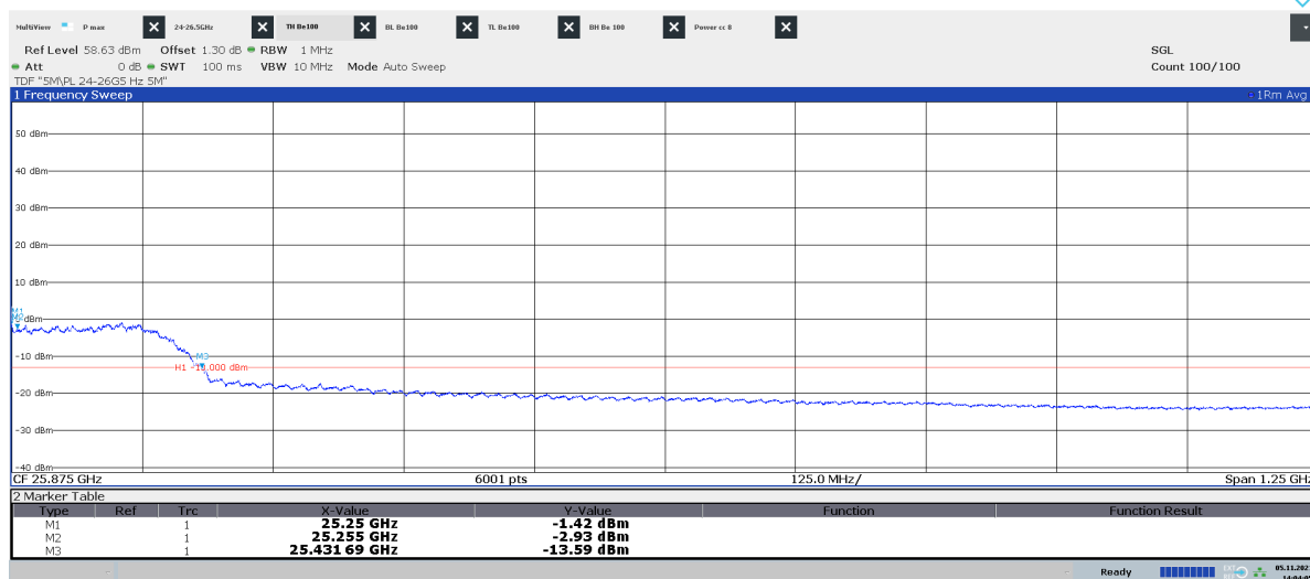
Diagram 2.20e: 25.25 – 26.5 GHz, QPSK, BT8 50 , EIRP Horizontal polarization
