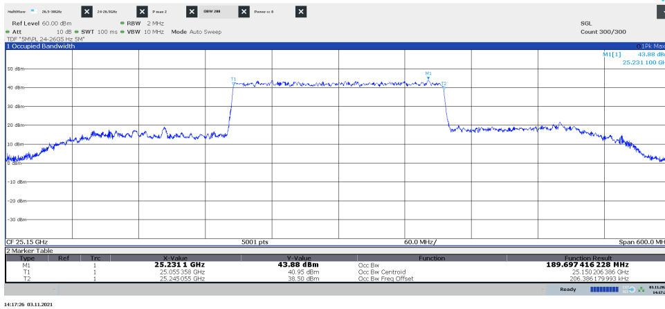
Diagram 1.6, Symbolic name: TH 200 , QPSK, Vertical:
