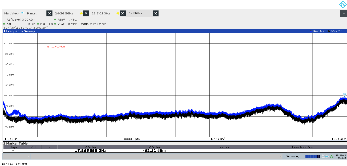
Diagram 2.18b: 1 – 18 GHz, QPSK, BT8 50 , EIRP Vertical polarization
