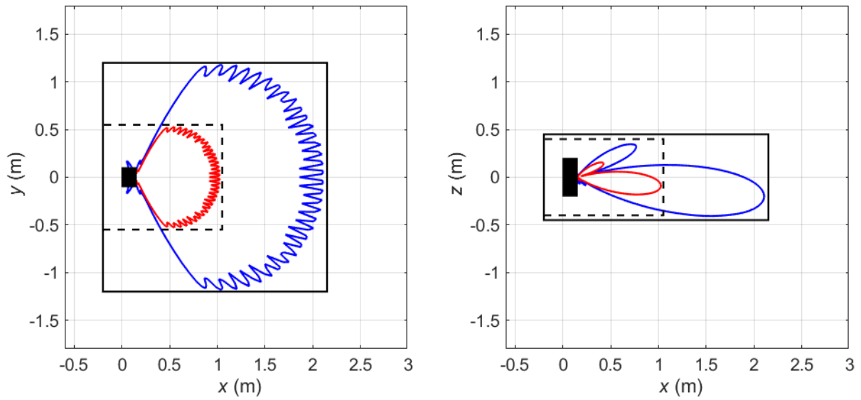
Figure 5 Compliance boundaries for general public (black solid line) and occupational (black dashed line) exposure for the USA and markets where the FCC exposure limits apply for Macro4 sector shape (Config Mode 0). The blue solid lines correspond to compliance distance results for general public exposure obtained using the spherical model. The solid red lines indicate the corresponding compliance distance results for occupational exposure. The EUT is shown from above (left) and from the side (right) with its backplane located at x = 0 m. Mode: B261 (28 GHz) (NR). Total EIRP of the Streetmacro: 57.2 dBm.
