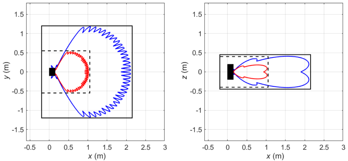
Figure 3 Compliance boundaries for general public (black solid line) and occupational (black dashed line) exposure for the USA and markets where the FCC exposure limits apply for Hotspot5 sector shape (Config Mode 0). The blue solid lines correspond to compliance distance results for general public exposure obtained using the spherical model. The solid red lines indicate the corresponding compliance distance results for occupational exposure. The EUT is shown from above (left) and from the side (right) with its backplane located at x = 0 m. Mode: B261 (28 GHz) (NR). Total EIRP of the Streetmacro: 57.2 dBm.
