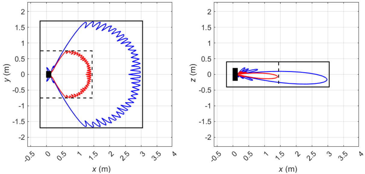
Figure 8 Compliance boundaries for general public (black solid line) and occupational (black dashed line) exposure for the USA and markets where the FCC exposure limits apply for Macro9 sector shape (Config Mode 1). The blue solid lines correspond to compliance distance results for general public exposure obtained using the spherical model. The solid red lines indicate the corresponding compliance distance results for occupational exposure. The EUT is shown from above (left) and from the side (right) with its backplane located at x = 0 m. Mode: B261 (28 GHz) (NR). Total EIRP of the Streetmacro: 60.2 dBm.
