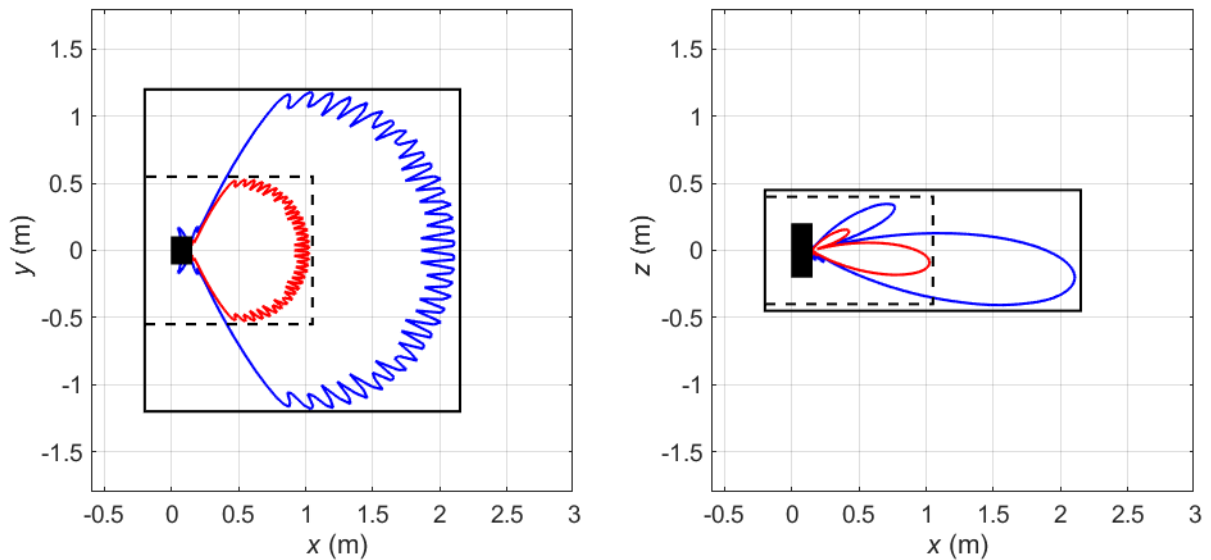
Figure 4 Compliance boundaries for general public (black solid line) and occupational (black dashed line) exposure for the USA and markets where the FCC exposure limits apply for Macro3 sector shape (Config Mode 0). The blue solid lines correspond to compliance distance results for general public exposure obtained using the spherical model. The solid red lines indicate the corresponding compliance distance results for occupational exposure. The EUT is shown from above (left) and from the side (right) with its backplane located at x = 0 m. Mode: B261 (28 GHz) (NR). Total EIRP of the Streetmacro: 57.2 dBm.
