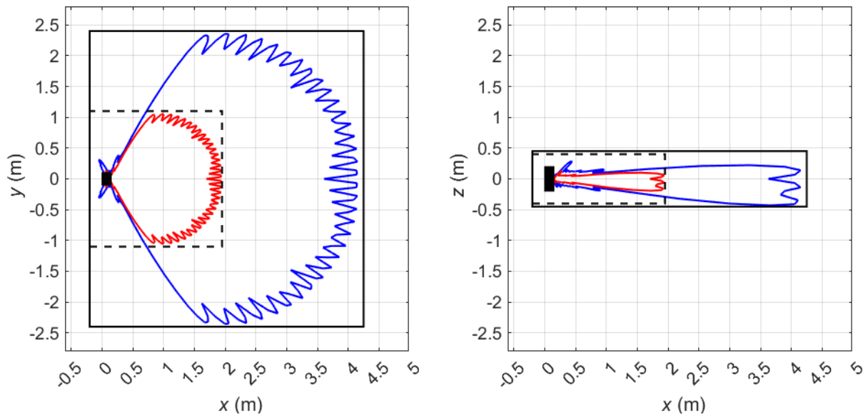
Figure 14 Compliance boundaries for general public (black solid line) and occupational (black dashed line) exposure for the USA and markets where the FCC exposure limits apply for Macro13 sector shape (Config Mode 2). The blue solid lines correspond to compliance distance results for general public exposure obtained using the spherical model. The solid red lines indicate the corresponding compliance distance results for occupational exposure. The EUT is shown from above (left) and from the side (right) with its backplane located at x = 0 m. Mode: B261 (28 GHz) (NR). Total EIRP of the Streetmacro: 63.2 dBm.
