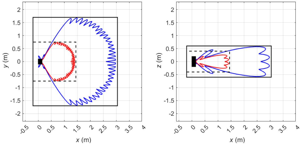
Figure 6 Compliance boundaries for general public (black solid line) and occupational (black dashed line) exposure for the USA and markets where the FCC exposure limits apply for Hotspot2 sector shape (Config Mode 1). The blue solid lines correspond to compliance distance results for general public exposure obtained using the spherical model. The solid red lines indicate the corresponding compliance distance results for occupational exposure. The EUT is shown from above (left) and from the side (right) with its backplane located at x = 0 m. Mode: B261 (28 GHz) (NR). Total EIRP of the Streetmacro: 60.2 dBm.
