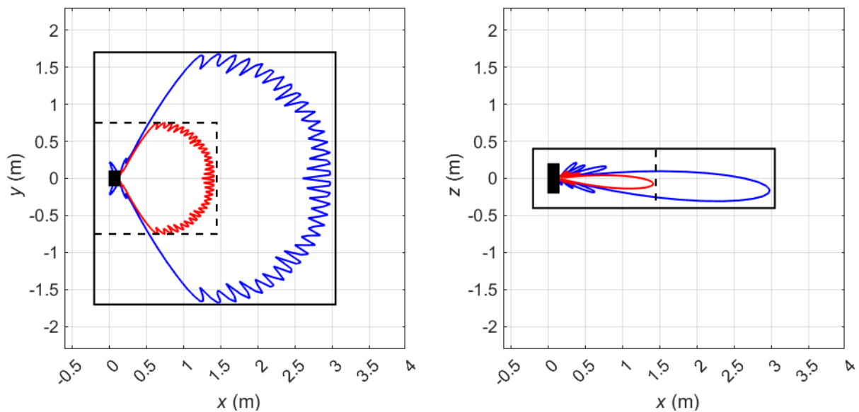
Figure 10 Compliance boundaries for general public (black solid line) and occupational (black dashed line) exposure for the USA and markets where the FCC exposure limits apply for Macro11 sector shape (Config Mode 2). The blue solid lines correspond to compliance distance results for general public exposure obtained using the spherical model. The solid red lines indicate the corresponding compliance distance results for occupational exposure. The EUT is shown from above (left) and from the side (right) with its backplane located at x = 0 m. Mode: B261 (28 GHz) (NR). Total EIRP of the Streetmacro: 60.2 dBm.
