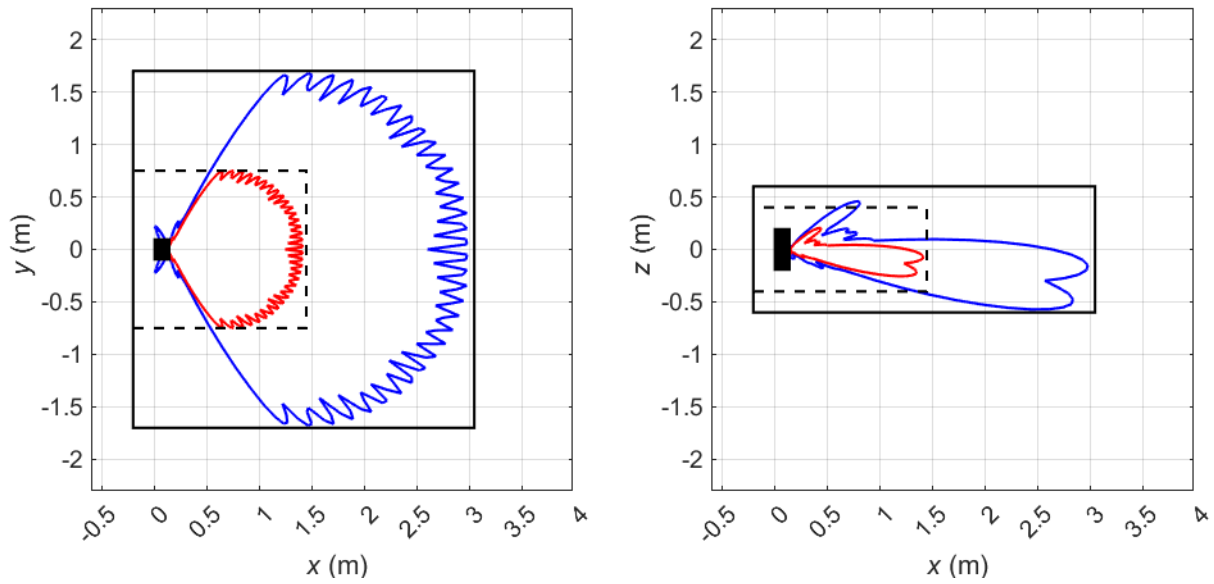
Figure 9 Compliance boundaries for general public (black solid line) and occupational (black dashed line) exposure for the USA and markets where the FCC exposure limits apply for Macro10 sector shape (Config Mode 1). The blue solid lines correspond to compliance distance results for general public exposure obtained using the spherical model. The solid red lines indicate the corresponding compliance distance results for occupational exposure. The EUT is shown from above (left) and from the side (right) with its backplane located at x = 0 m. Mode: B261 (28 GHz) (NR). Total EIRP of the Streetmacro: 60.2 dBm.
