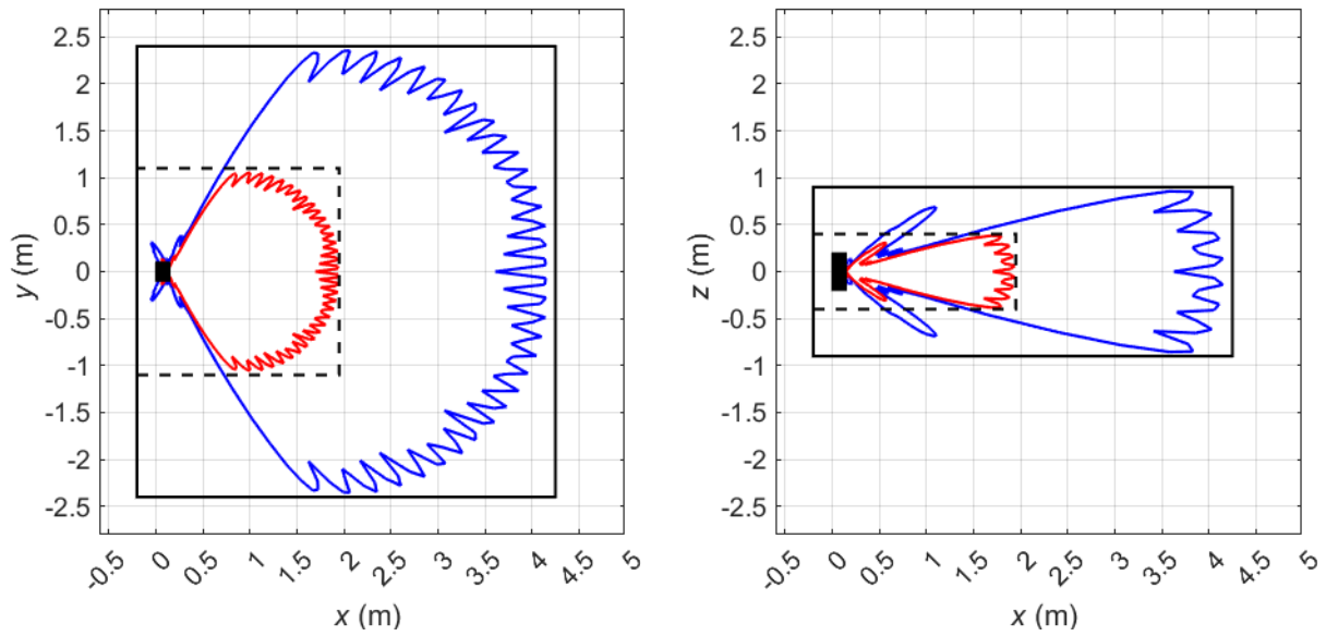
Figure 11 Compliance boundaries for general public (black solid line) and occupational (black dashed line) exposure for the USA and markets where the FCC exposure limits apply for Hotspot2 sector shape (Config Mode 2). The blue solid lines correspond to compliance distance results for general public exposure obtained using the spherical model. The solid red lines indicate the corresponding compliance distance results for occupational exposure. The EUT is shown from above (left) and from the side (right) with its backplane located at x = 0 m. Mode: B261 (28 GHz) (NR). Total EIRP of the Streetmacro: 63.2 dBm.
