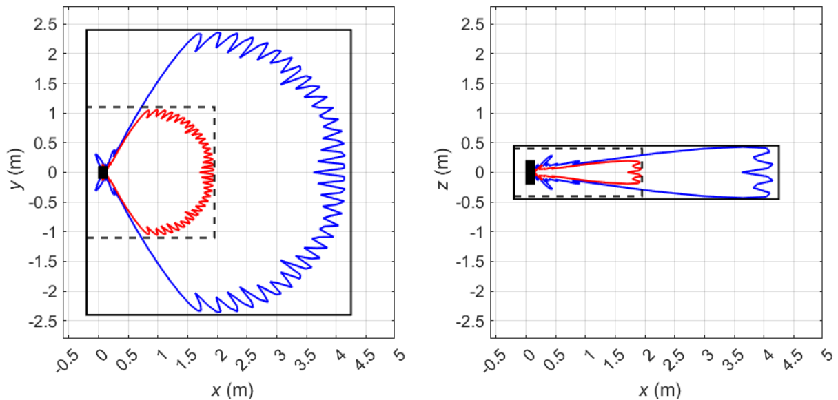
Figure 12 Compliance boundaries for general public (black solid line) and occupational (black dashed line) exposure for the USA and markets where the FCC exposure limits apply for Macro5 sector shape (Config Mode 2). The blue solid lines correspond to compliance distance results for general public exposure obtained using the spherical model. The solid red lines indicate the corresponding compliance distance results for occupational exposure. The EUT is shown from above (left) and from the side (right) with its backplane located at x = 0 m. Mode: B261 (28 GHz) (NR). Total EIRP of the Streetmacro: 63.2 dBm.
