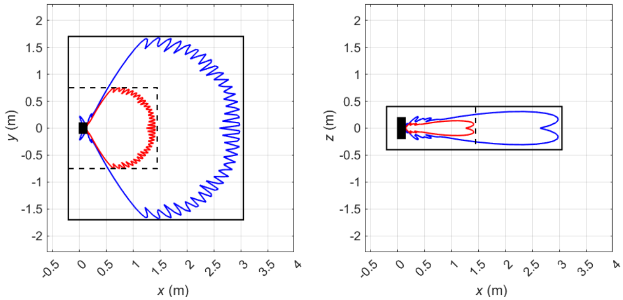
Figure 7 Compliance boundaries for general public (black solid line) and occupational (black dashed line) exposure for the USA and markets where the FCC exposure limits apply for Macro3 sector shape (Config Mode 1). The blue solid lines correspond to compliance distance results for general public exposure obtained using the spherical model. The solid red lines indicate the corresponding compliance distance results for occupational exposure. The EUT is shown from above (left) and from the side (right) with its backplane located at x = 0 m. Mode: B261 (28 GHz) (NR). Total EIRP of the Streetmacro: 60.2 dBm.
