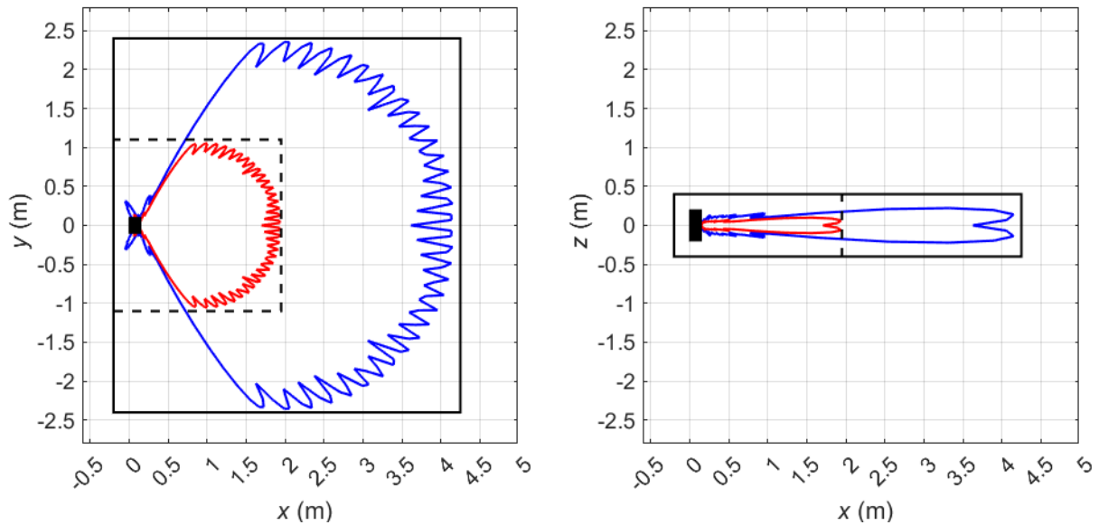
Figure 13 Compliance boundaries for general public (black solid line) and occupational (black dashed line) exposure for the USA and markets where the FCC exposure limits apply for Macro7 sector shape (Config Mode 2). The blue solid lines correspond to compliance distance results for general public exposure obtained using the spherical model. The solid red lines indicate the corresponding compliance distance results for occupational exposure. The EUT is shown from above (left) and from the side (right) with its backplane located at x = 0 m. Mode: B261 (28 GHz) (NR). Total EIRP of the Streetmacro: 63.2 dBm.
