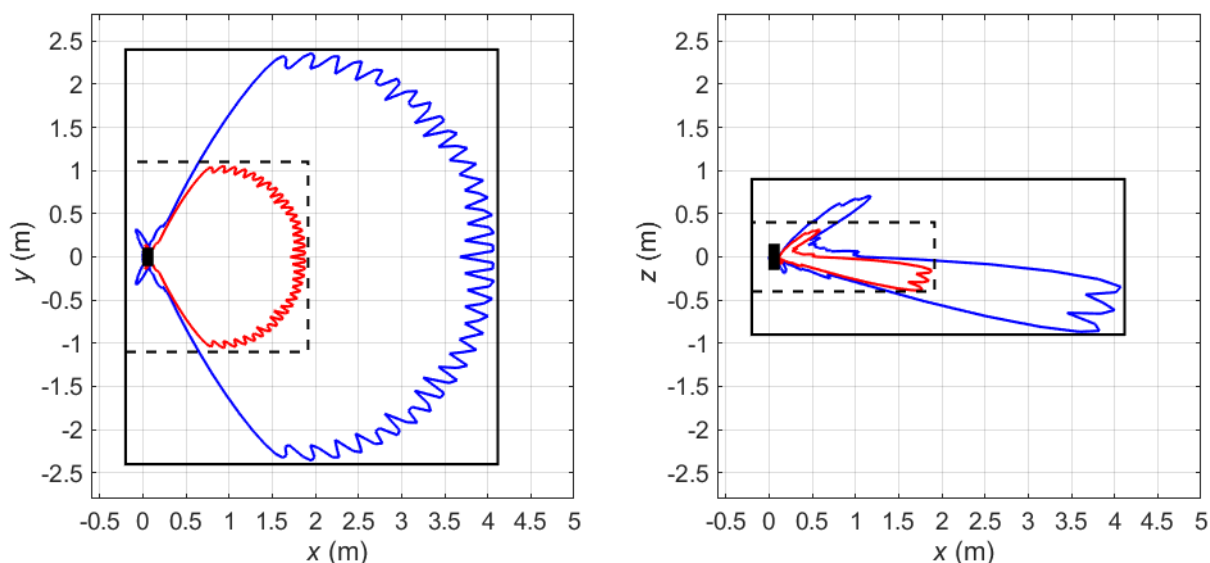
Figure 20 Compliance boundaries for general public (black solid line) and workers (black dashed line) exposure for markets where the FCC exposure limits apply for Macro13 (tilt 11.25^\circ ) sector shape (Configuration Mode 2). The blue solid lines correspond to compliance distance results for general public exposure obtained using the spherical models. The solid red lines indicate the corresponding compliance distance results for workers exposure. The EUT is shown from above (left) and from the side (right) with its backplane located at x = 0 m. Mode: B258 (26 GHz) (NR). Total EIRP of the radio: 63.2 dBm.
