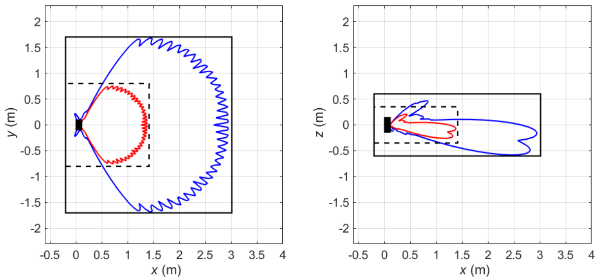
Figure 8 Compliance boundaries for general public (black solid line) and workers (black dashed line) exposure for markets where the FCC exposure limits apply for Macro3 (tilt 7.5^\circ ) sector shape (Configuration Mode 1). The blue solid lines correspond to compliance distance results for general public exposure obtained using the spherical models. The solid red lines indicate the corresponding compliance distance results for workers exposure. The EUT is shown from above (left) and from the side (right) with its backplane located at x = 0 m. Mode: B258 (26 GHz) (NR). Total EIRP of the radio: 60.2 dBm.
