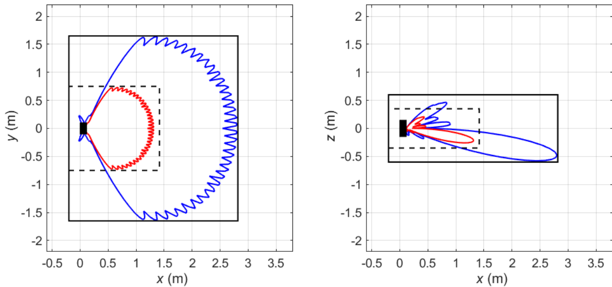
Figure 10 Compliance boundaries for general public (black solid line) and workers (black dashed line) exposure for markets where the FCC exposure limits apply for Macro9 (tilt 7.5^\circ ) sector shape (Configuration Mode 1). The blue solid lines correspond to compliance distance results for general public exposure obtained using the spherical models. The solid red lines indicate the corresponding compliance distance results for workers exposure. The EUT is shown from above (left) and from the side (right) with its backplane located at x = 0 m. Mode: B258 (26 GHz) (NR). Total EIRP of the radio: 60.2 dBm.
