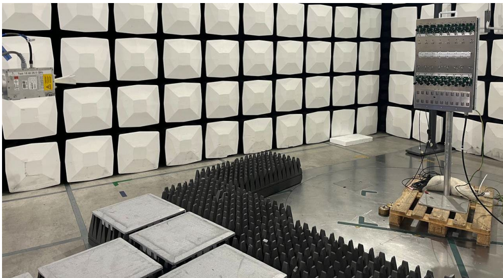
Photo of the test set-up for radiated emission above 1 GHz
