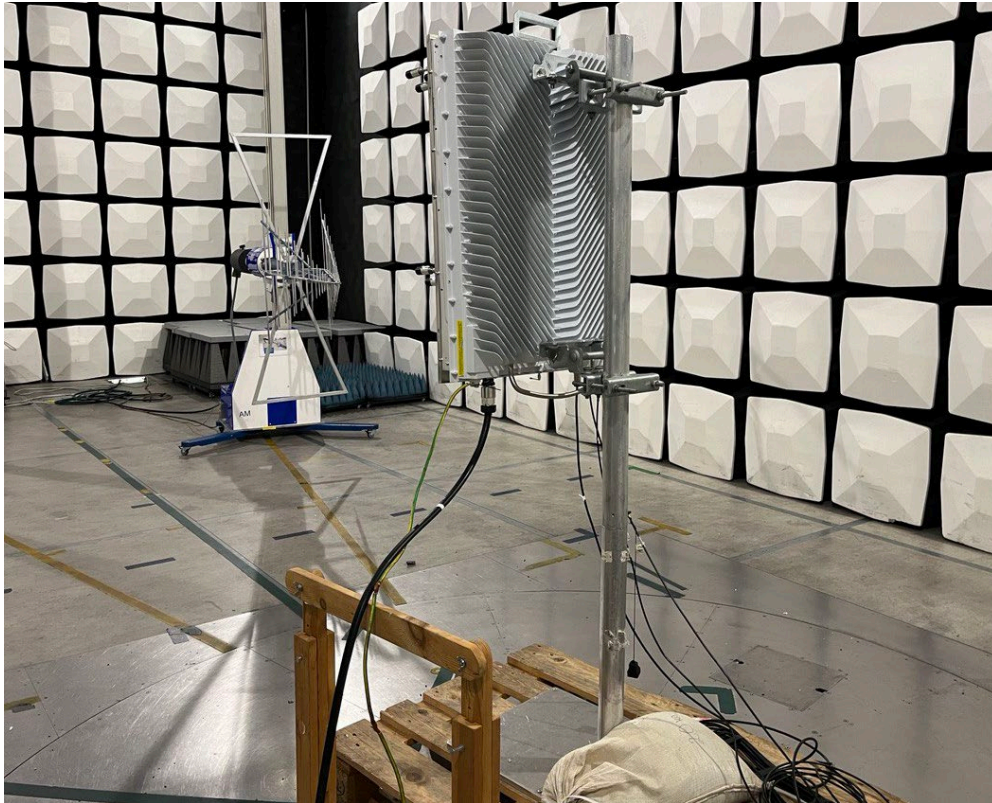
Photo of the test set-up for radiated emission 30 – 1000 MHz
