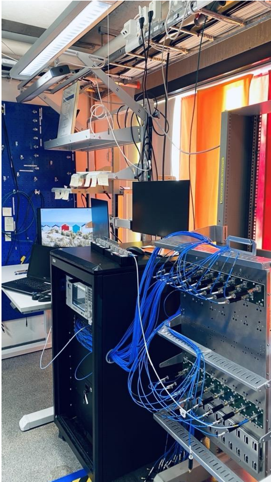
Conducted Lab Testing- Conducted - HP-VEE Software
