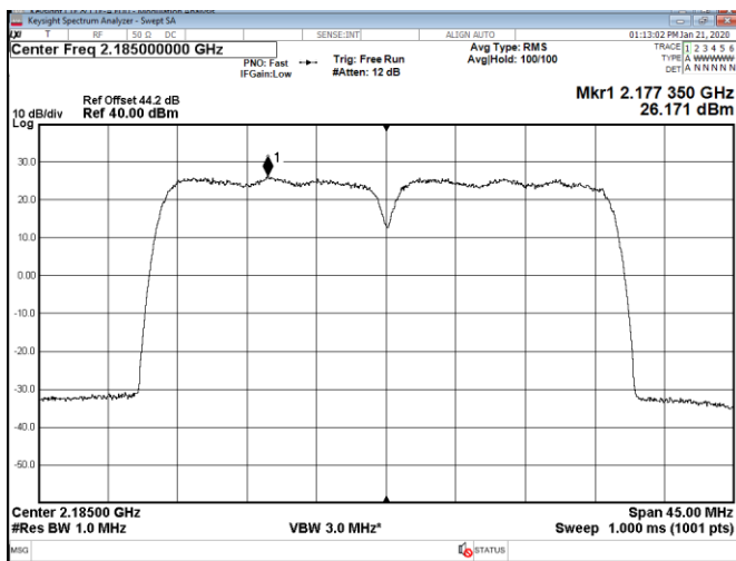
Figure 8.1-9: PSD of 15 MHz channel bandwidth, two-carrier operation, sample plot
