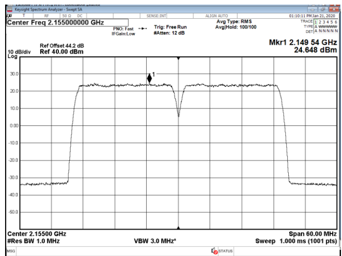
Figure 8.1-10: PSD of 20 MHz channel bandwidth, two-carrier operation, sample plot
