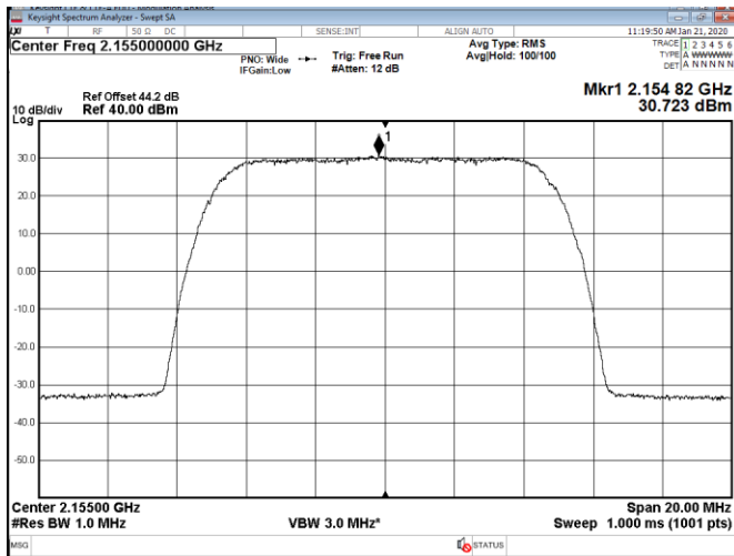
Figure 8.1-5: PSD of 10 MHz channel bandwidth, single carrier operation, sample plot
