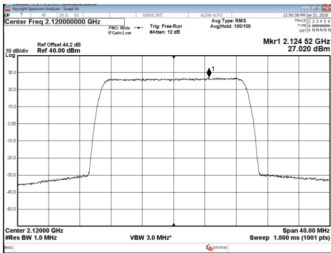
Figure 8.1-7: PSD of 20 MHz channel bandwidth, single carrier operation, sample plot
