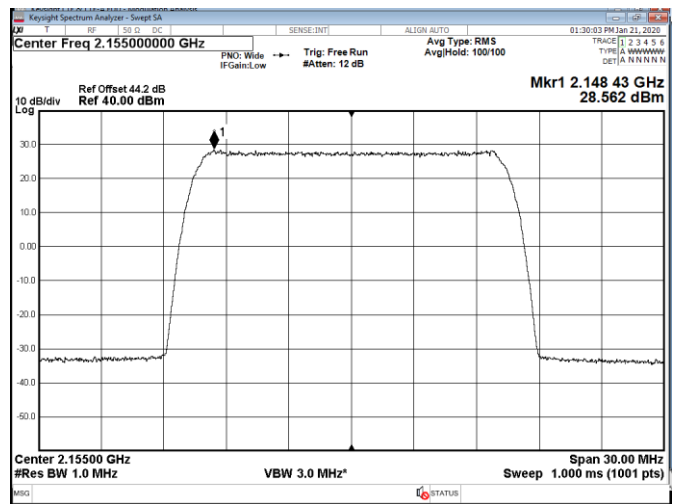
Figure 8.1-12: PSD of 15 MHz channel bandwidth, LTE and IoT operation, sample plot
