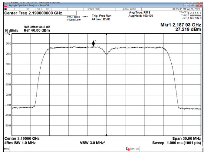
Figure 8.1-8: PSD of 10 MHz channel bandwidth, two-carrier operation, sample plot
