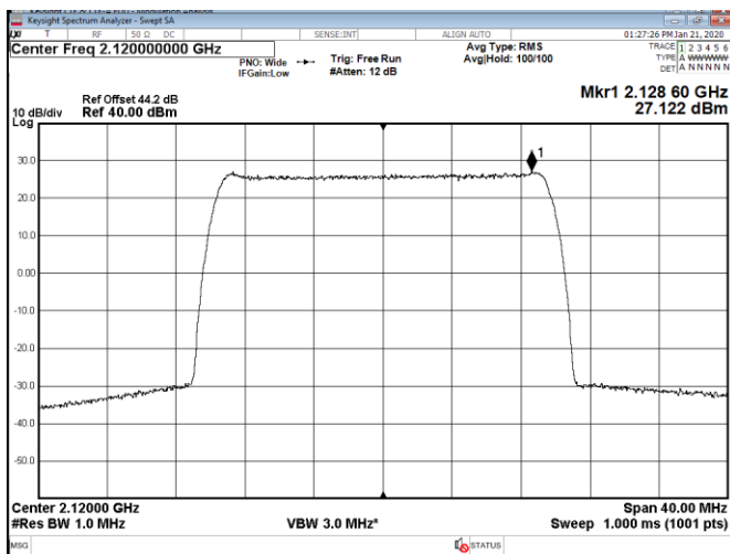
Figure 8.1-13: PSD of 20 MHz channel bandwidth, LTE and IoT operation, sample plot
