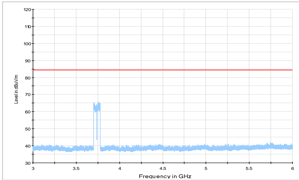
Configuration NR-MIMO-2C; 256QAM; 40MHz, Vertical, 3GHz-6GHz
