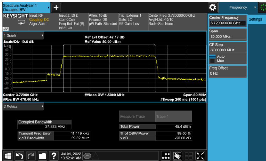
Port 10, 256QAM 40.0M Channel position M
