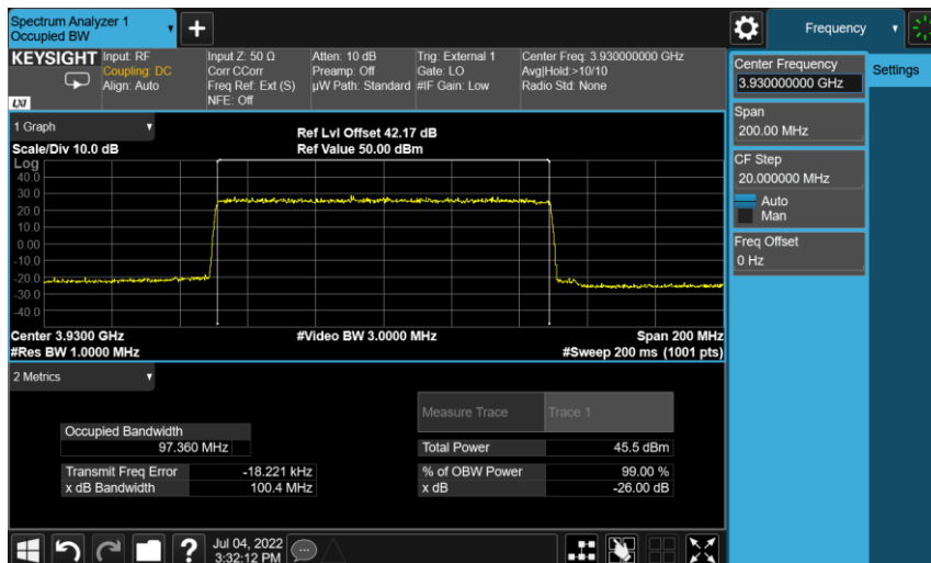
Port 10, 256QAM 100.0M Channel position T
