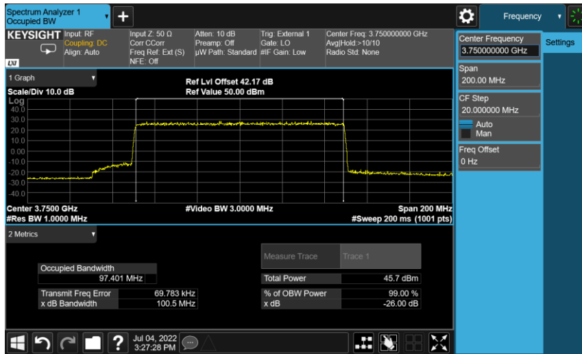
Port 10, 256QAM 100.0M Channel position M
