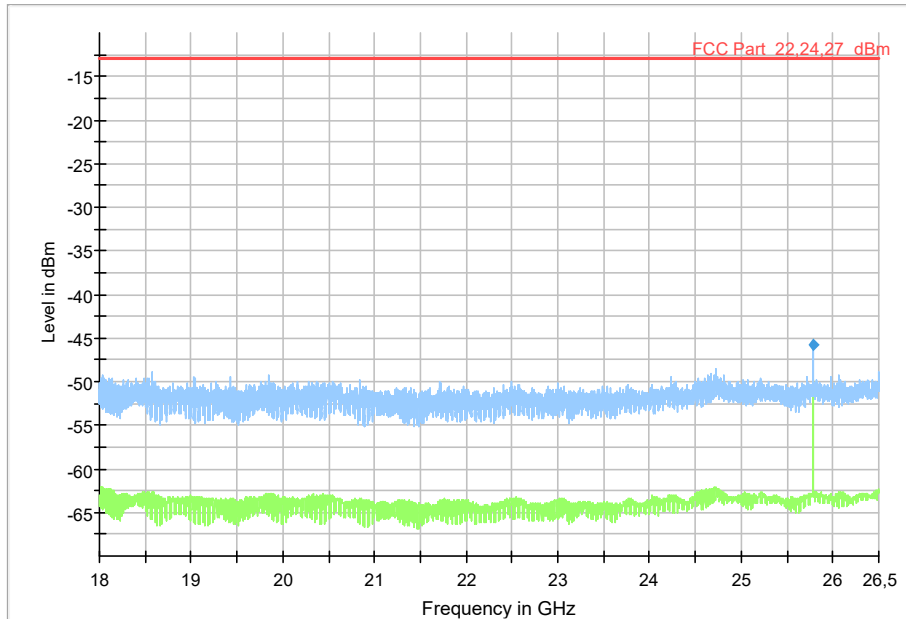
Diagram, Peak and average overview sweep, 18 – 26.5 GHz at 3 m distance. Channel 2 Measurement results, RMS
