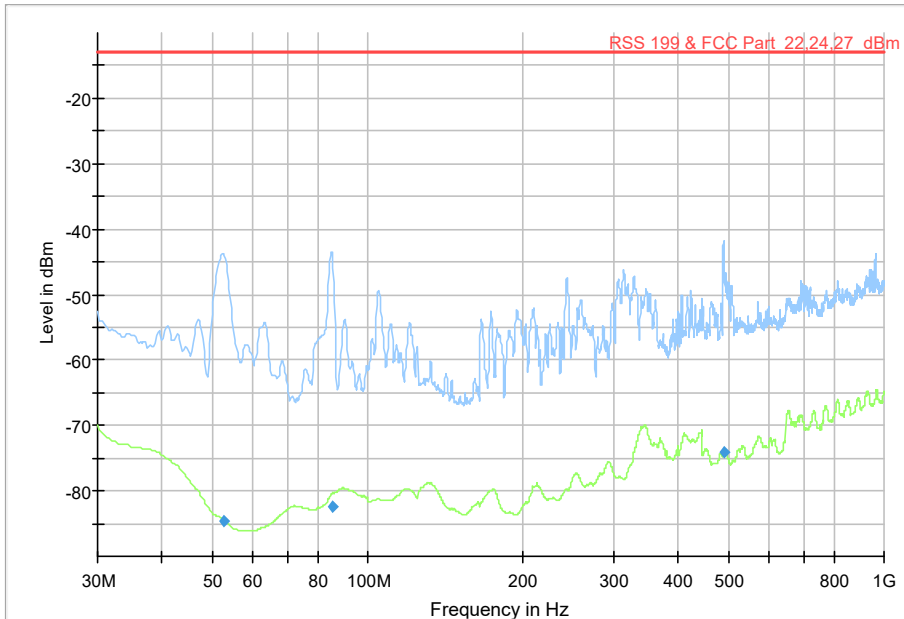
Diagram, Peak and average overview sweep, 30 – 1000 MHz at 3 m distance. Channel 2
