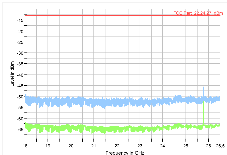
Diagram, Peak and average overview sweep, 18 – 26.5 GHz at 3 m distance. Channel 3 Measurement results, RMS
