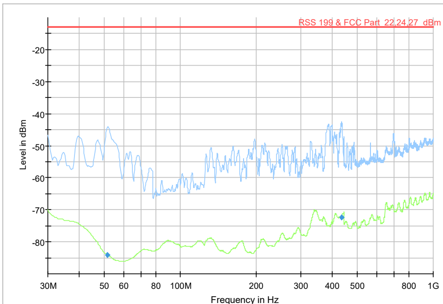
Diagram, Peak and average overview sweep, 30 – 1000 MHz at 3 m distance. Channel 3
