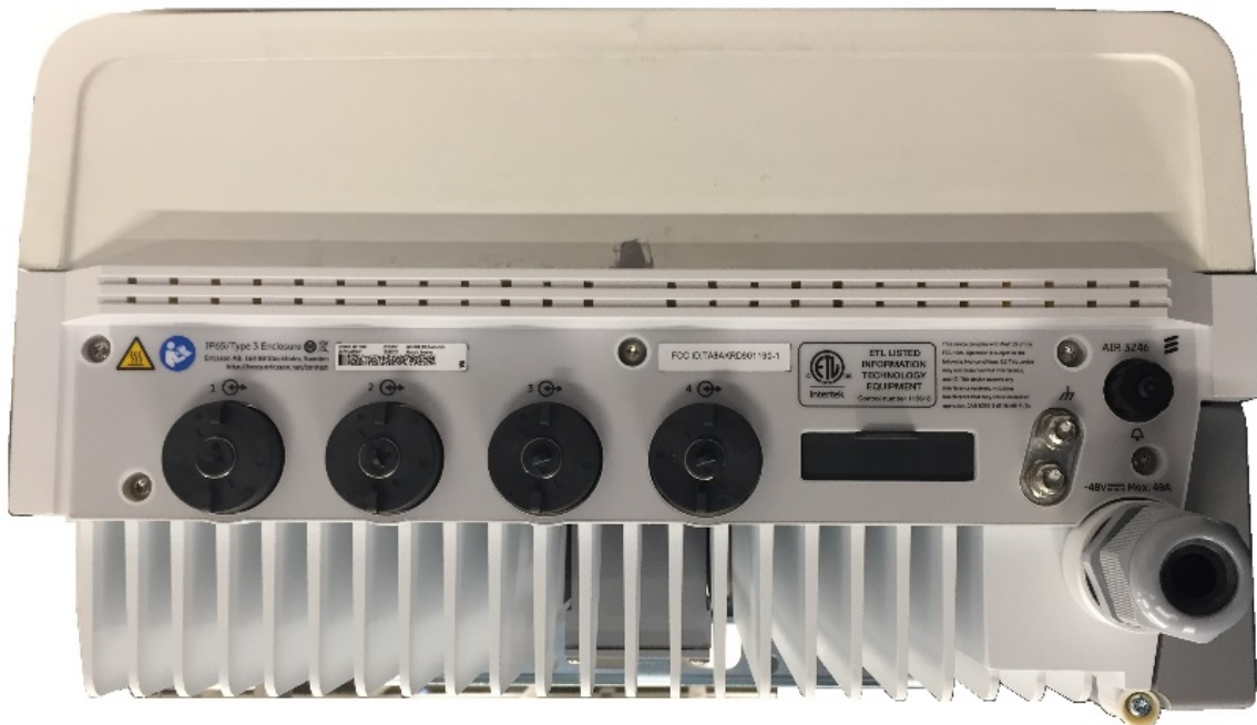
Figure 2: AIR 3246 B66 Bottom / Connector View
