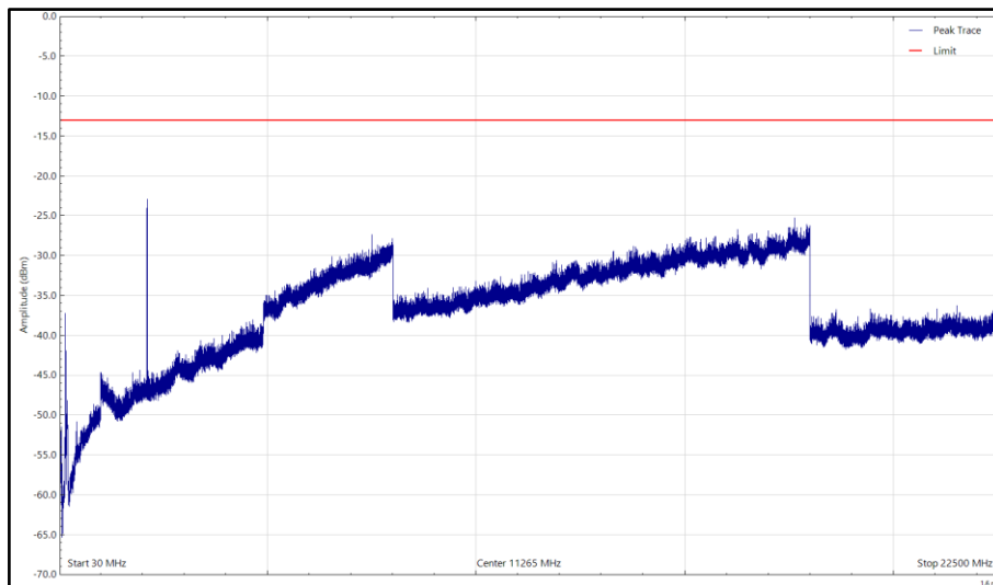
Bot - NR&NB-IoT - B66, 2115MHz, 30 MHz to 22.5 GHz, Vertical (Peak)
