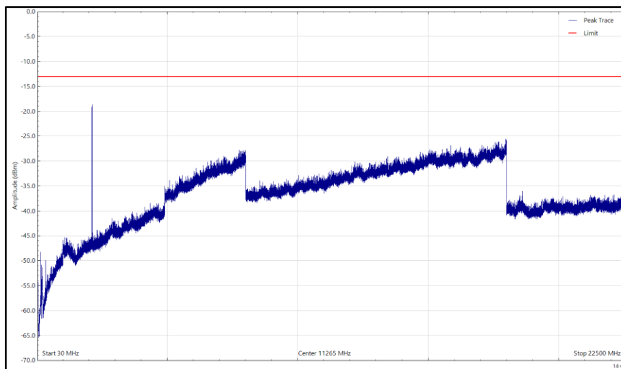
Bot - NR&NB-IoT - B66, 2115MHz, 30 MHz to 22.5 GHz, Horizontal (Peak)
