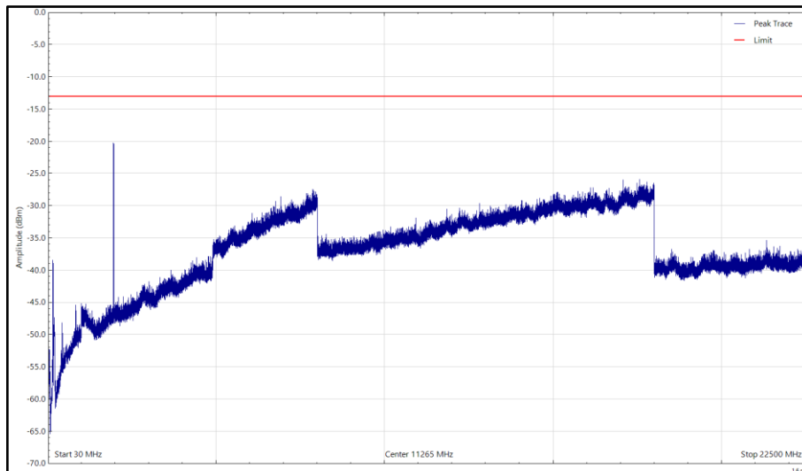
Mid - NR&NB-IoT - B25, 1962.5MHz, 30 MHz to 22.5 GHz, Vertical (Peak)
