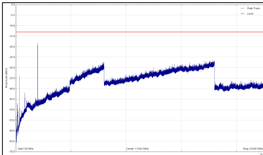
Top - NR&NB-IoT - B2, 1985MHz, 30 MHz to 22.5 GHz, Horizontal (Peak)
