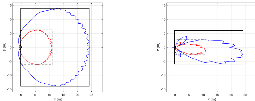
Figure 2 Compliance boundaries for general public (black solid line) and workers (black dashed line) exposure for the markets where the FCC exposure limits apply. The blue solid lines correspond to compliance distance results for general public exposure obtained using the spherical models. The solid red lines indicate the corresponding compliance distance results for workers exposure. The antenna is shown from above (left) and from the side (right) with its backplane located at x = 0 m. Mode: B41 (2500 MHz) (LTE). Total time-averaged power delivered to the antenna: 54.8 dBm.
