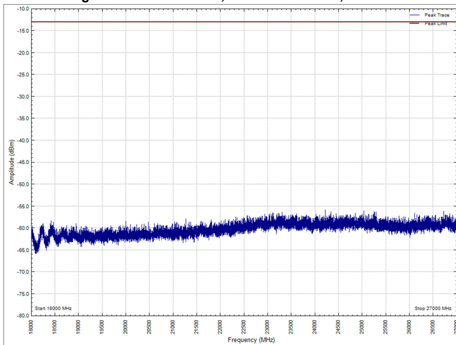
Figure 17 - 2593.02 MHz, 18 GHz to 27 GHz, Horizontal
