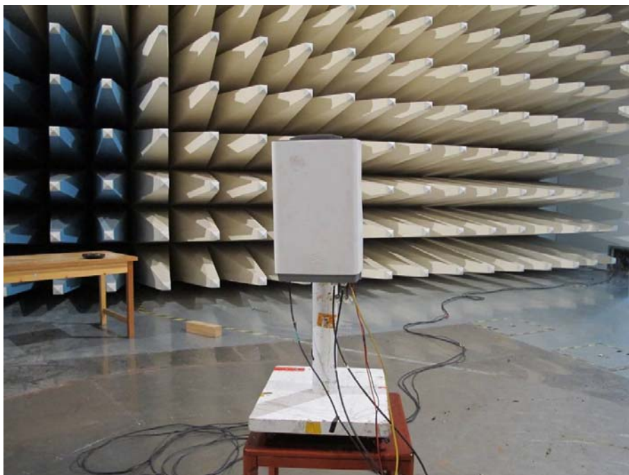
Internal antenna KRE 101 2141/1, upright mounted Maximum PEAK Output Power – Radiated (EIRP)
