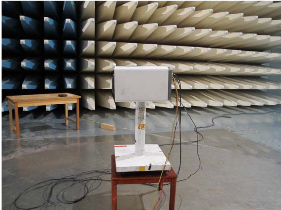
Internal antenna KRE 101 2141/1, side mounted Maximum PEAK Output Power – Radiated (EIRP)
