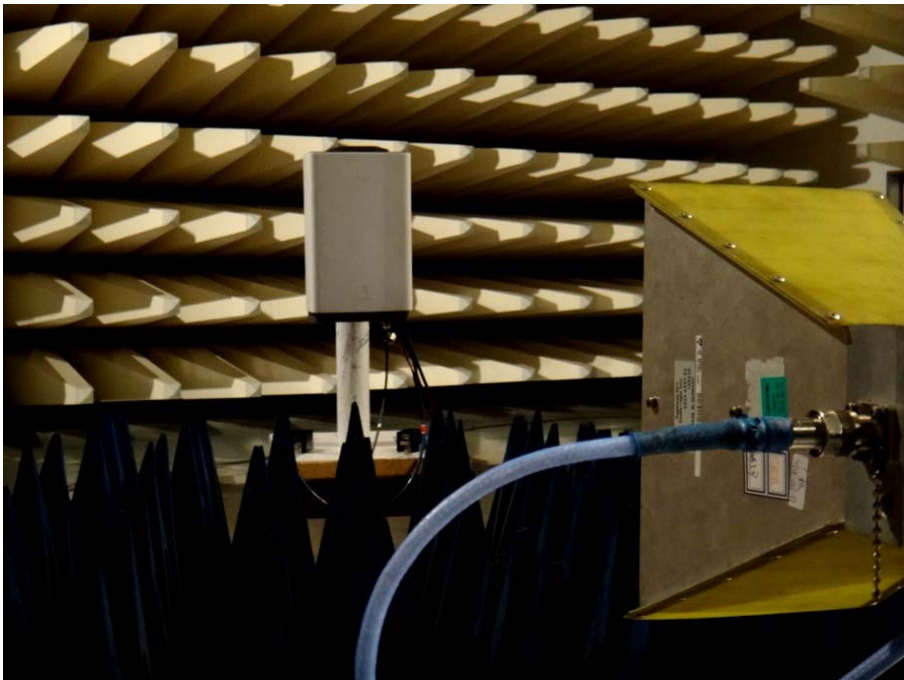
Radiated Emissions (3GHz – 10GHz)
