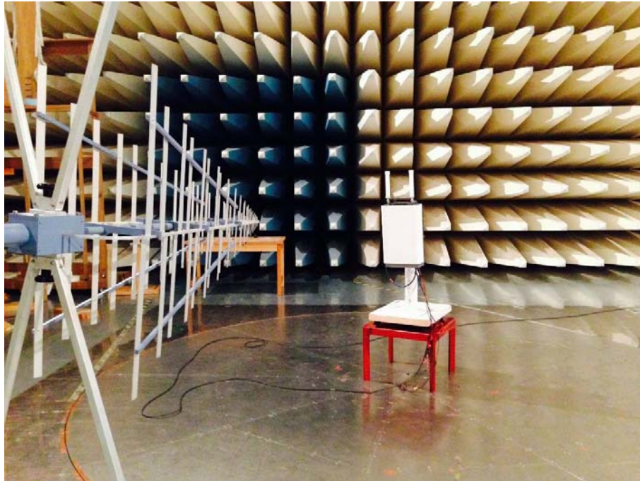
Semi-integrated Omni antenna KRE 101 2245/1, upright mounted
