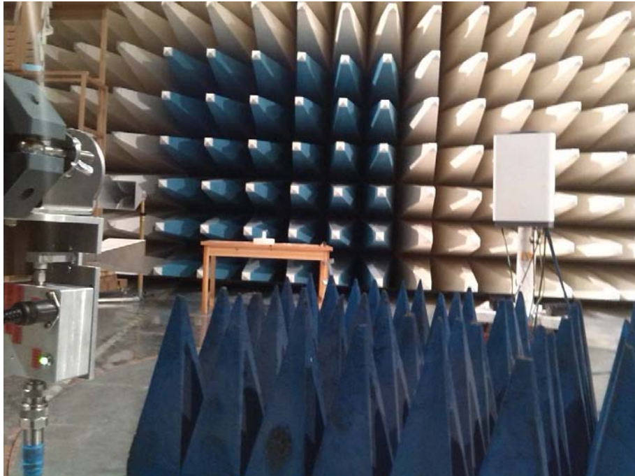
Radiated Emissions
