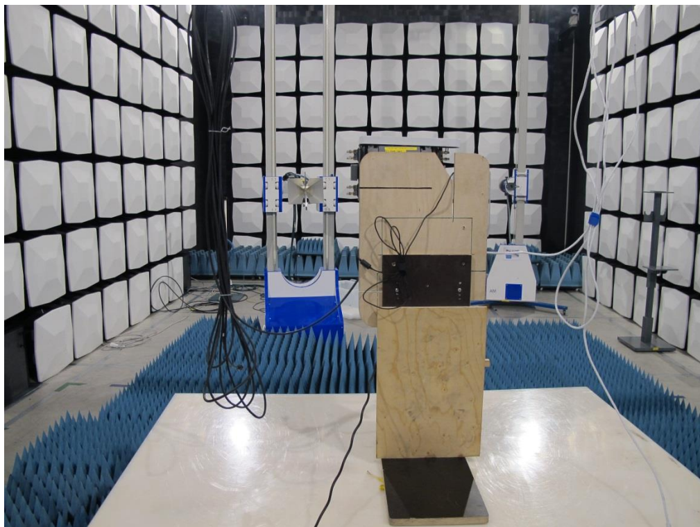
Test set up radiated emission 1GHz – 18 GHz. EUT in vertical position.
