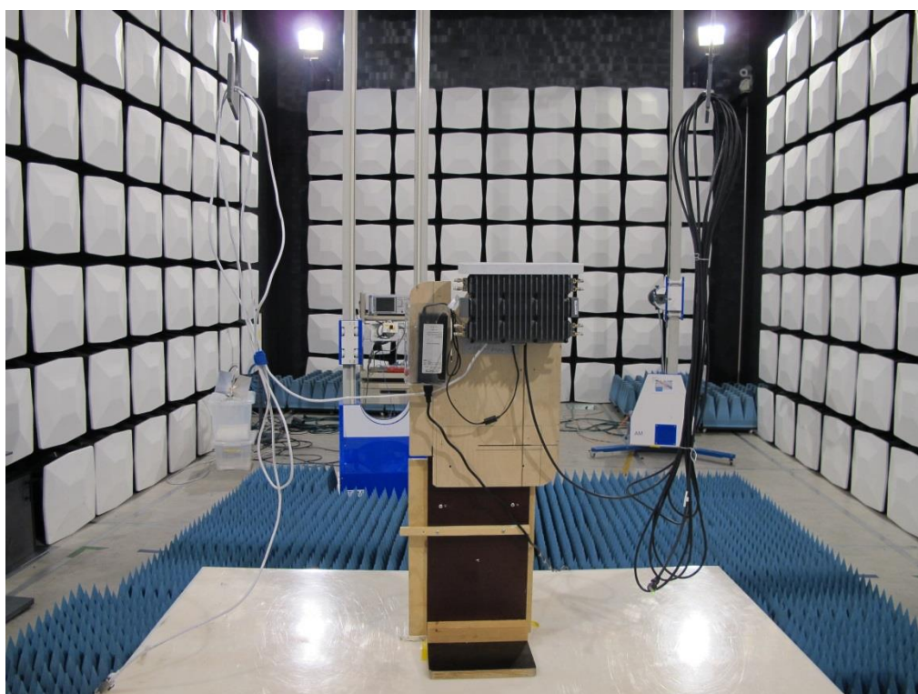
Test set up radiated emission 26 GHz – 40 GHz. EUT in vertical position.
