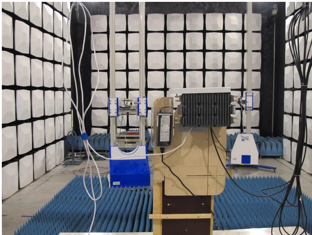
Test set up radiated emission 18 GHz – 26.5 GHz. EUT in vertical position.
