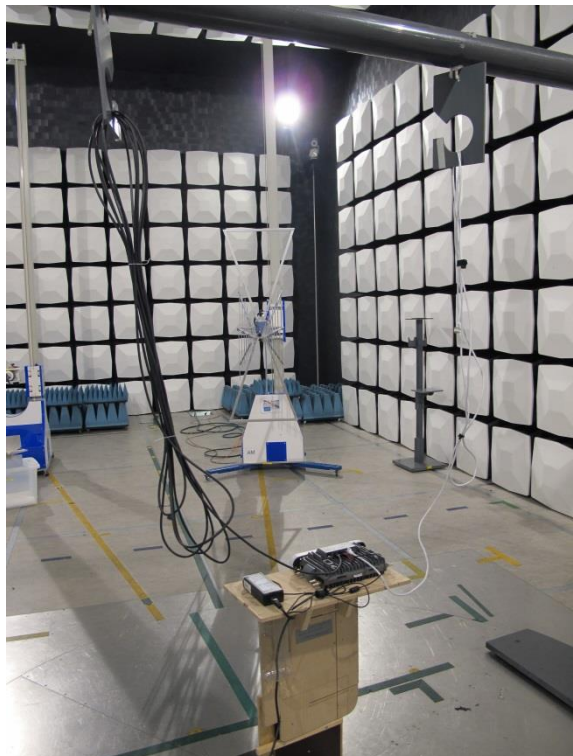
Test set up radiated emission 30 MHz – 1GHz. EUT in horizontal position.
