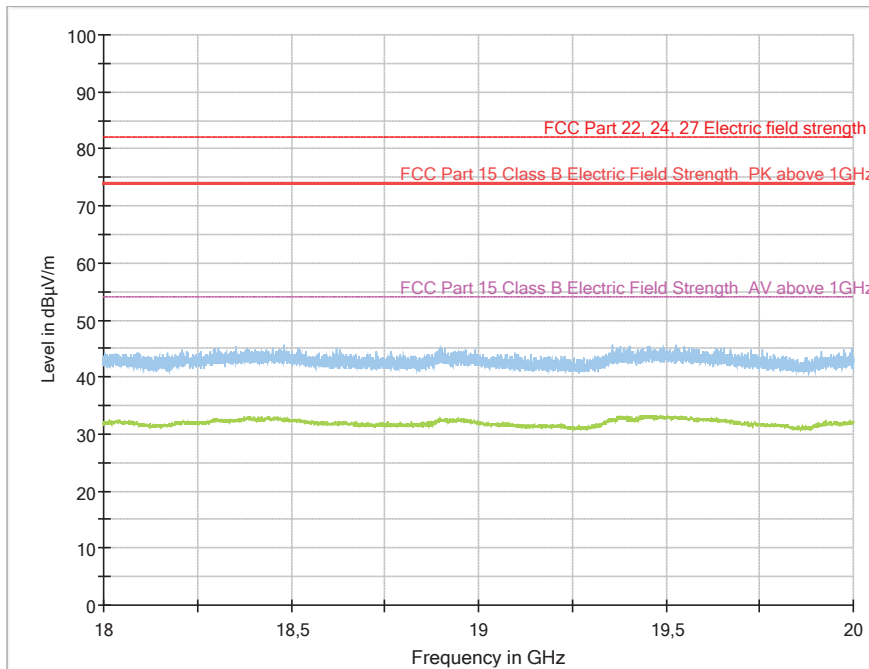
Diagram, Peak overview sweep, 18 – 20 GHz at 3 m distance, Middle channel, EUT in vertical position, powered by PoE injection
