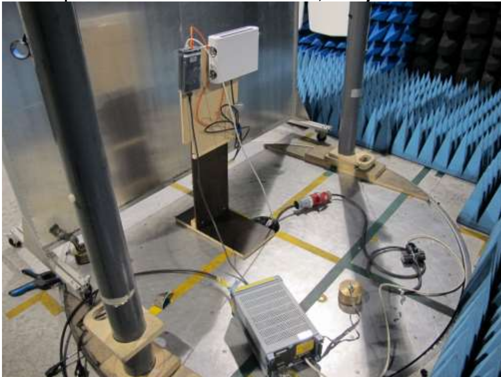
Test set up conducted emission 150 kHz – 30 MHz, PoE injector
