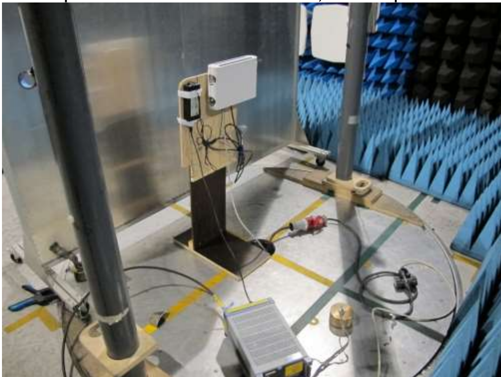
Test set up conducted emission 150 kHz – 30 MHz, AC/DC adapter
