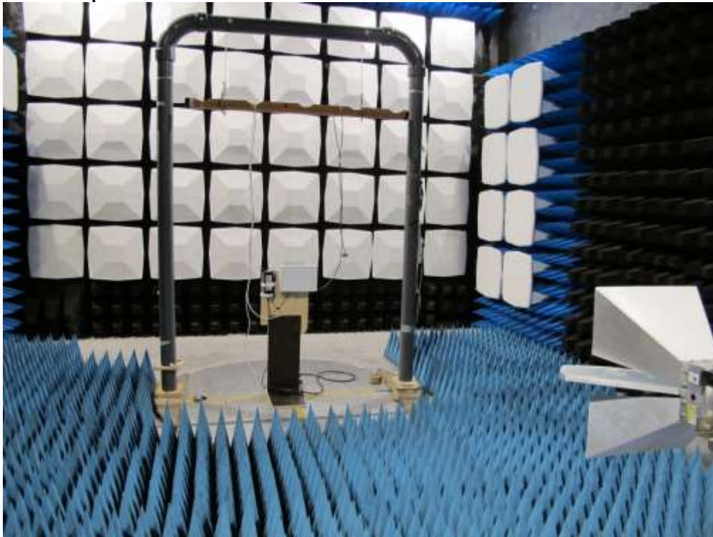
Test set up radiated emission 18 GHz – 26.5 GHz
