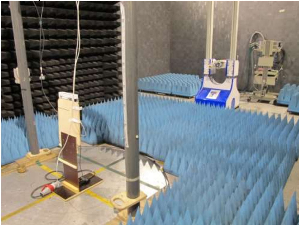
Test set up radiated emission 26.5 GHz – 40 GHz
