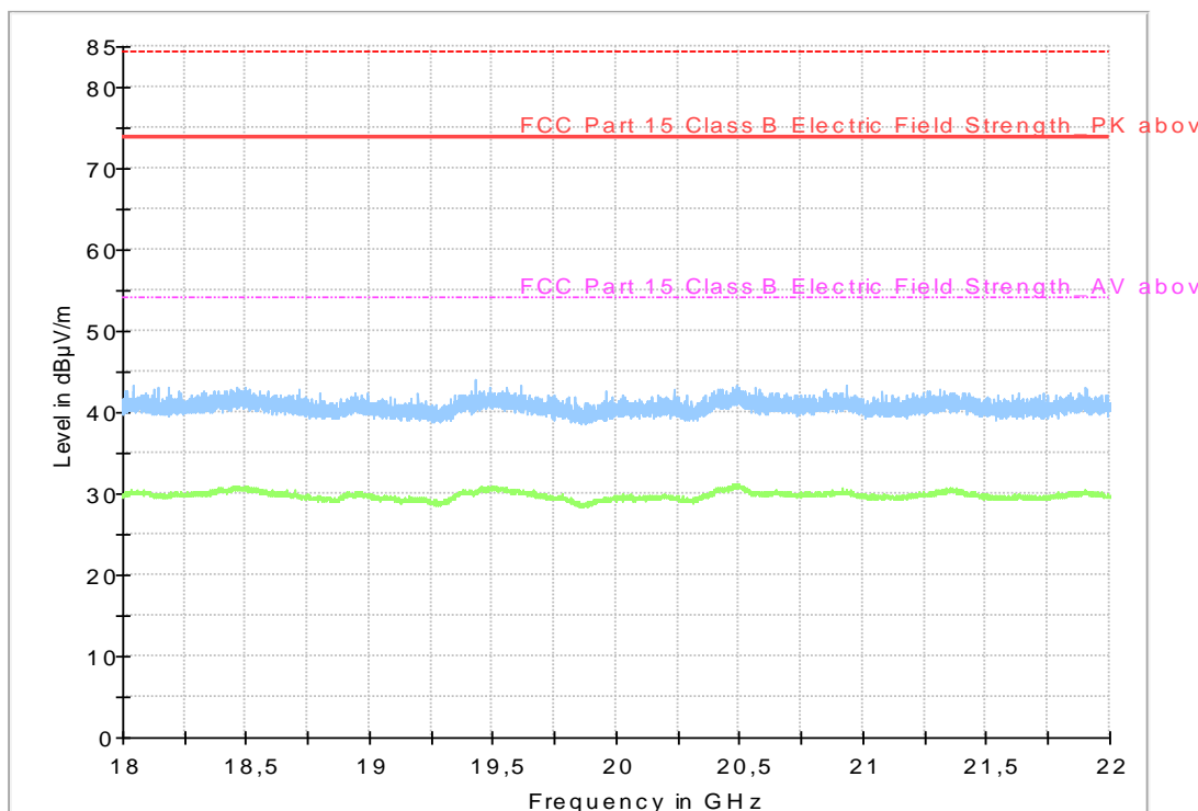
Diagram, Peak overview sweep, 18 – 22 GHz at 3 m distance. Middle channel. EUT in vertical position, powered by AC/DC adapter.
