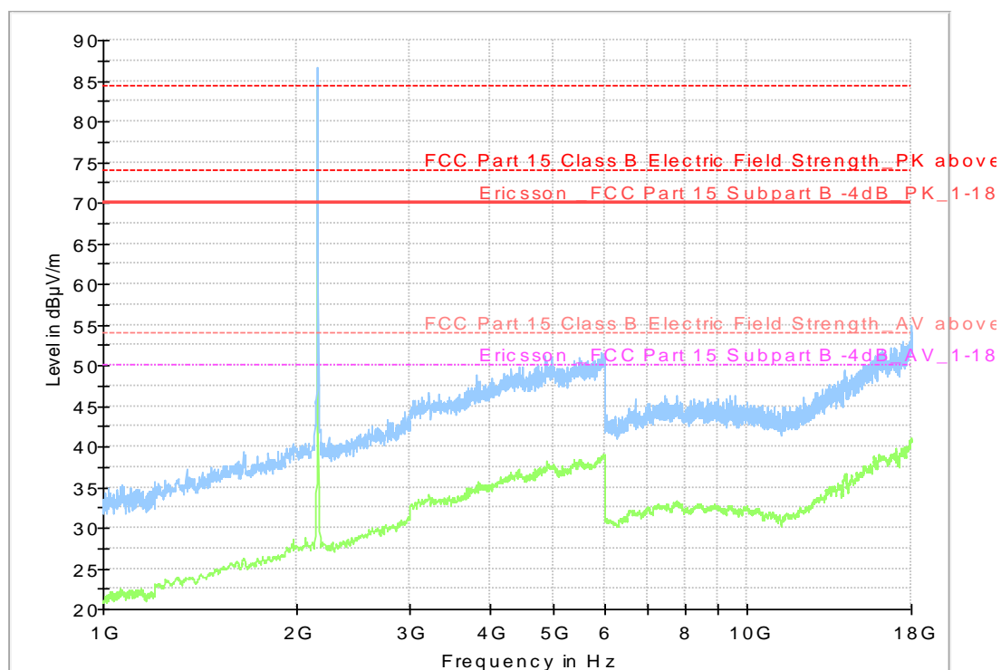
Diagram, Peak overview sweep, 1 – 18 GHz at 3 m distance. Top channel. EUT in vertical position, powered by AC/DC adapter.
