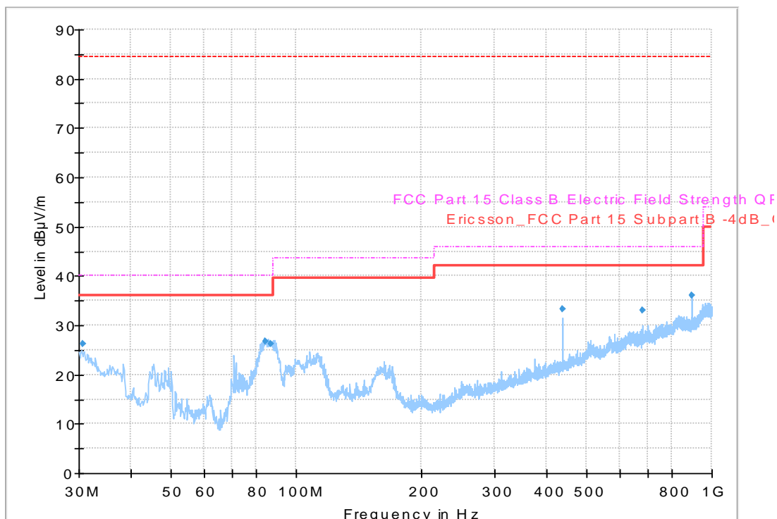
Diagram, Peak overview sweep, 30 – 1000 MHz at 3 m distance. Bottom and top channel. EUT in vertical position, powered by AC/DC adapter.
