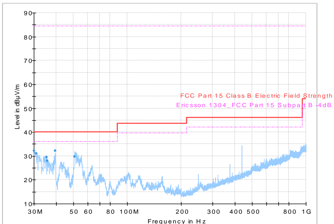
Diagram, Peak overview sweep, 30 – 1000 MHz at 3 m distance. Bottom and top channel. EUT in horizontal position, powered by PoE injector.
