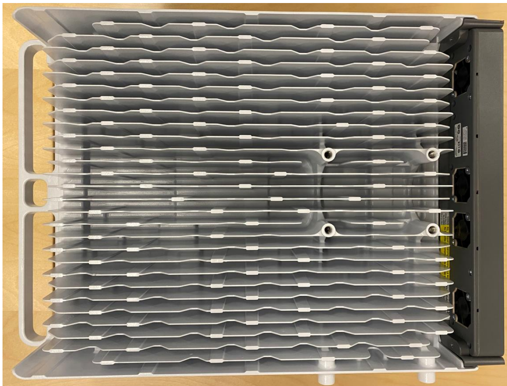
Figure 3: Radio 4480 44B66 44B70 C (with Optional Fan) Front / Back (Mounting) View
