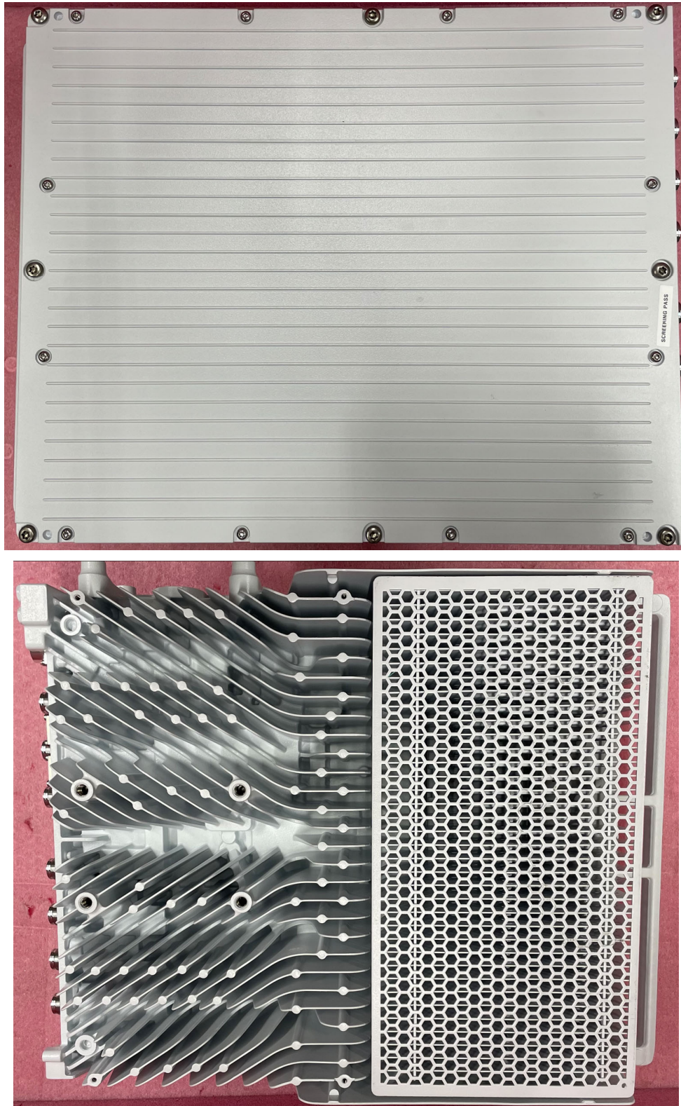
Figure 3: Radio 4890HP 48B2/B25 48B66 M01 Front / Back (Mounting) View
