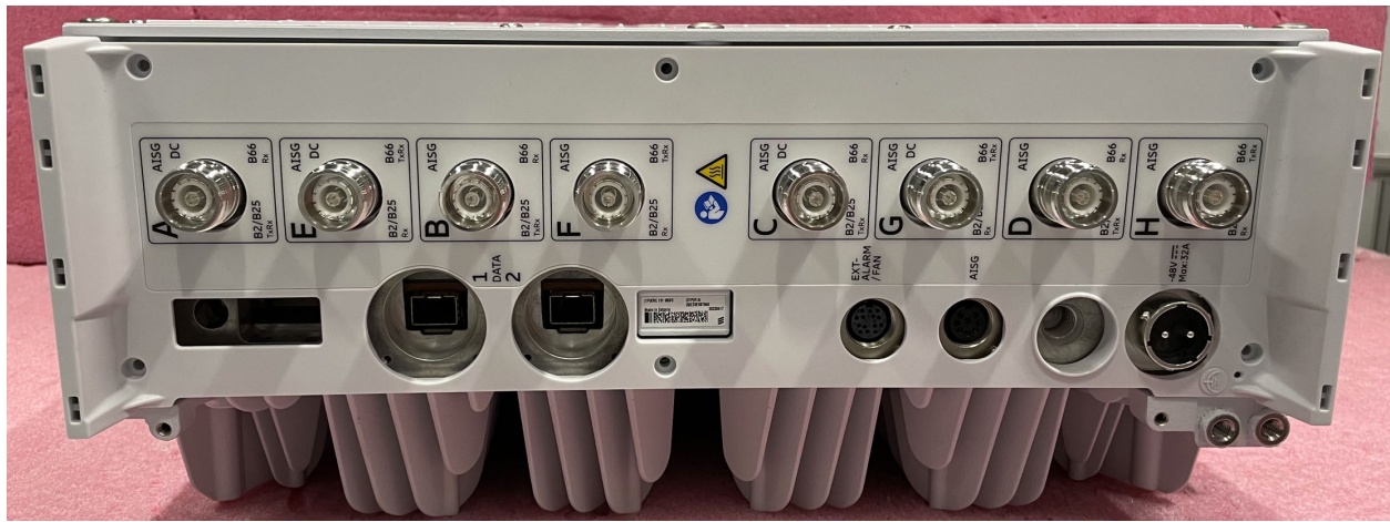
Figure 1: Radio 4890HP 48B2/B25 48B66 M01 Bottom / Connector View
