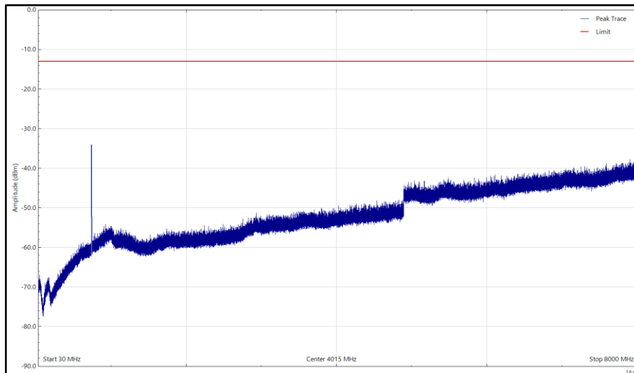
Mid - NR&NB-IoT - B85A, 736.5MHz, 30 MHz to 8 GHz, Horizontal (Peak)
