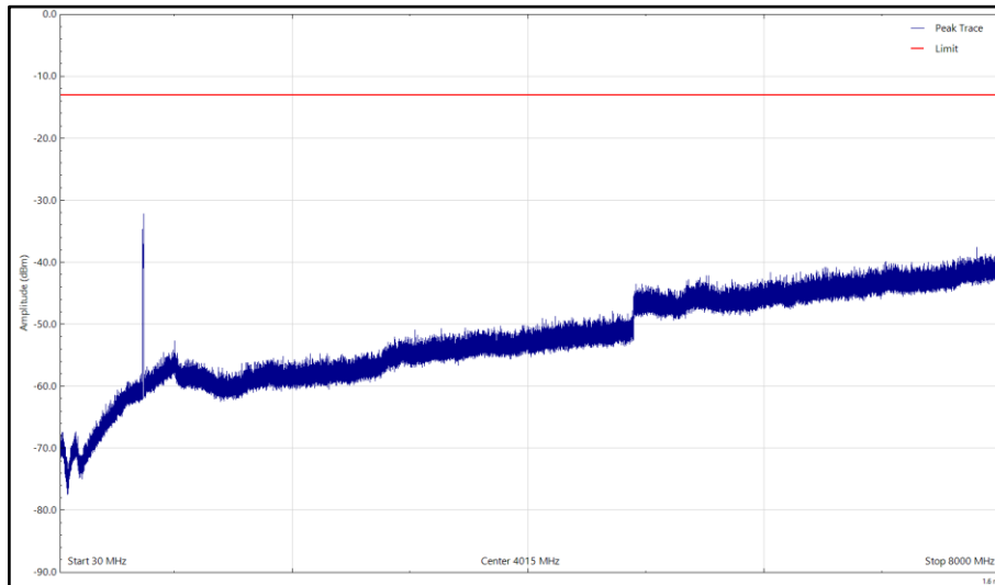
Bot - NR&NB-IoT - B85A, 733MHz, 30 MHz to 8 GHz, Horizontal (Peak)
