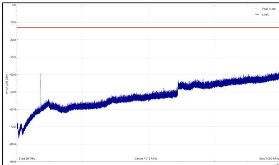
Bot - NR&NB-IoT - B85A, 733MHz, 30 MHz to 8 GHz, Vertical (Peak)
