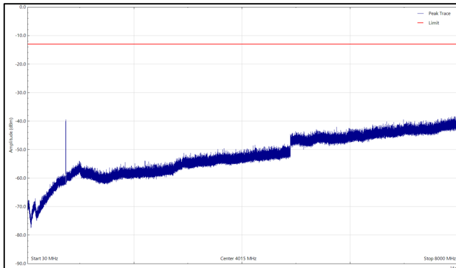
Mid - NR&NB-IoT - B85A, 736.5MHz, 30 MHz to 8 GHz, Vertical (Peak)
