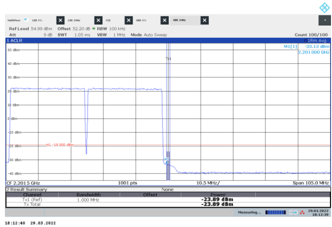
Figure 8.3-42: Conducted emission 1 MHz away from the upper band edge
