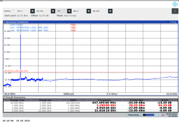
Figure 8.3-6: Conducted spurious emissions of NR 30 MHz top channel, single carrier operation
