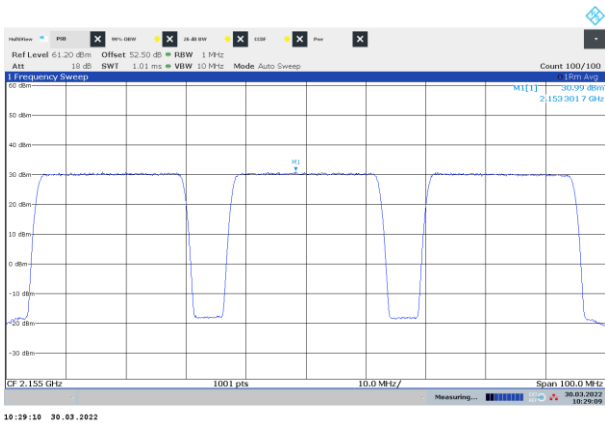
Figure 8.1-11: PSD of NR 25 MHz channel bandwidth, three-carrier operation, sample plot, mid channel
