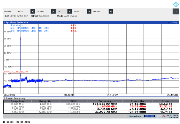
Figure 8.3-14: Conducted spurious emissions of NR 30 MHz two-carrier operation, top
