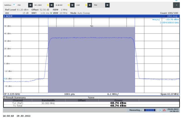
Figure 8.1-16: Power of NR 30 MHz channel bandwidth, single carrier operation, sample plot, bottom channel
