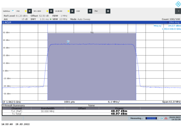
Figure 8.2-17: Power of NR 30 MHz channel bandwidth, single carrier operation, sample plot, mid channel
