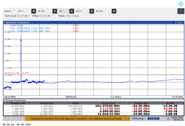
Figure 8.3-22: Conducted spurious emissions of NR 40 MHz three-carrier operation 2 x NR 40 MHz+ 1 x NR 5 MHz, top
