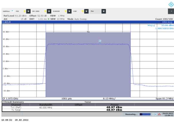
Figure 8.2-21: Power of NR 40 MHz channel bandwidth, single carrier operation, sample plot, top channel
