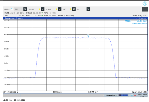
Figure 8.2-2: PSD of NR 25 MHz channel bandwidth, single carrier operation, sample plot, mid channel
