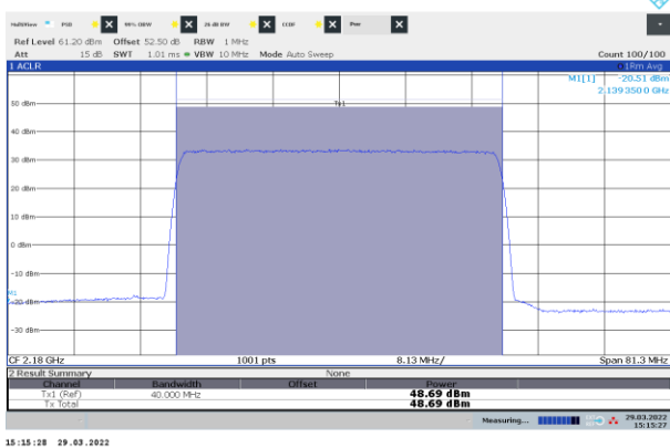
Figure 8.1-21: Power of NR 40 MHz channel bandwidth, single carrier operation, sample plot, top channel
