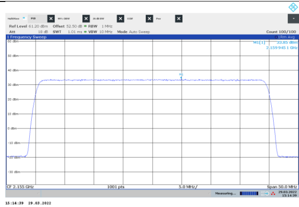
Figure 8.1-8: PSD of NR 40 MHz channel bandwidth, single carrier operation, sample plot, mid channel
