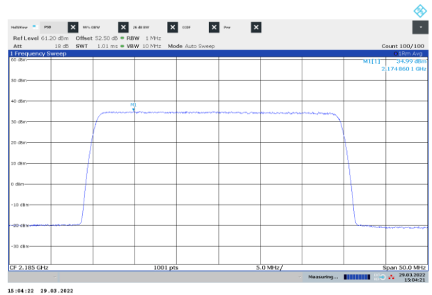
Figure 8.1-6: PSD of NR 30 MHz channel bandwidth, single carrier operation, sample plot, top channel
