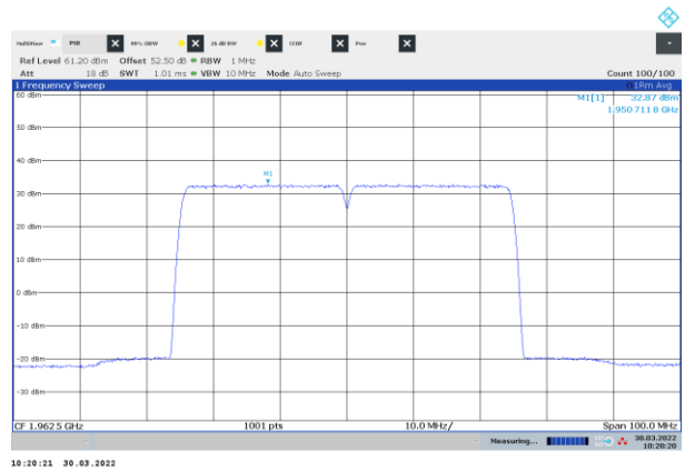
Figure 8.2-10: PSD of NR 25 MHz channel bandwidth, two-carrier operation, sample plot, middle channels
