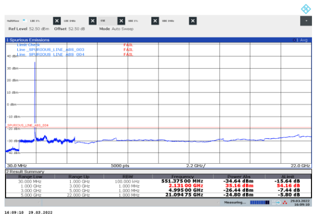
Figure 8.3-4: Conducted spurious emissions of NR 30 MHz bottom channel, single carrier operation
