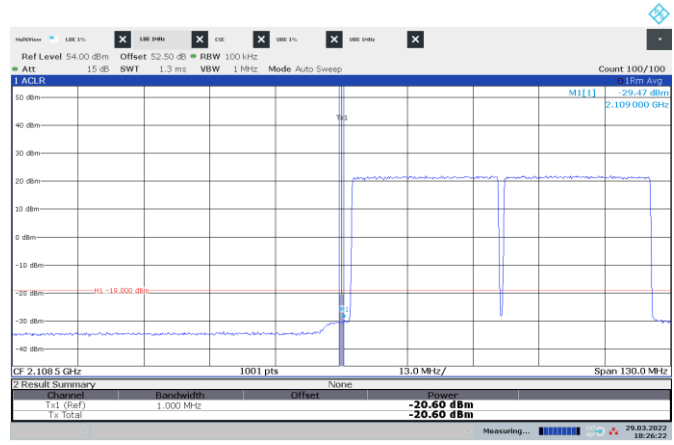
Figure 8.3-44: Conducted emission 1 MHz away from the lower band edge
