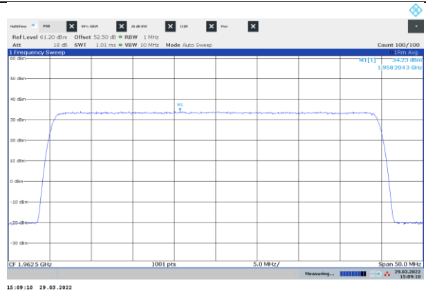
Figure 8.2-8: PSD of NR 40 MHz channel bandwidth, single carrier operation, sample plot, mid channel
