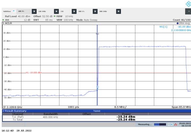
Figure 8.3-35: Conducted emission at the lower band edge
