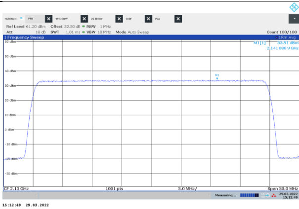
Figure 8.1-7: PSD of NR 40 MHz channel bandwidth, single carrier operation, sample plot, bottom channel
