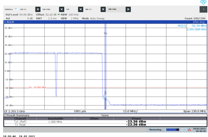
Figure 8.3-46: Conducted emission 1 MHz away from the upper band edge
