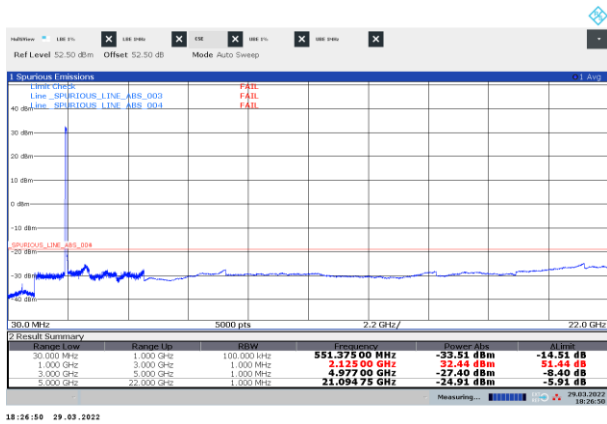
Figure 8.3-13: Conducted spurious emissions of NR 30 MHz two-carrier operation, bottom
