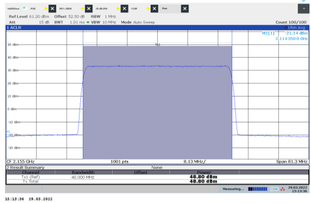
Figure 8.1-20: Power of NR 40 MHz channel bandwidth, single carrier operation, sample plot, mid channel
