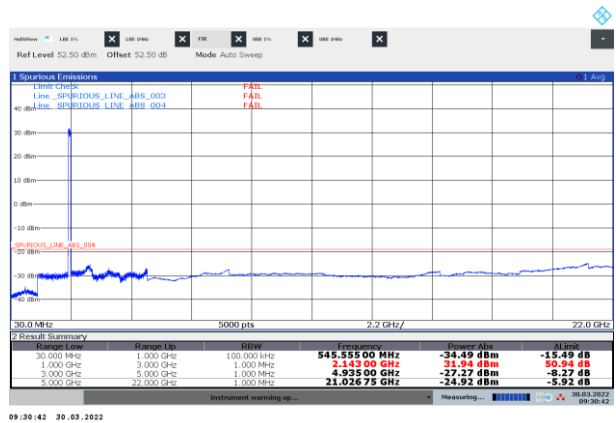
Figure 8.3-16: Conducted spurious emissions of NR 40 MHz two-carrier operation, top
