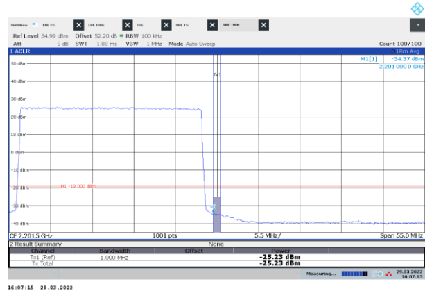
Figure 8.3-30: Conducted emission 1 MHz away from the upper band edge
