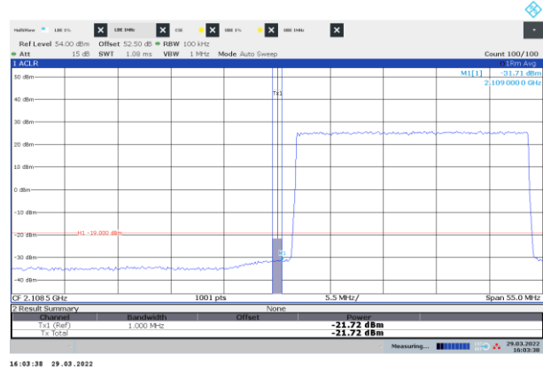
Figure 8.3-28: Conducted emission 1 MHz away from the lower band edge
