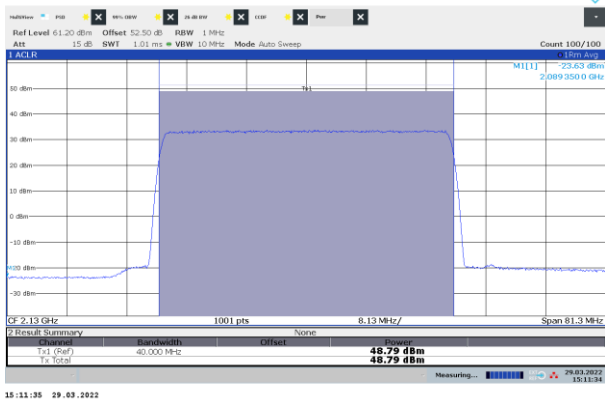
Figure 8.1-19: Power of NR 40 MHz channel bandwidth, single carrier operation, sample plot, bottom channel
