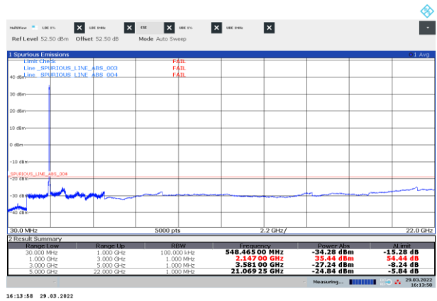
Figure 8.3-8: Conducted spurious emissions of NR 40 MHz mid channel, single carrier operation
