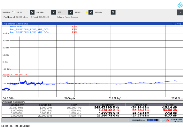
Figure 8.3-3: Conducted spurious emissions of NR 25 MHz top channel, single carrier operation
