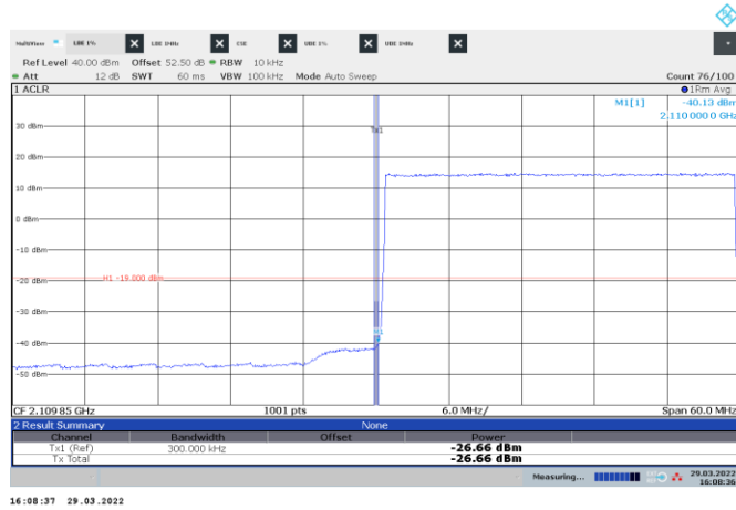
Figure 8.3-31: Conducted emission at the lower band edge
