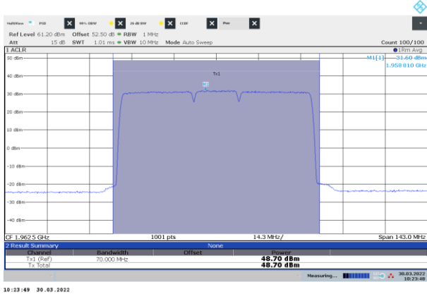
Figure 8.2-23: Power of NR 25 MHz and 15 MHz channel bandwidth, three-carrier operation (2x 25 MHz + 1x15 MHz), sample plot, mid channel
