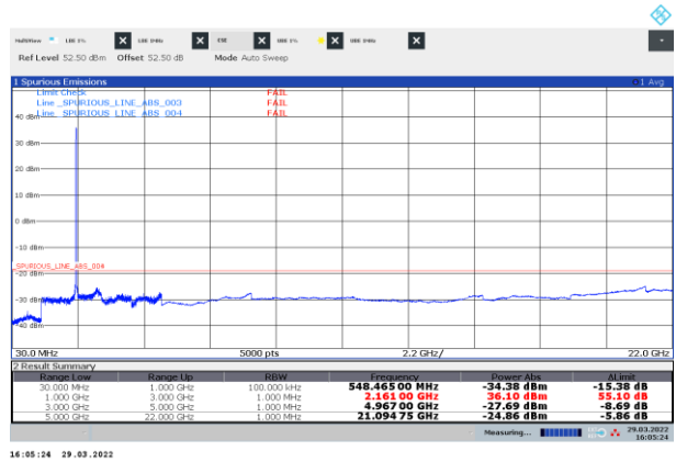
Figure 8.3-2: Conducted spurious emissions of NR 25 MHz mid channel, single carrier operation
