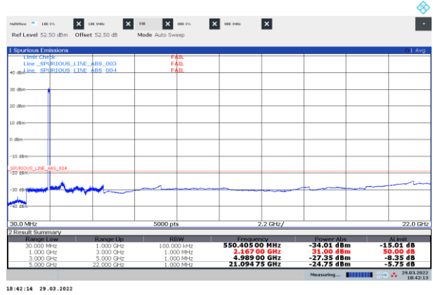
Figure 8.3-20: Conducted spurious emissions of NR 30 MHz three-carrier operation, top
