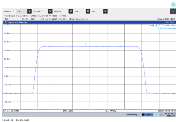
Figure 8.1-5: PSD of NR 30 MHz channel bandwidth, single carrier operation, sample plot, mid channel
