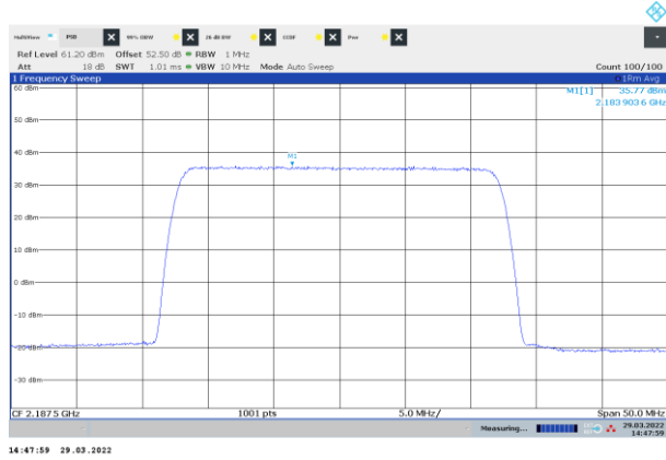
Figure 8.1-3: PSD of NR 25 MHz channel bandwidth, single carrier operation, sample plot, top channel
