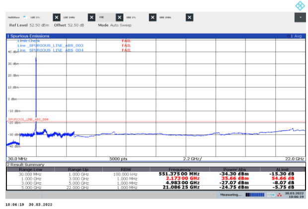
Figure 8.3-24: Conducted spurious emissions of multi-RAT operation, LTE 5 MHz + NR 25 MHz, top
