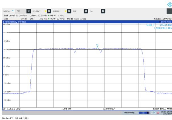
Figure 8.2-11: PSD of NR 25 MHz and 15 MHz channel bandwidth, three-carrier operation (2x 25 MHz + 1x15 MHz), sample plot, mid channel
