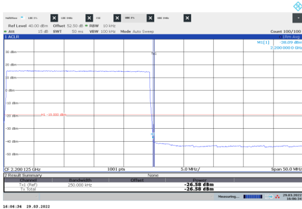
Figure 8.3-29: Conducted emission at the upper band edge
