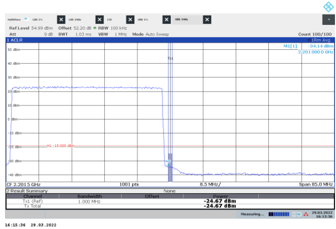
Figure 8.3-38: Conducted emission 1 MHz away from the upper band edge
