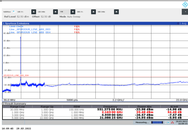
Figure 8.3-5: Conducted spurious emissions of NR 30 MHz mid channel, single carrier operation
