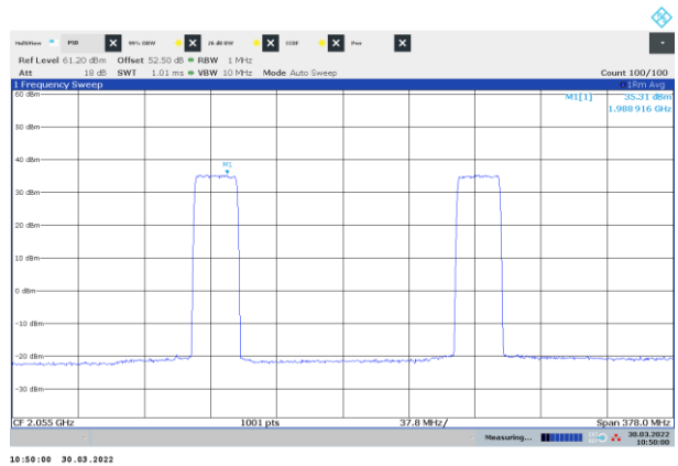
Figure 8.2-12: PSD of NR 25 MHz channel bandwidth, two-carrier operation (1x 25 MHz band 25 + 1x 25 MHz band 66), sample plot, top channel band 25 and bottom channel band 66
