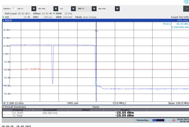
Figure 8.3-45: Conducted emission at the upper band edge
