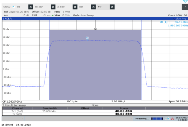
Figure 8.2-15: Power of NR 25 MHz channel bandwidth, single carrier operation, sample plot, top channel
