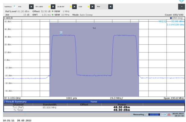
Figure 8.1-22: Power of NR 25 MHz channel bandwidth, two-carrier operation, sample plot, bottom and top channels
