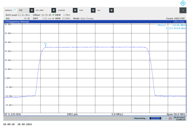
Figure 8.1-4: PSD of NR 30 MHz channel bandwidth, single carrier operation, sample plot, bottom channel
