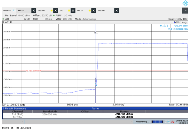
Figure 8.3-27: Conducted emission at the lower band edge
