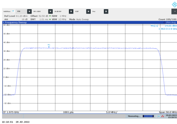
Figure 8.2-9: PSD of NR 40 MHz channel bandwidth, single carrier operation, sample plot, top channel
