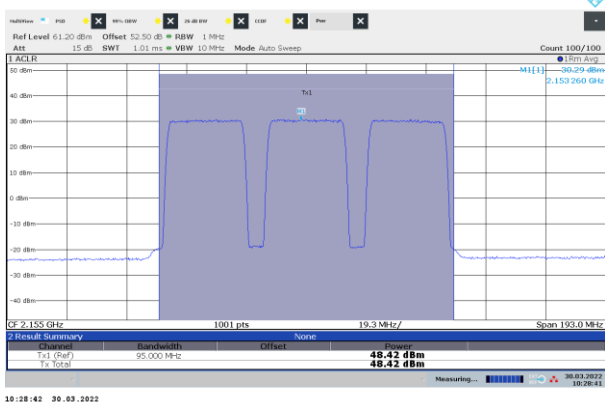
Figure 8.1-23: Power of NR 25 MHz channel bandwidth, three-carrier operation, sample plot, mid channel
