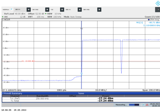
Figure 8.3-39: Conducted emission at the lower band edge
