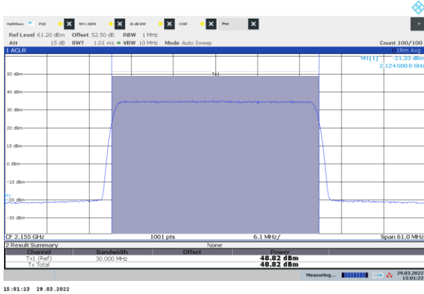
Figure 8.1-17: Power of NR 30 MHz channel bandwidth, single carrier operation, sample plot, mid channel
