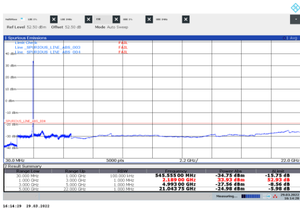
Figure 8.3-9: Conducted spurious emissions of NR 40 MHz top channel, single carrier operation
