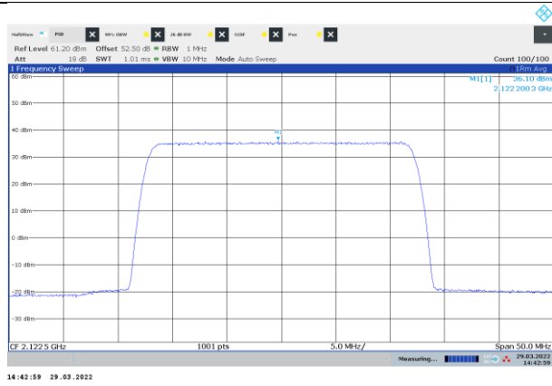
Figure 8.1-1: PSD of NR 25 MHz channel bandwidth, single carrier operation, sample plot, bottom channel
