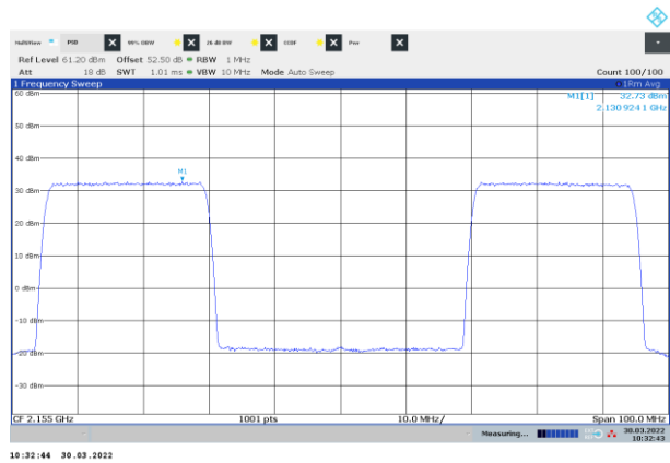
Figure 8.1-10: PSD of NR 25 MHz channel bandwidth, two-carrier operation, sample plot, bottom and top channels
