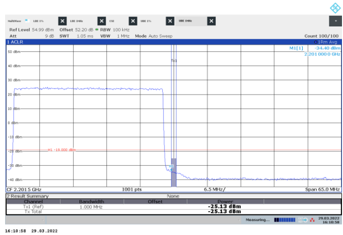
Figure 8.3-34: Conducted emission 1 MHz away from the upper band edge
