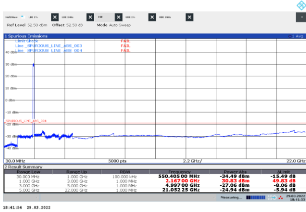
Figure 8.3-19: Conducted spurious emissions of NR 30 MHz three-carrier operation, bottom
