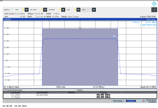
Figure 8.2-20: Power of NR 40 MHz channel bandwidth, single carrier operation, sample plot, mid channel
