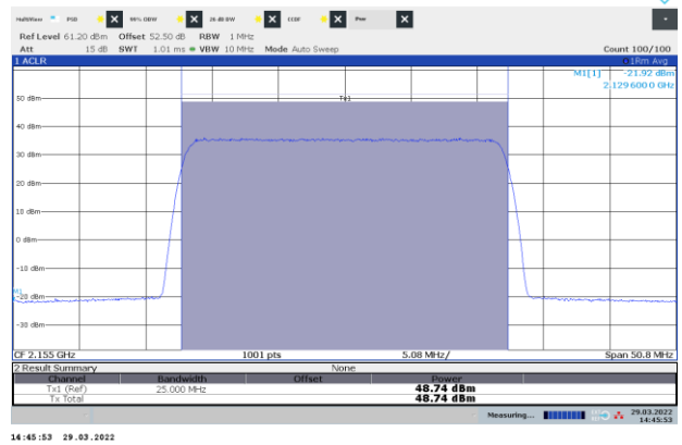
Figure 8.1-14: Power of NR 25 MHz channel bandwidth, single carrier operation, sample plot, mid channel
