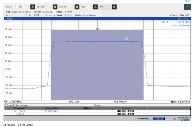
Figure 8.2-16: Power of NR 30 MHz channel bandwidth, single carrier operation, sample plot, bottom channel
