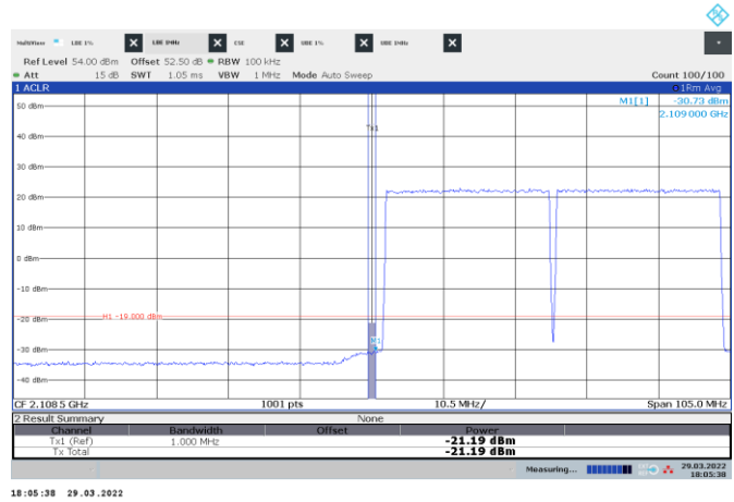
Figure 8.3-40: Conducted emission 1 MHz away from the lower band edge
