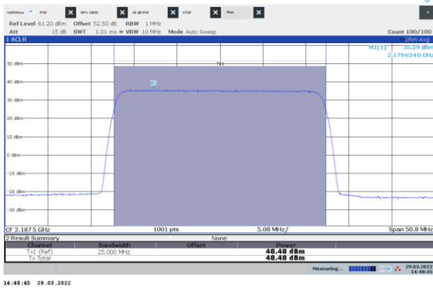
Figure 8.1-15: Power of NR 25 MHz channel bandwidth, single carrier operation, sample plot, top channel
