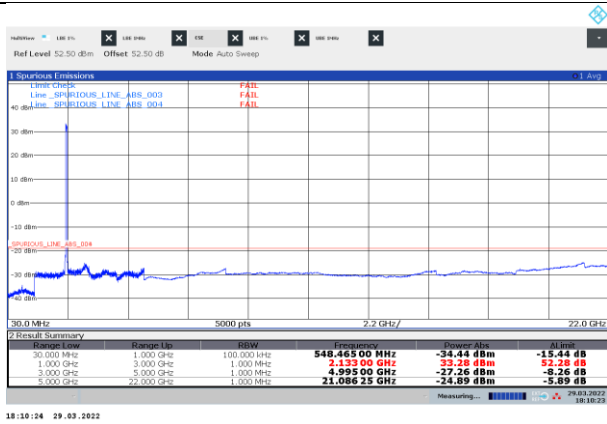
Figure 8.3-11: Conducted spurious emissions of NR 25 MHz two-carrier operation, middle
