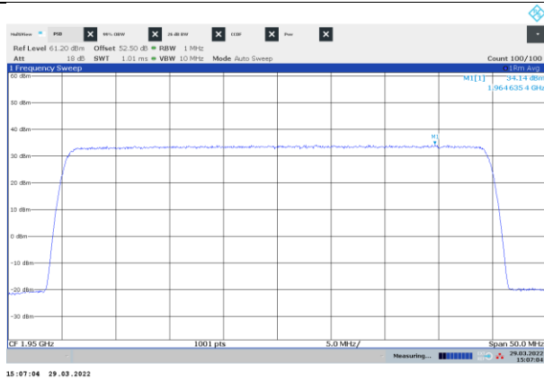
Figure 8.2-7: PSD of NR 40 MHz channel bandwidth, single carrier operation, sample plot, bottom channel
