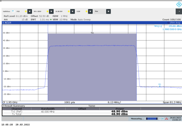
Figure 8.2-19: Power of NR 40 MHz channel bandwidth, single carrier operation, sample plot, bottom channel
