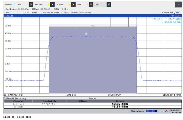
Figure 8.2-14: Power of NR 25 MHz channel bandwidth, single carrier operation, sample plot, mid channel
