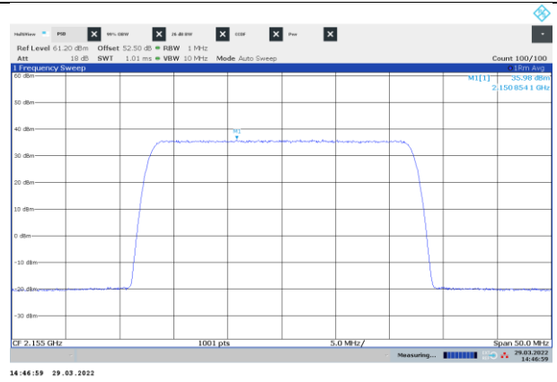
Figure 8.1-2: PSD of NR 25 MHz channel bandwidth, single carrier operation, sample plot, mid channel
