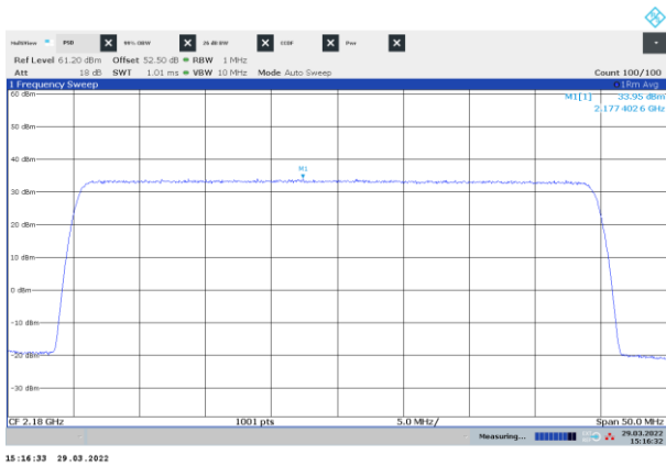
Figure 8.1-9: PSD of NR 40 MHz channel bandwidth, single carrier operation, sample plot, top channel
