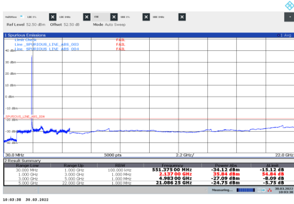
Figure 8.3-23: Conducted spurious emissions of multi-RAT operation, LTE 5 MHz + NR 25 MHz, bottom
