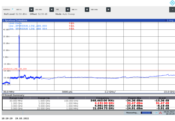
Figure 8.3-17: Conducted spurious emissions of NR 25 MHz three-carrier operation, bottom
