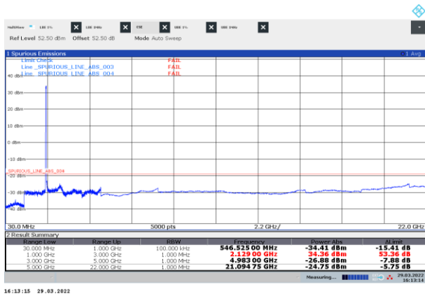
Figure 8.3-7: Conducted spurious emissions of NR 40 MHz bottom channel, single carrier operation
