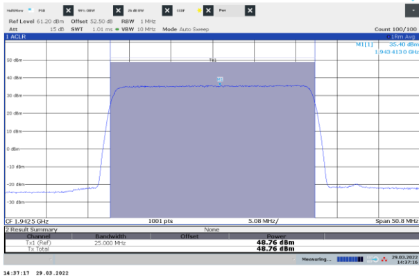
Figure 8.2-13: Power of NR 25 MHz channel bandwidth, single carrier operation, sample plot, bottom channel
