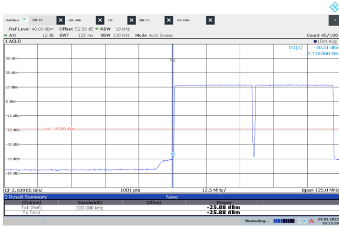
Figure 8.3-43: Conducted emission at the lower band edge
