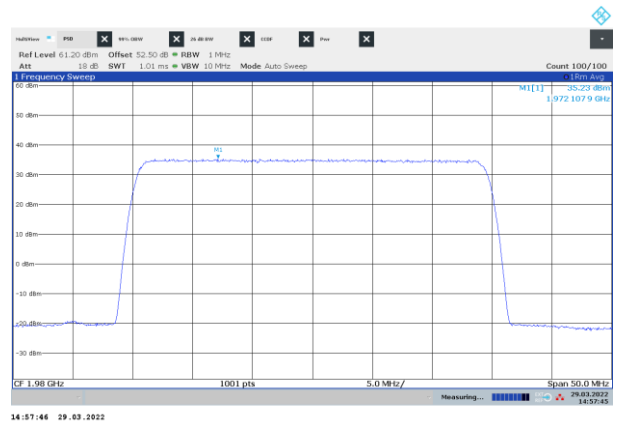
Figure 8.2-6: PSD of NR 30 MHz channel bandwidth, single carrier operation, sample plot, top channel
