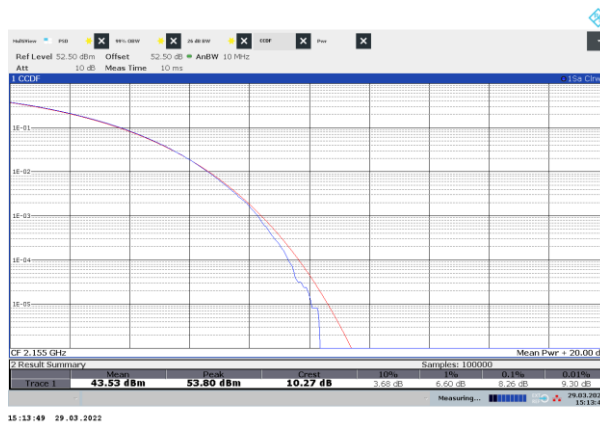
Figure 8.1-27: CCDF sample plot, NR 40 MHz channel bandwidth
