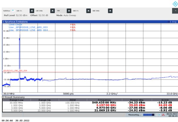
Figure 8.3-21: Conducted spurious emissions of NR 40 MHz three-carrier operation 2 x NR 40 MHz+ 1 x NR 5 MHz, bottom
