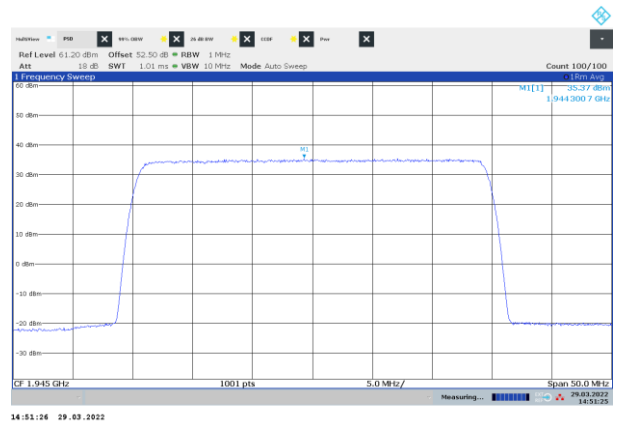
Figure 8.2-4: PSD of NR 30 MHz channel bandwidth, single carrier operation, sample plot, bottom channel
