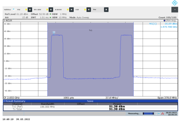
Figure 8.2-24: Power of NR 25 MHz channel bandwidth, two-carrier operation (1x 25 MHz band 25 + 1x 25 MHz band 66), sample plot, top channel band 25 and bottom channel band 66
