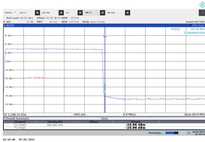
Figure 8.3-33: Conducted emission at the upper band edge
