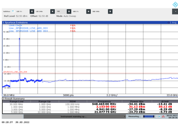
Figure 8.3-15: Conducted spurious emissions of NR 40 MHz two-carrier operation, bottom
