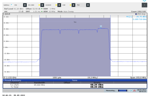
Figure 8.1-24: Power of NR 25 MHz and 15 MHz channel bandwidth, four-carrier operation (3 × 25 MHz + 1 × 15 MHz), sample plot, mid channel
