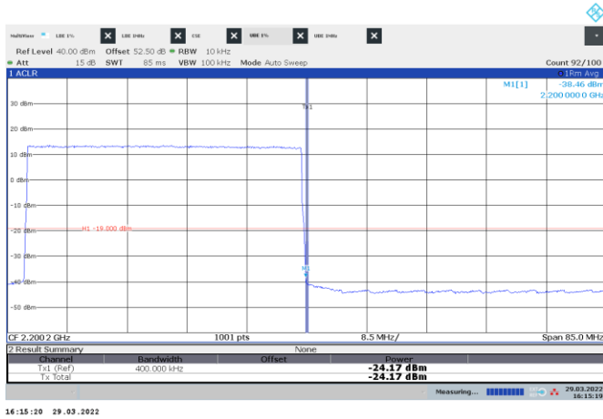
Figure 8.3-37: Conducted emission at the upper band edge
