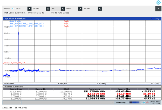
Figure 8.3-18: Conducted spurious emissions of NR 25 MHz three-carrier operation, top
