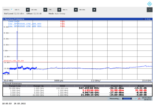
Figure 8.3-10: Conducted spurious emissions of NR 25 MHz two-carrier operation, bottom
