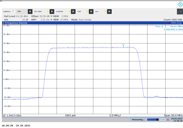
Figure 8.2-1: PSD of NR 25 MHz channel bandwidth, single carrier operation, sample plot, bottom channel
