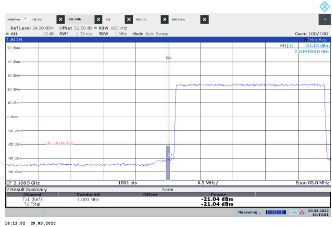
Figure 8.3-36: Conducted emission 1 MHz away from the lower band edge
