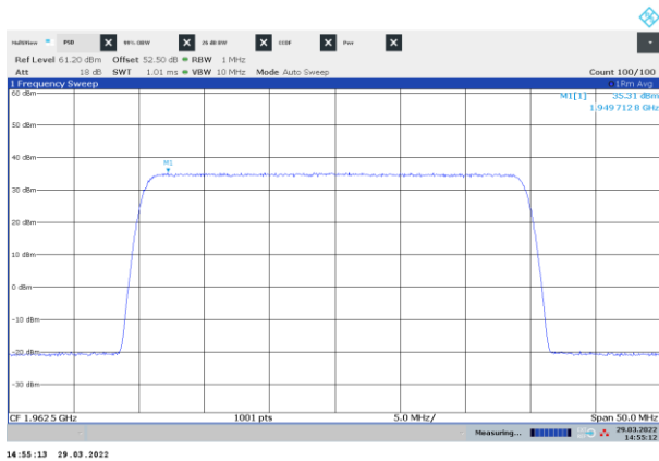
Figure 8.2-5: PSD of NR 30 MHz channel bandwidth, single carrier operation, sample plot, mid channel
