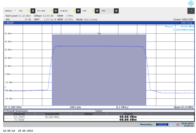
Figure 8.1-18: Power of NR 30 MHz channel bandwidth, single carrier operation, sample plot, top channel
