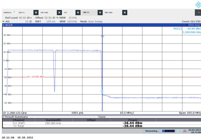
Figure 8.3-41: Conducted emission at the upper band edge
