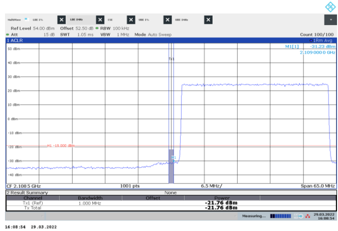
Figure 8.3-32: Conducted emission 1 MHz away from the lower band edge
