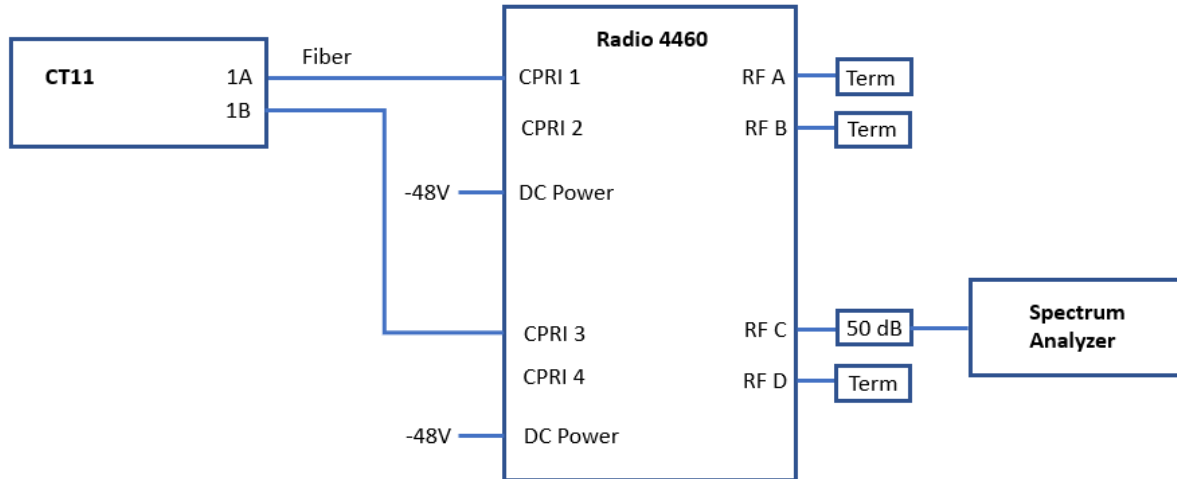
Figure 1.1-1: Setup diagram – Radio Compliance
