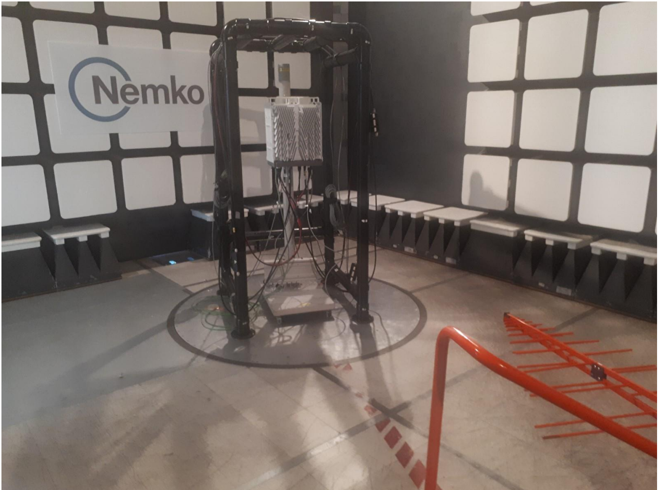
Figure 1.3-1: EUT Set-up photo for Radiated Compliance Testing
