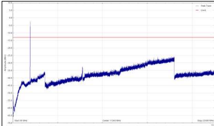
Bot - NR&NB-IoT - B2, 1940MHz, 30 MHz to 22.5 GHz, Horizontal (Peak)
