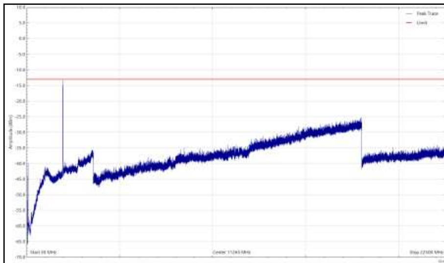
Mid - NR&NB-IoT - B25, 1962.5MHz, 30 MHz to 22.5 GHz, Vertical (Peak)
