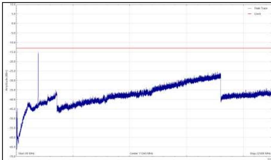
Bot - NR&NB-IoT - B2, 1940MHz, 30 MHz to 22.5 GHz, Vertical (Peak)
