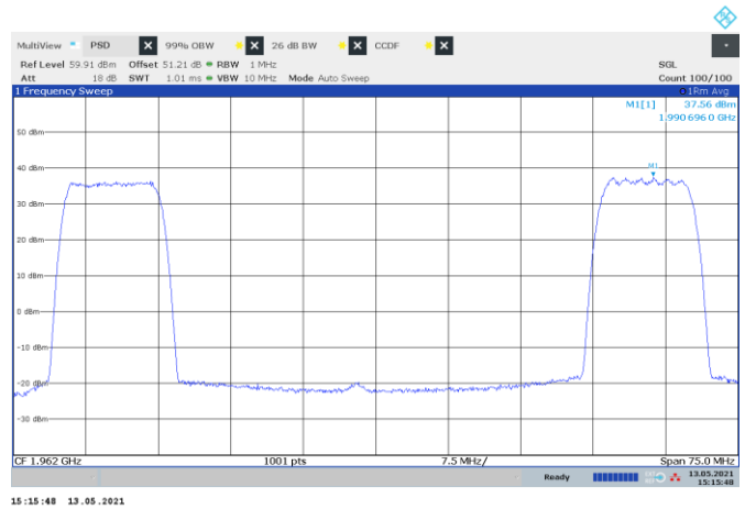
Figure 8.2-44: PSD of multi-RAT operation, LTE 10 MHz and NR 10 MHz
