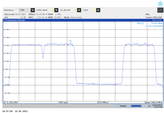
Figure 8.1-22: PSD of LTE 20 MHz channel bandwidth, multi-carrier operation, sample plot
