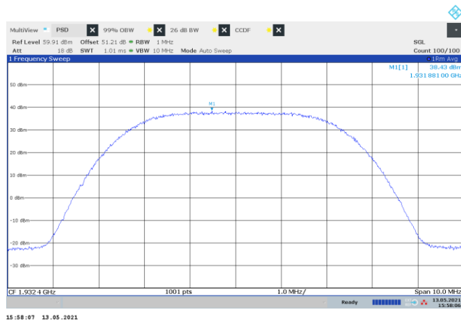
Figure 8.2-33: PSD of WCDMA, sample plot
