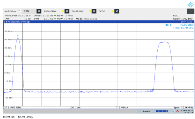
Figure 8.2-50: PSD of multi-RAT operation, GSM and WCDMA
