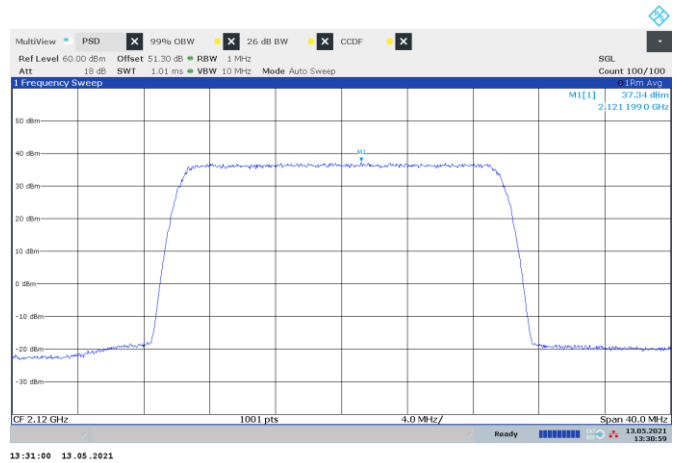
Figure 8.1-26: PSD of NR 20 MHz channel bandwidth, single carrier operation, sample plot
