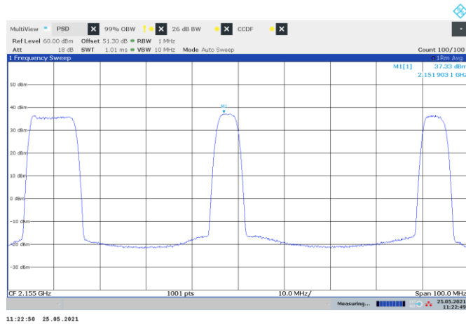
Figure 8.1-33: PSD of multi-RAT operation, LTE 10 MHz and WCDMA and NR 5 MHz
