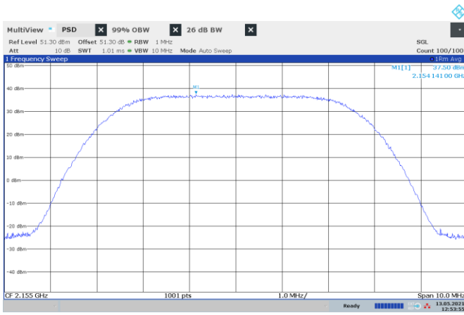
Figure 8.1-11: PSD of LTE 5 MHz channel bandwidth, single carrier operation, sample plot
