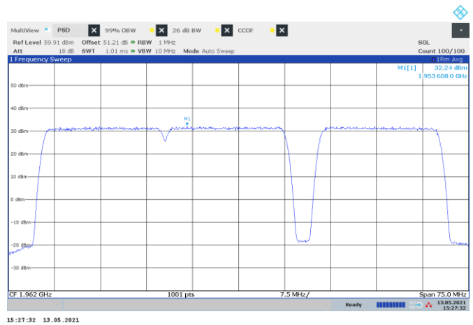
Figure 8.2-32: PSD of NR 20 MHz channel bandwidth, multi-carrier operation, sample plot
