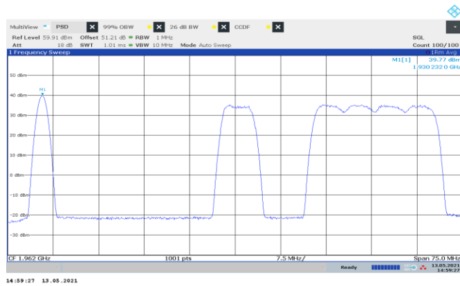
Figure 8.2-49: PSD of multi-RAT operation, GSM and LTE 5 MHz and 4xNR 5 MHz
