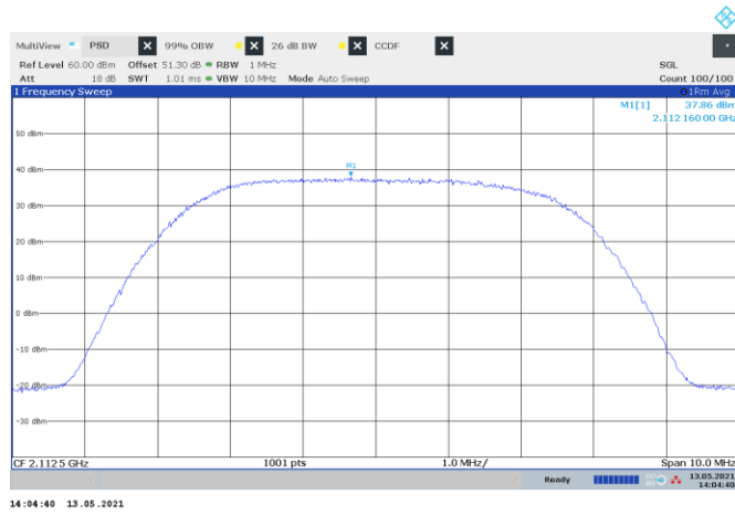
Figure 8.1-23: PSD of NR 5 MHz channel bandwidth, single carrier operation, sample plot
