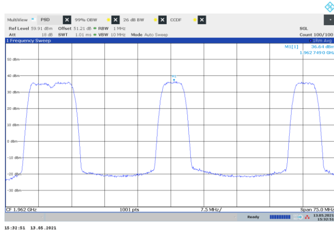
Figure 8.2-21: PSD of LTE 5 MHz channel bandwidth, multi-carrier operation, sample plot
