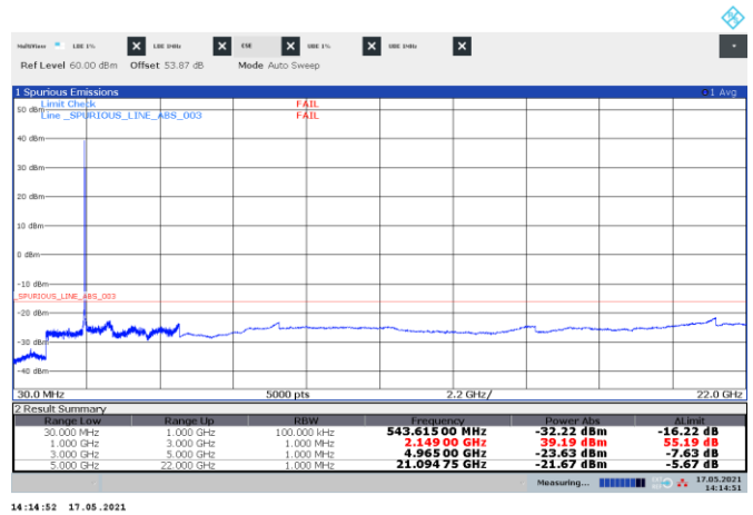
Figure 8.3-8: Conducted spurious emissions of LTE 15 MHz mid channel, single carrier operation
