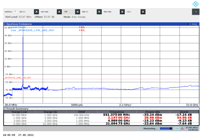
Figure 8.3-6: Conducted spurious emissions of LTE 10 MHz top channel, single carrier operation
