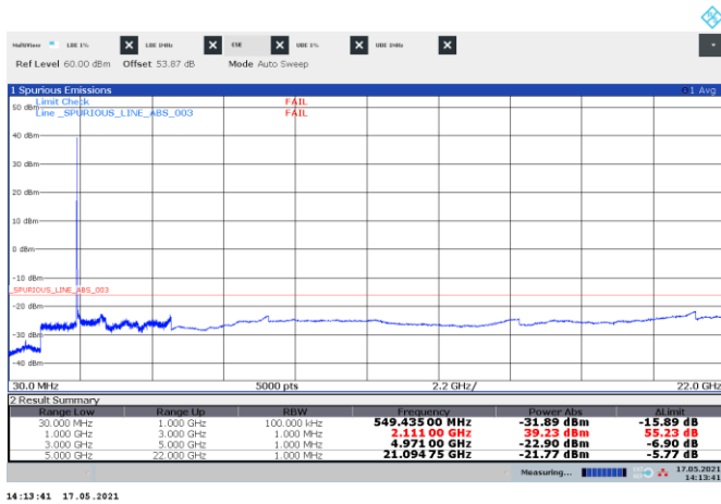
Figure 8.3-7: Conducted spurious emissions of LTE 15 MHz low channel, single carrier operation
