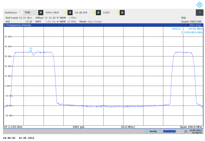
Figure 8.1-28: PSD of NR 10 MHz channel bandwidth, multi-carrier operation, sample plot
