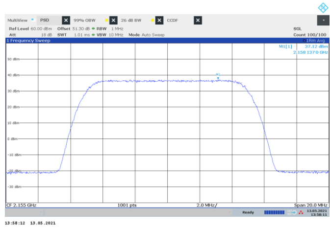
Figure 8.1-24: PSD of NR 10 MHz channel bandwidth, single carrier operation, sample plot
