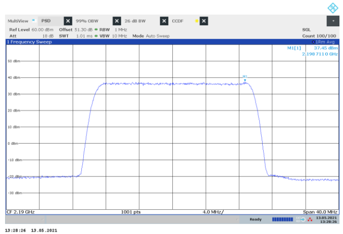
Figure 8.1-18: PSD of LTE 20 MHz channel bandwidth with IoT, single carrier operation, sample plot
