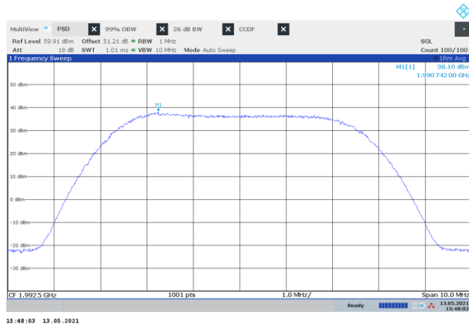
Figure 8.2-17: PSD of LTE 5 MHz channel bandwidth with guard-band, single carrier operation, sample plot
