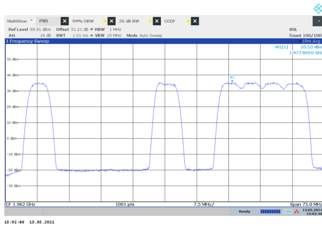
Figure 8.2-45: PSD of multi-RAT operation, WCDMA and LTE 5 MHz and 4xNR 5 MHz
