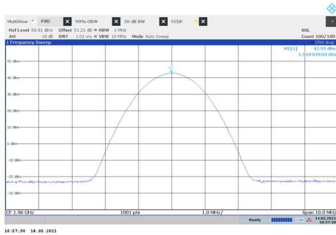
Figure 8.2-35: PSD of GSM, sample plot
