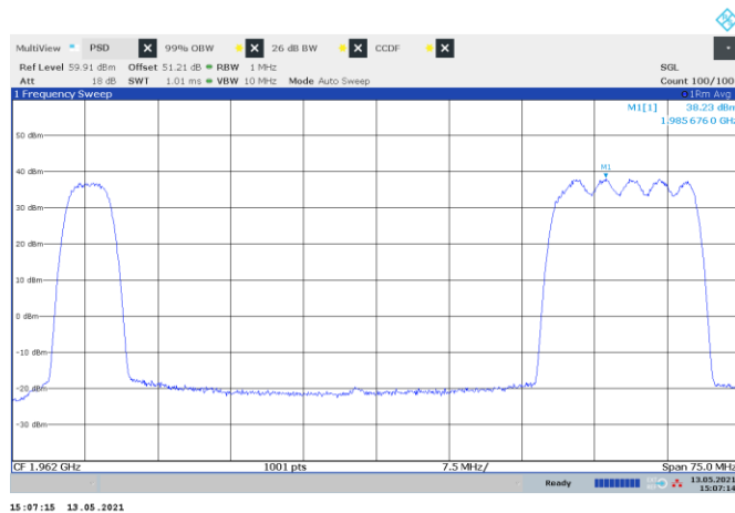
Figure 8.2-47: PSD of multi-RAT operation, WCDMA and NR 15 MHz
