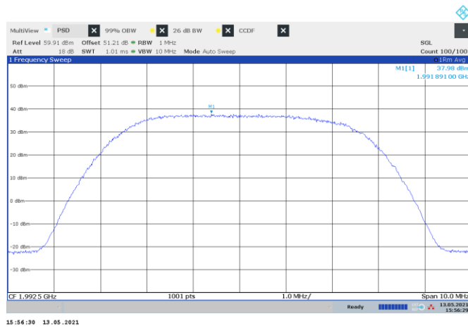
Figure 8.2-25: PSD of NR 5 MHz channel bandwidth, single carrier operation, sample plot
