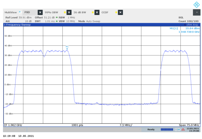
Figure 8.2-30: PSD of NR 10 MHz channel bandwidth, multi-carrier operation, sample plot
