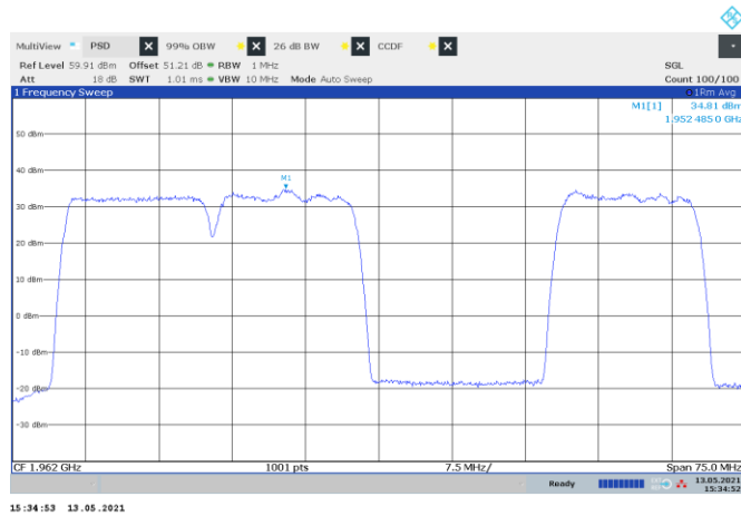
Figure 8.2-23: PSD of LTE 15 MHz channel bandwidth, multi-carrier operation, sample plot
