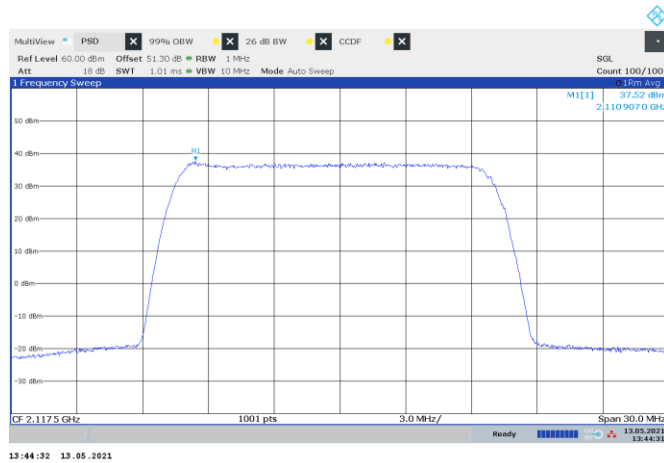
Figure 8.1-17: PSD of LTE 15 MHz channel bandwidth with IoT, single carrier operation, sample plot
