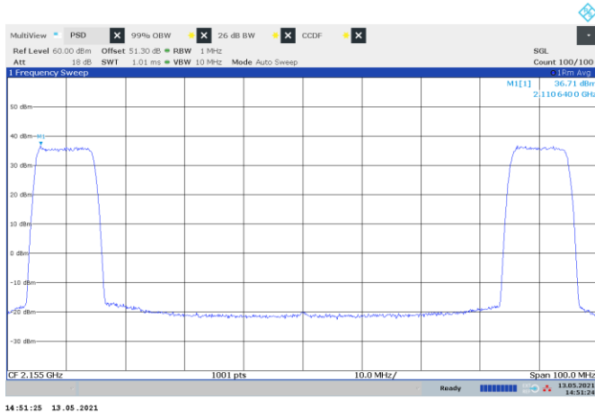
Figure 8.1-35: PSD of multi-RAT operation, LTE 10 MHz and NR 10 MHz
