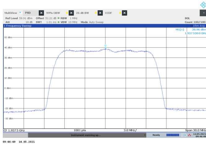
Figure 8.2-15: PSD of LTE 15 MHz channel bandwidth, single carrier operation, sample plot
