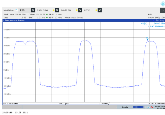
Figure 8.2-29: PSD of NR 5 MHz channel bandwidth, multi-carrier operation, sample plot
