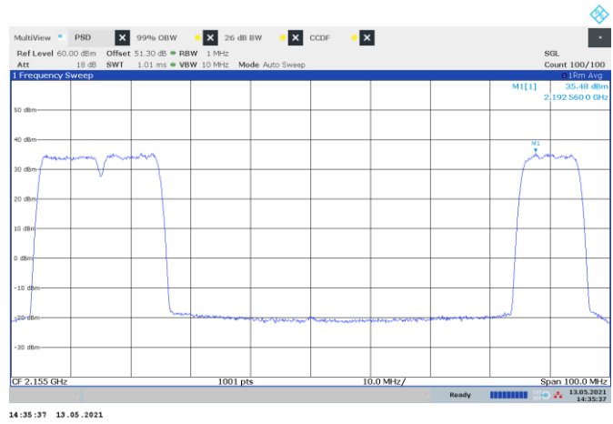
Figure 8.1-20: PSD of LTE 10 MHz channel bandwidth, multi-carrier operation, sample plot
