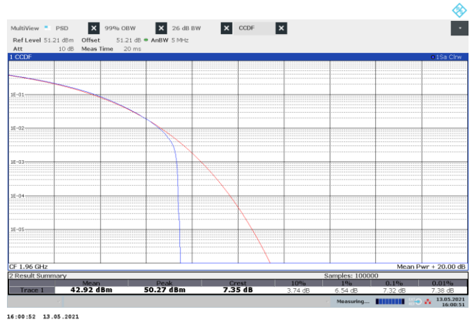
Figure 8.2-57: CCDF sample plot, WCDMA
