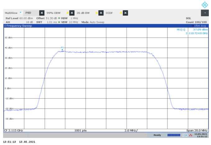
Figure 8.1-16: PSD of LTE 10 MHz channel bandwidth with IoT, single carrier operation, sample plot
