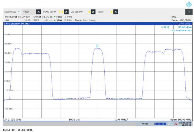
Figure 8.1-34: PSD of multi-RAT operation, WCDMA + LTE 15 MHz and NR 5 MHz and NR 10 MHz + LTE 5 MHz + NR 5 MHz
