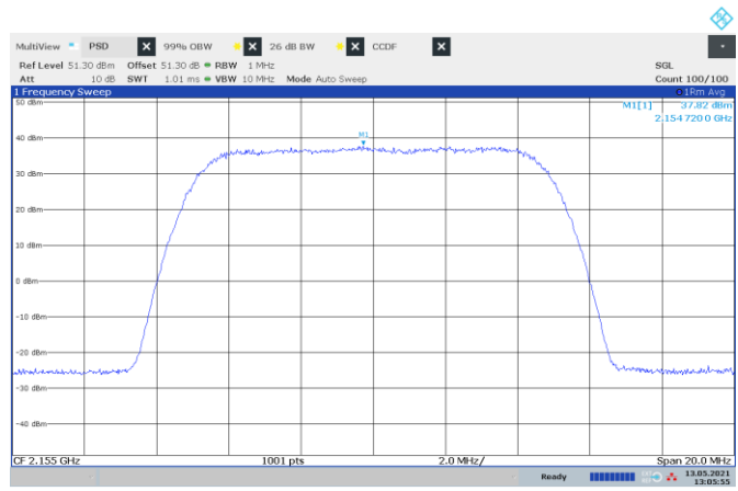
Figure 8.1-12: PSD of LTE 10 MHz channel bandwidth, single carrier operation, sample plot
