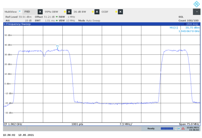
Figure 8.2-22: PSD of LTE 10 MHz channel bandwidth, multi-carrier operation, sample plot
