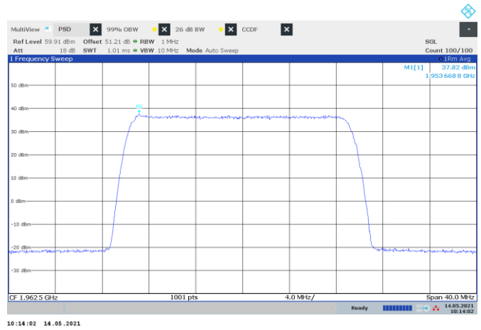
Figure 8.2-20: PSD of LTE 20 MHz channel bandwidth with IoT, single carrier operation, sample plot
