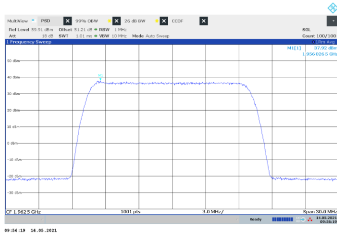
Figure 8.2-19: PSD of LTE 15 MHz channel bandwidth with IoT, single carrier operation, sample plot
