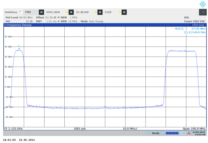
Figure 8.1-36: PSD of multi-RAT operation, WCDMA and LTE 15 MHz
