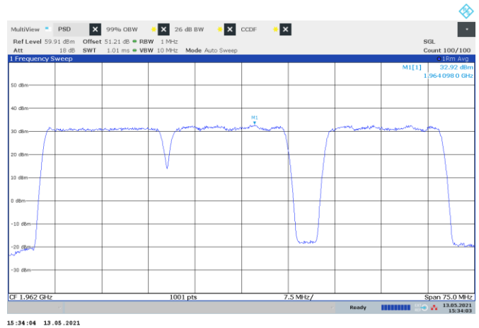
Figure 8.2-24: PSD of LTE 20 MHz channel bandwidth, multi-carrier operation, sample plot
