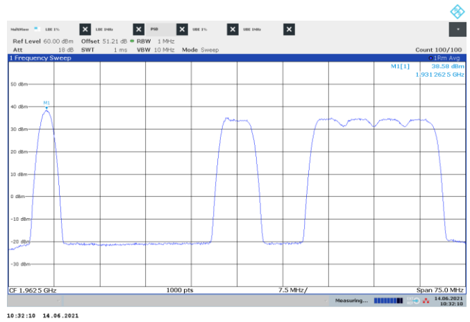
Figure 8.2-36: PSD of multi-RAT operation, CDMA and LTE 5 MHz and 4xNR 5 MHz
