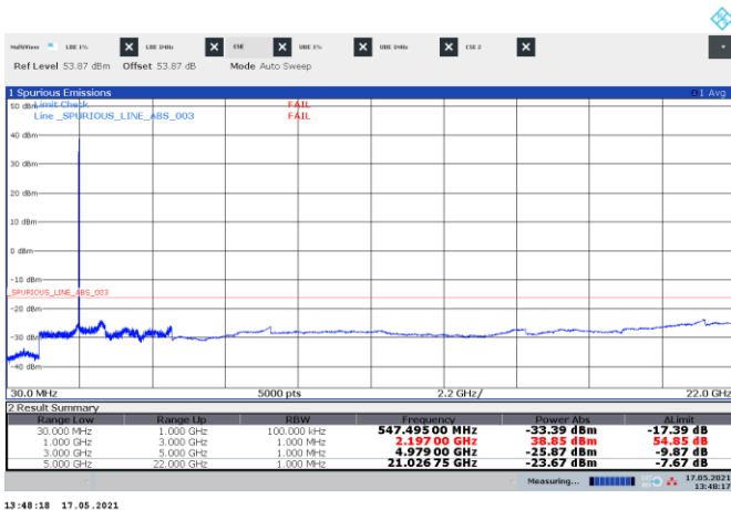
Figure 8.3-3: Conducted spurious emissions of LTE 5 MHz top channel, single carrier operation
