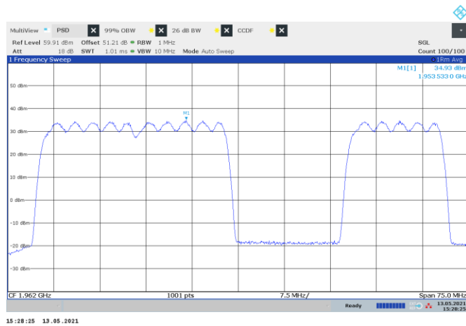
Figure 8.2-31: PSD of NR 15 MHz channel bandwidth, multi-carrier operation, sample plot
