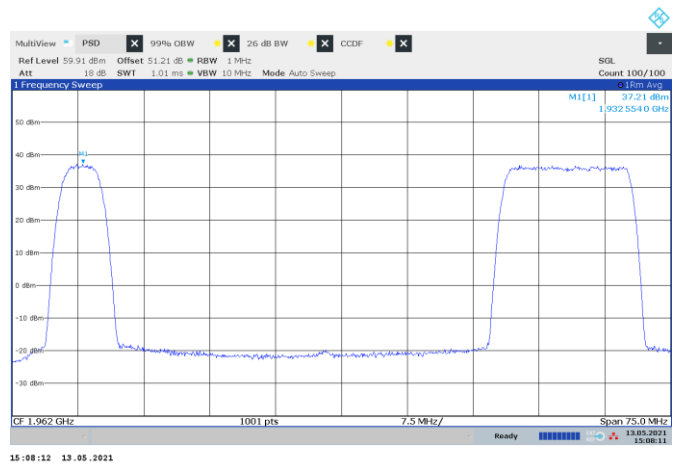
Figure 8.2-46: PSD of multi-RAT operation, WCDMA and LTE 15 MHz
