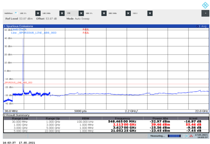
Figure 8.3-4: Conducted spurious emissions of LTE 10 MHz low channel, single carrier operation
