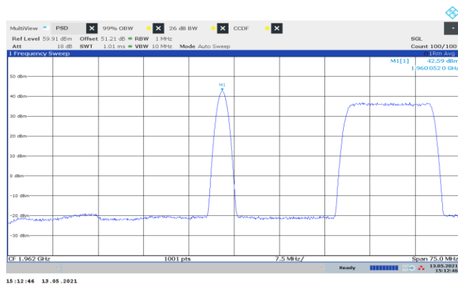
Figure 8.2-51: PSD of multi-RAT operation, GSM and LTE 15 MHz
