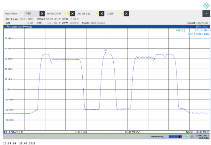
Figure 8.2-48: PSD of multi-RAT operation, WCDMA + LTE 15 MHz and NR 5 MHz and NR 10 MHz + LTE 5 MHz + NR 5 MHz
