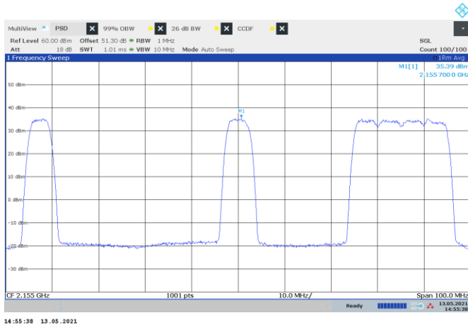
Figure 8.1-37: PSD of multi-RAT operation, WCDMA and LTE 5 MHz and 4xNR 5 MHz
