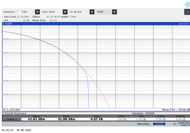
Figure 8.1-39: CCDF sample plot, LTE
