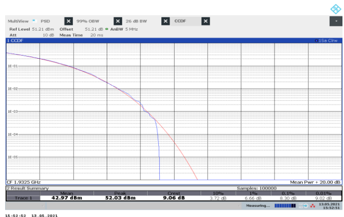
Figure 8.2-55: CCDF sample plot, NR
