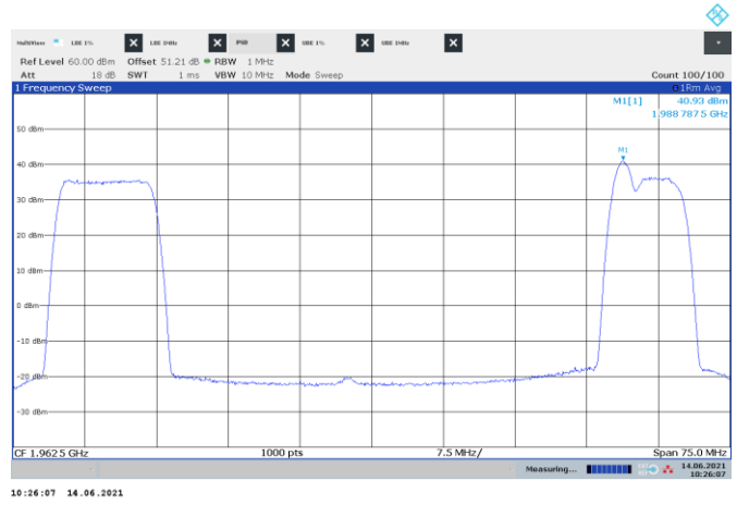
Figure 8.2-42: PSD of multi-RAT operation, LTE 10 MHz and CDMA + NR 5 MHz
