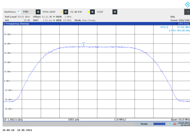
Figure 8.2-13: PSD of LTE 5 MHz channel bandwidth, single carrier operation, sample plot
