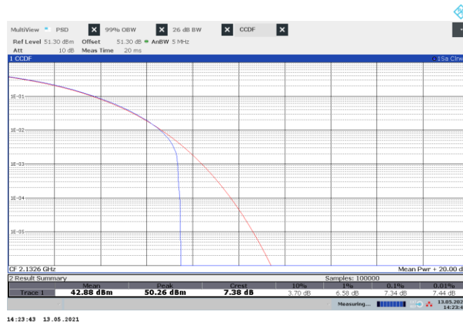
Figure 8.1-41: CCDF sample plot, WCDMA
