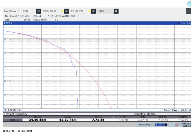
Figure 8.2-58: CCDF sample plot, GSM
