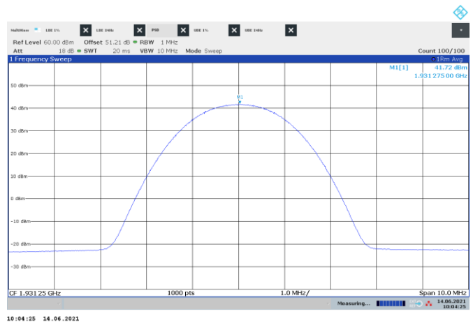
Figure 8.2-34: PSD of CDMA, sample plot
