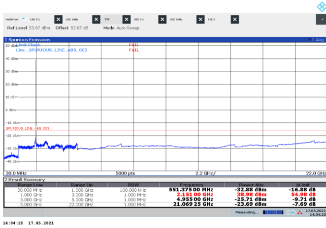
Figure 8.3-5: Conducted spurious emissions of LTE 10 MHz mid channel, single carrier operation
