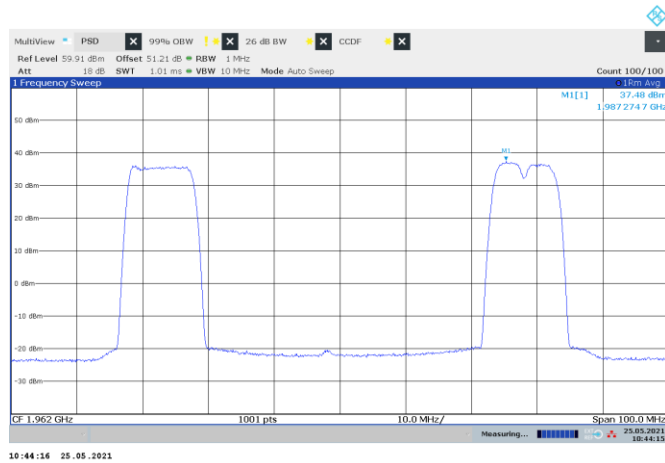
Figure 8.2-43: PSD of multi-RAT operation, LTE 10 MHz and WCDMA and NR 5 MHz
