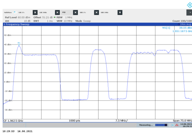
Figure 8.2-39: PSD of multi-RAT operation, CDMA + LTE 15 MHz and NR 5 MHz and NR 10 MHz + LTE 5 MHz
