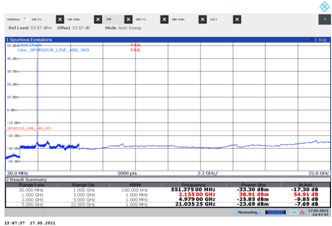
Figure 8.3-2: Conducted spurious emissions of LTE 5 MHz mid channel, single carrier operation
