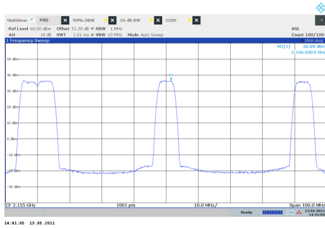
Figure 8.1-19: PSD of LTE 5 MHz channel bandwidth, multi-carrier operation, sample plot
