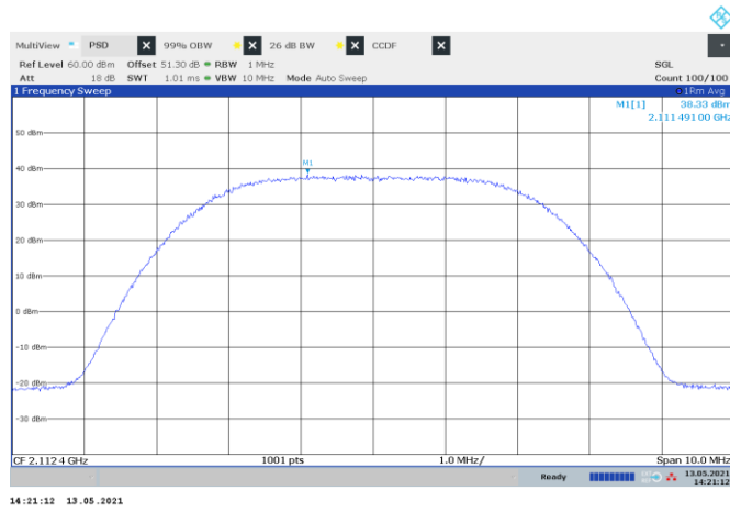
Figure 8.1-31: PSD of WCDMA, sample plot
