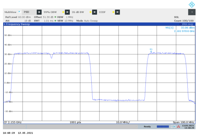
Figure 8.1-30: PSD of NR 20 MHz channel bandwidth, multi-carrier operation, sample plot
