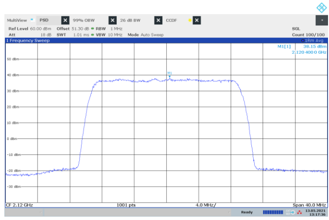
Figure 8.1-14: PSD of LTE 20 MHz channel bandwidth, single carrier operation, sample plot
