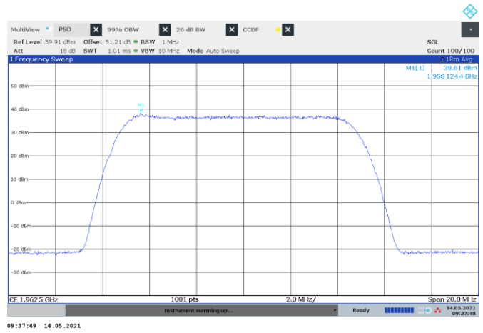
Figure 8.2-18: PSD of LTE 10 MHz channel bandwidth with IoT, single carrier operation, sample plot
