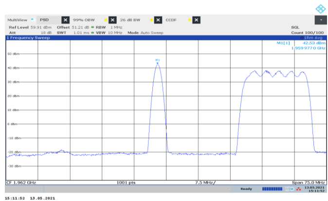
Figure 8.2-52: PSD of multi-RAT operation, GSM and NR 15 MHz
