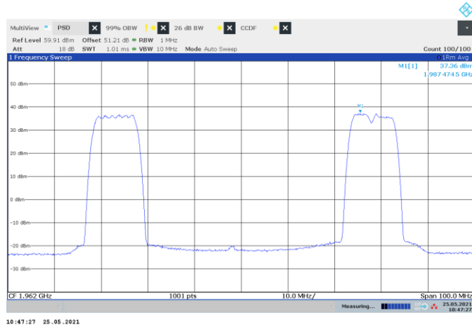
Figure 8.2-41: PSD of multi-RAT operation, LTE 5 MHz and WCDMA and NR 10 MHz
