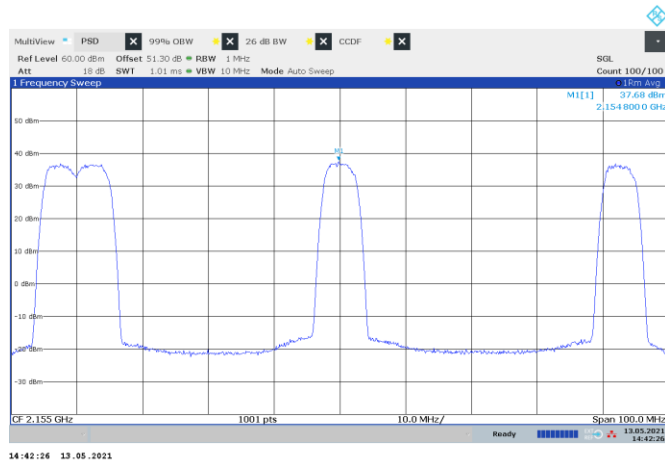
Figure 8.1-27: PSD of NR 5 MHz channel bandwidth, multi-carrier operation, sample plot
