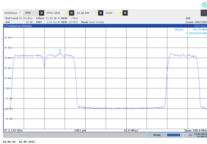
Figure 8.1-21: PSD of LTE 15 MHz channel bandwidth, multi-carrier operation, sample plot
