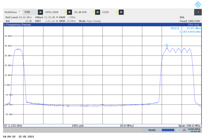
Figure 8.1-38: PSD of multi-RAT operation, WCDMA and NR 15 MHz
