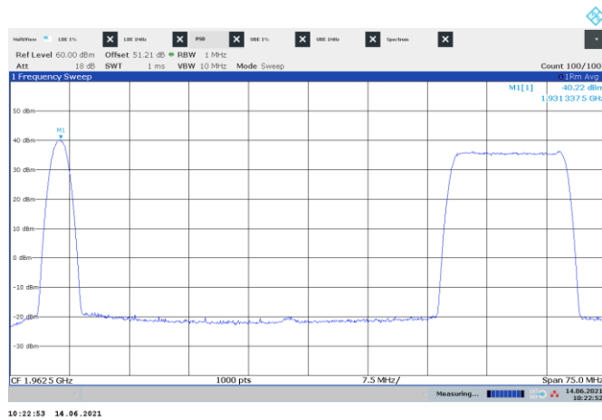
Figure 8.2-37: PSD of multi-RAT operation, CDMA and LTE 15 MHz
