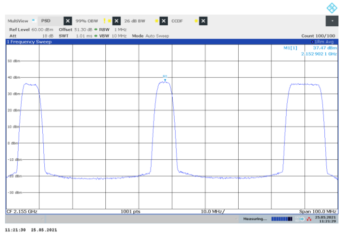
Figure 8.1-32: PSD of multi-RAT operation, LTE 5 MHz and WCDMA and NR 10 MHz
