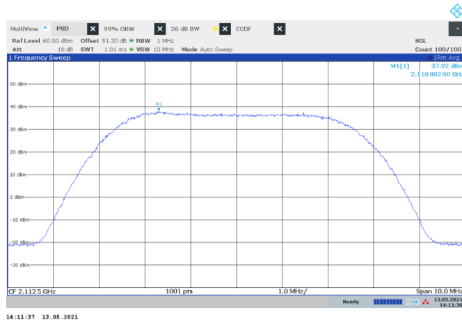
Figure 8.1-15: PSD of LTE 5 MHz channel bandwidth with guard-band, single carrier operation, sample plot
