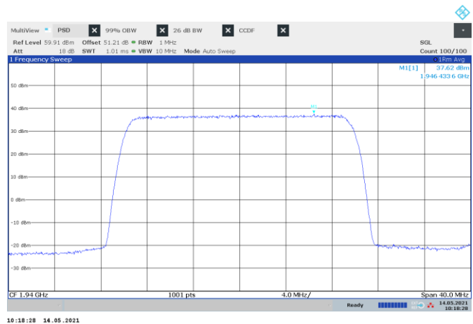
Figure 8.2-28: PSD of NR 20 MHz channel bandwidth, single carrier operation, sample plot
