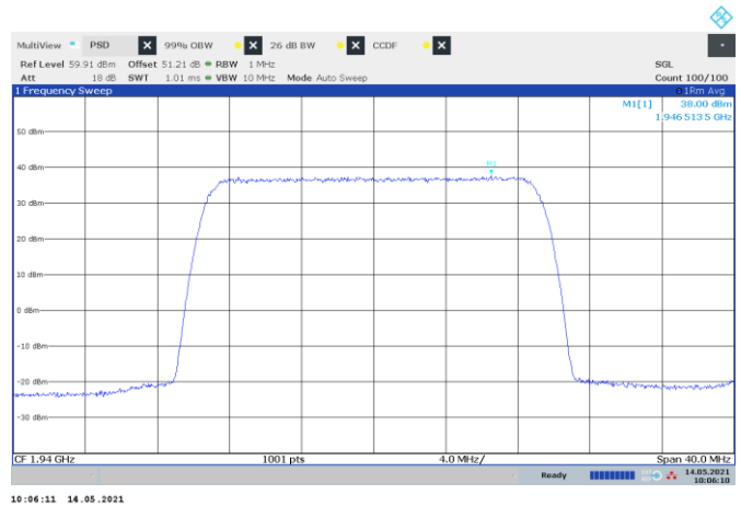
Figure 8.2-16: PSD of LTE 20 MHz channel bandwidth, single carrier operation, sample plot
