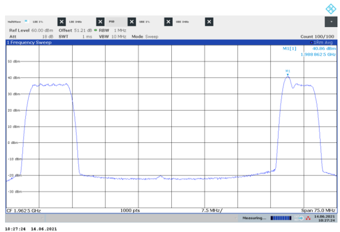
Figure 8.2-40: PSD of multi-RAT operation, NR 10 MHz and CDMA + LTE 5 MHz
