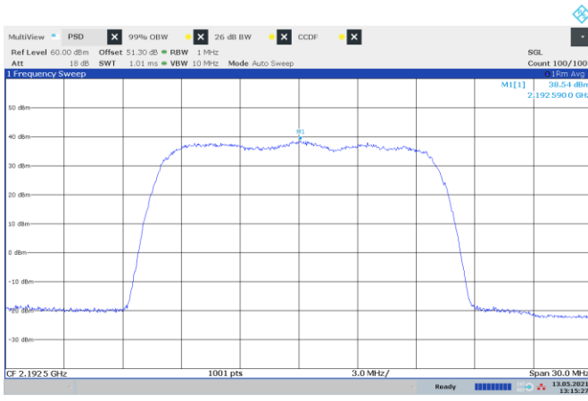
Figure 8.1-13: PSD of LTE 15 MHz channel bandwidth, single carrier operation, sample plot
