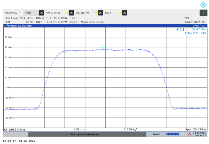
Figure 8.2-14: PSD of LTE 10 MHz channel bandwidth, single carrier operation, sample plot
