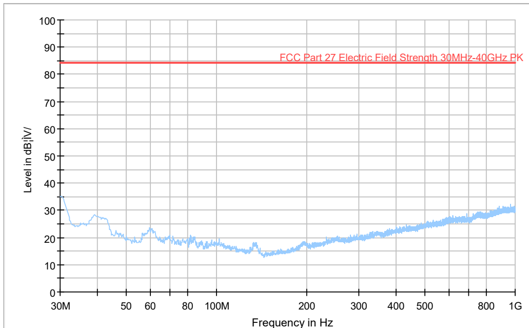
30-1000MHz, Horizontal and Vertical Full Spectrum
