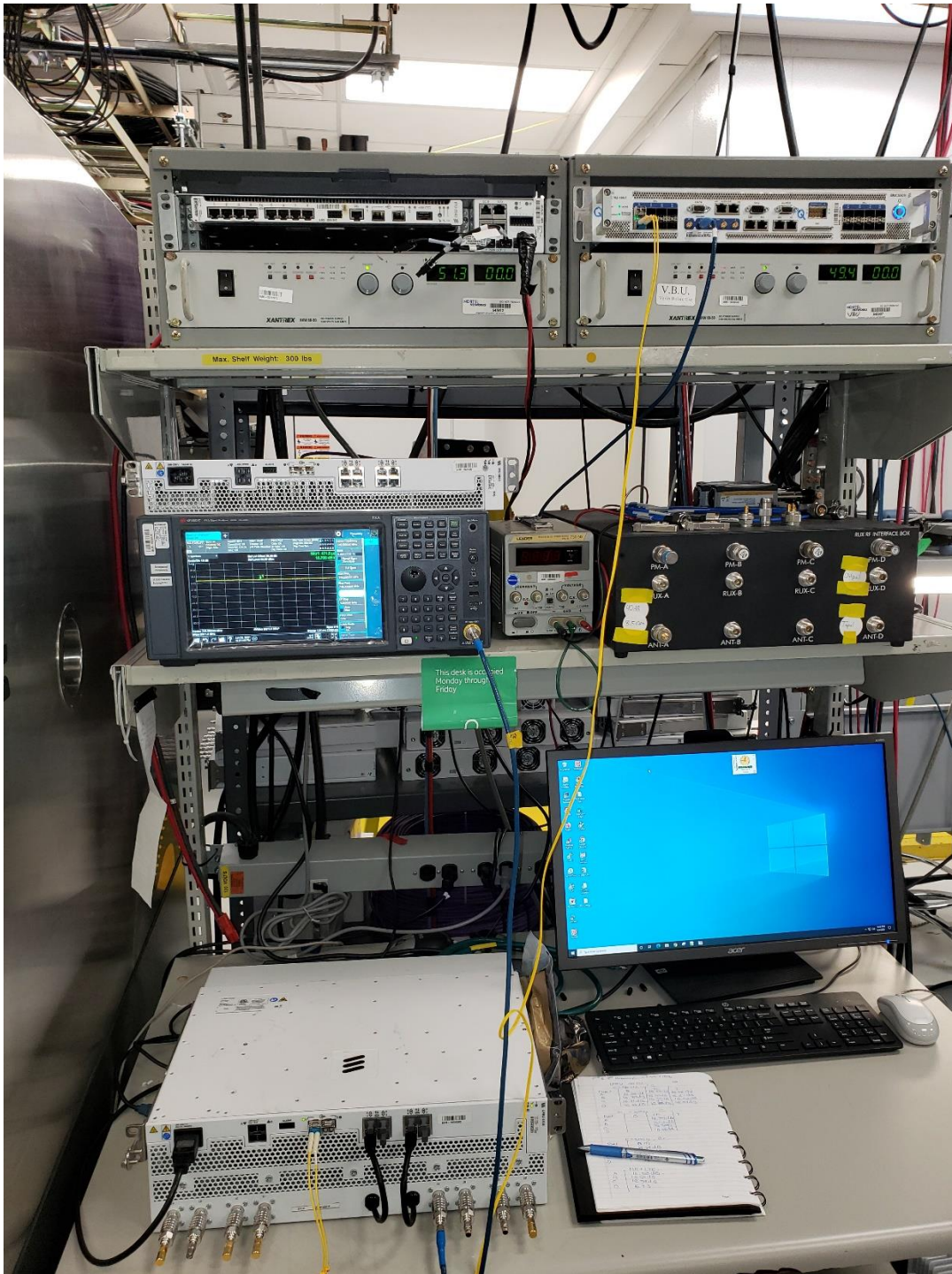
Figure 2: RF Conducted Test Equipment
