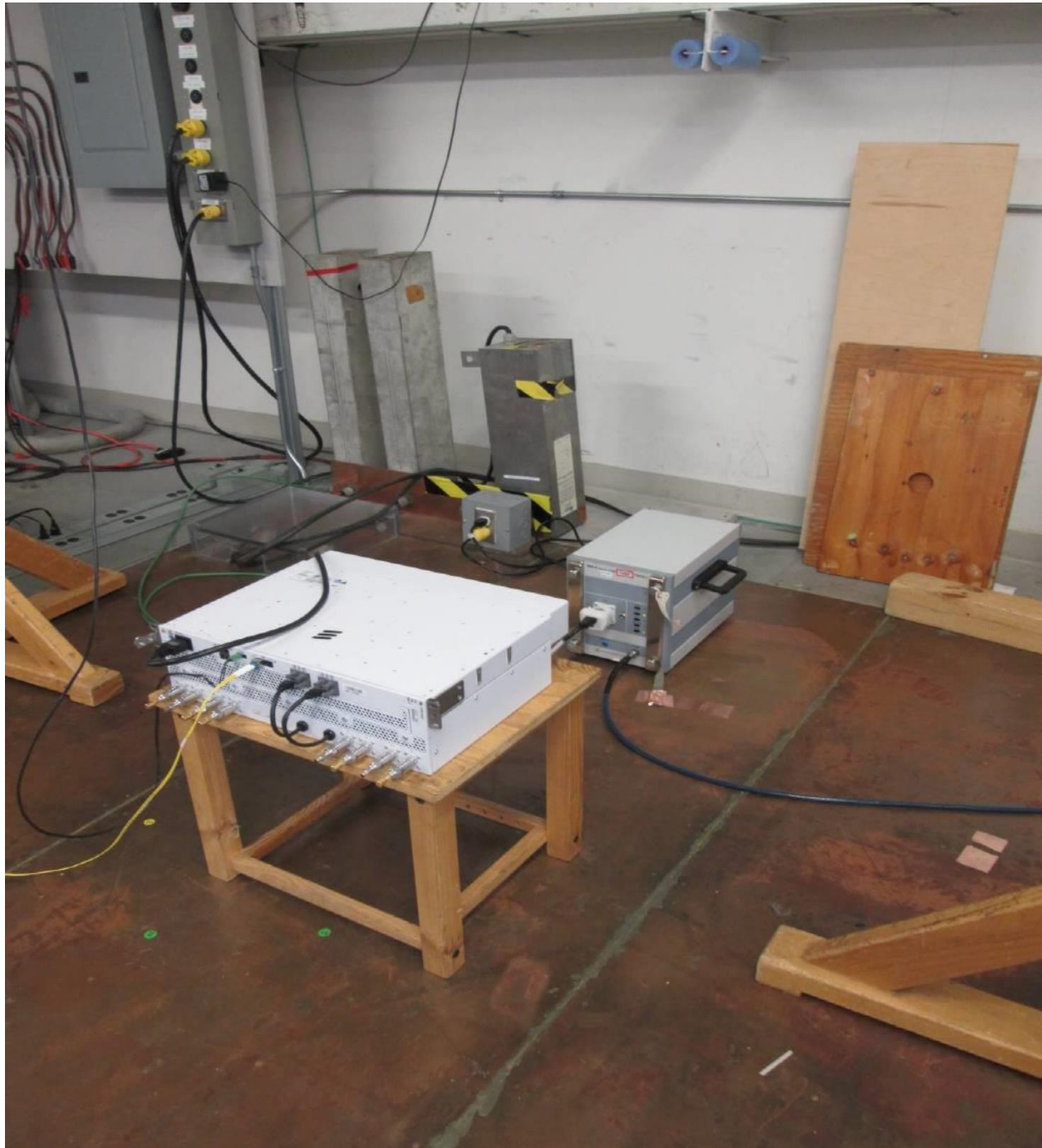
Figure 3: AC Port Conducted Test Equipment
