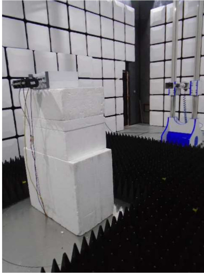
Radiated 1GHz – 8GHz Testing
