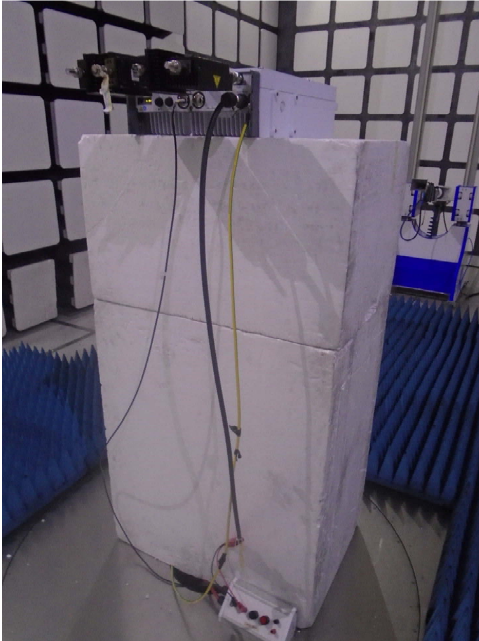
Radiated Testing 1GHz – 18GHz
