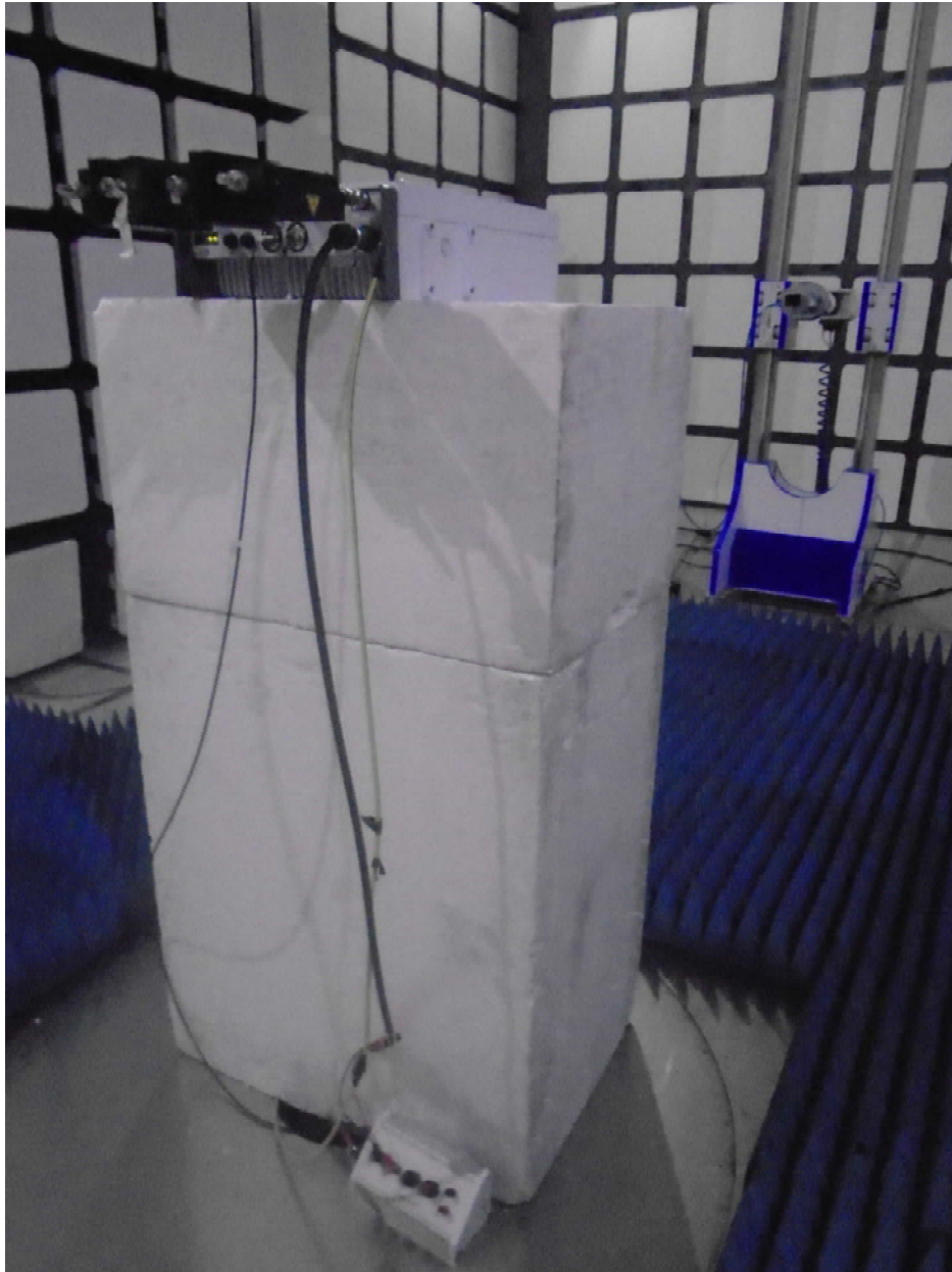
Radiated Testing 18GHz – 22GHz
