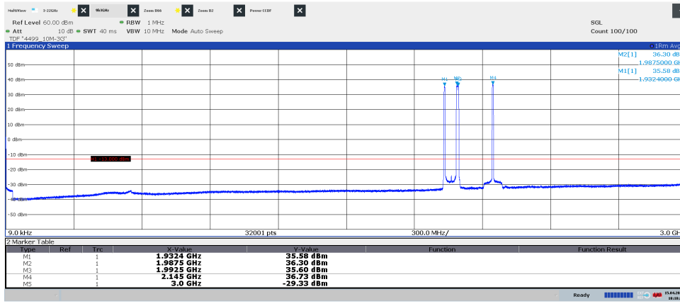
Diagram 3.2a, WCDMA TM1, LTE: E-TM1.1, Tim_{W+L} , 9 kHz – 3 GHz, Port A:
