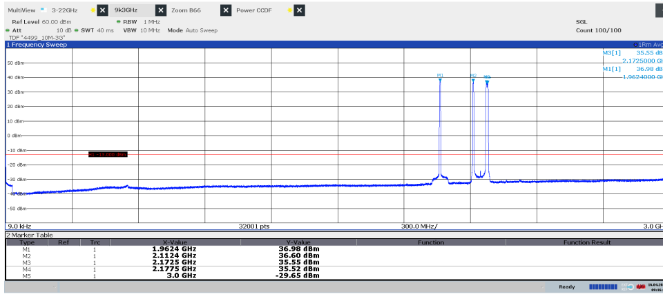
Diagram 3.5a, WCDMA TM1, LTE: E-TM1.1, T_{imW+L} , 9 kHz – 3 GHz, Port B:
