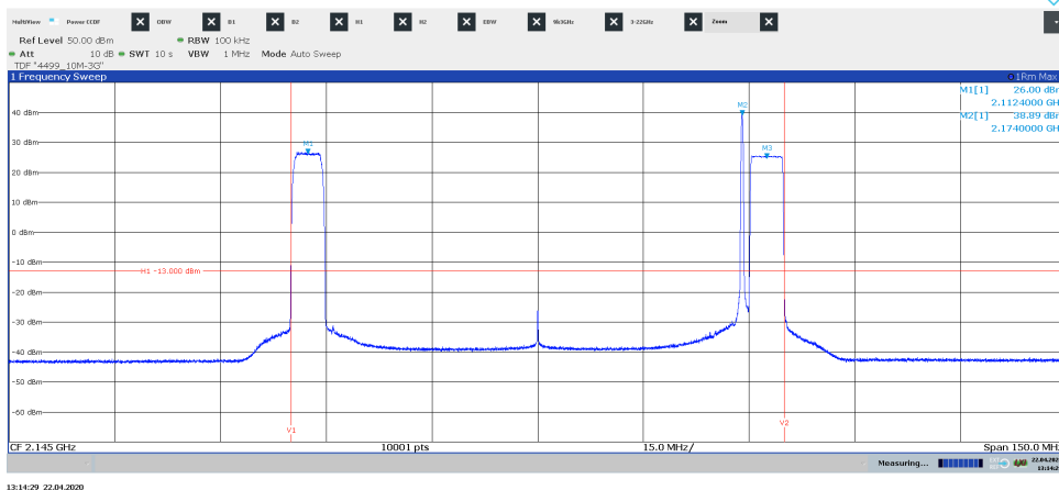
Diagram 3.10b, WCDMA: TM1, LTE: E-TM1.1, T_{imW+L+IoT} , 2.070 GHz – 2.220 GHz, Port B:
