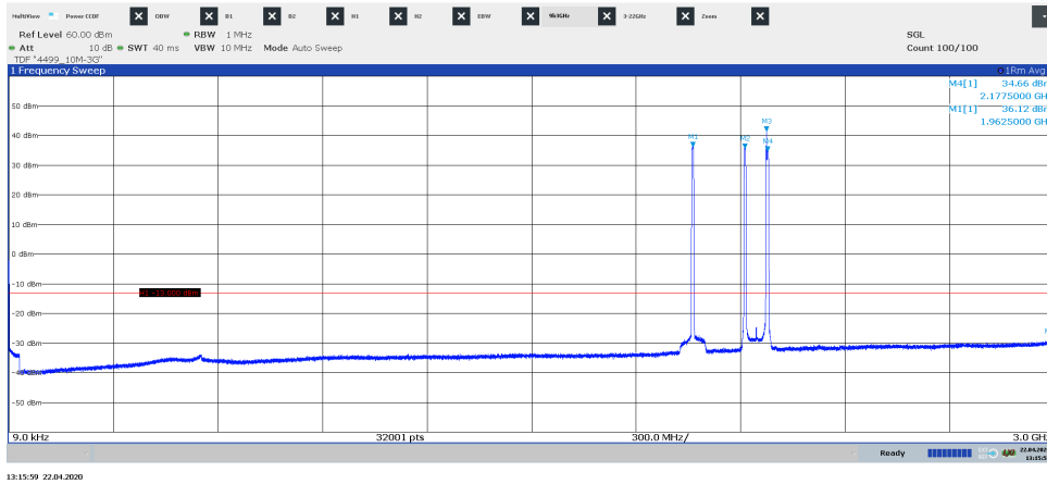
Diagram 3.10a, WCDMA: TM1, LTE: E-TM1.1, T_{imW+L+IoT} , 9 kHz – 3 GHz, Port B:
