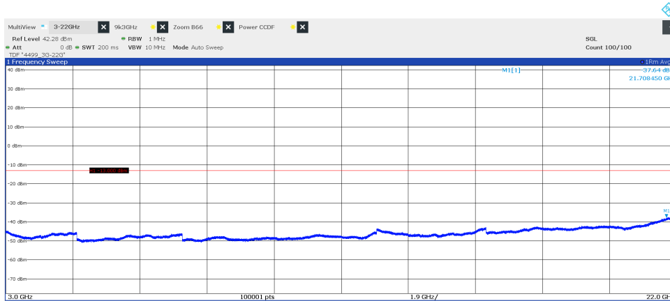
Diagram 3.5c, WCDMA TM1, LTE: E-TM1.1, T_{imW+L} , 3 GHz – 22 GHz, Port B:
