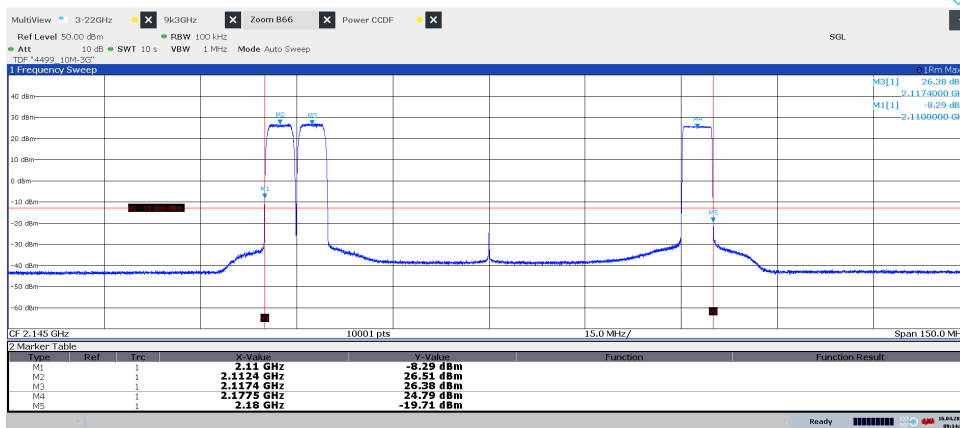
Diagram 3.4b, WCDMA TM1, LTE: E-TM1.1, Bim W+L 2.070 GHz – 2.220 GHz, Port B:
