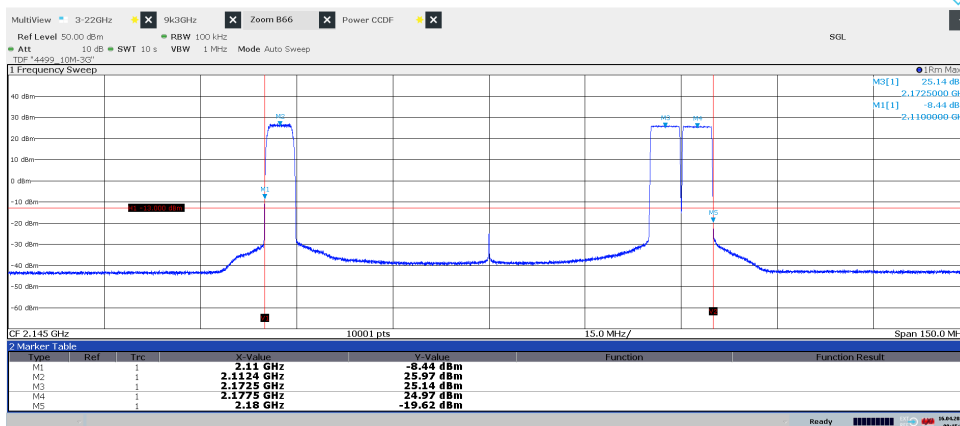
Diagram 3.5b, WCDMA TM1, LTE: E-TM1.1, T_{imW+L} 2.070 GHz – 2.220 GHz, Port B:
