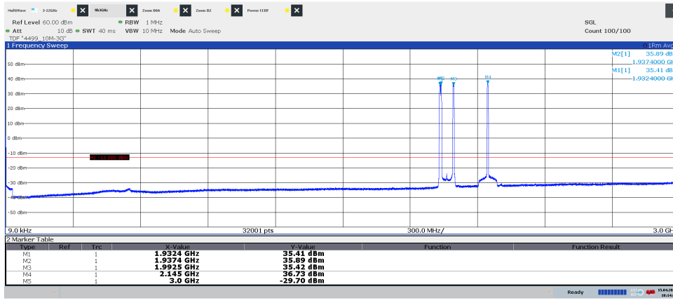
Diagram 3.1a, WCDMA TM1, LTE: E-TM1.1, Bim W+L , 9 kHz – 3 GHz, Port A:
