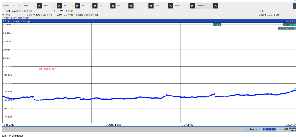
Diagram 3.8c, WCDMA: TM1, LTE: E-TM1.1, T_{imW+L+IoT} , 3 GHz – 22 GHz, Port A:
