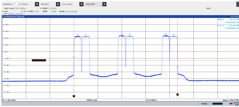
Diagram 3.3b, WCDMA TM1, LTE: E-TM1.1, BMT6, 1.8875 GHz – 2.0375 GHz, Port A:
