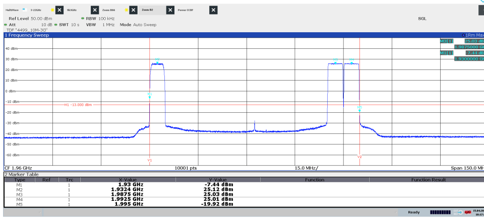
Diagram 3.2b, WCDMA TM1, LTE: E-TM1.1, Tim_{W+L} , 1.8875 GHz – 2.0375 GHz, Port A:
