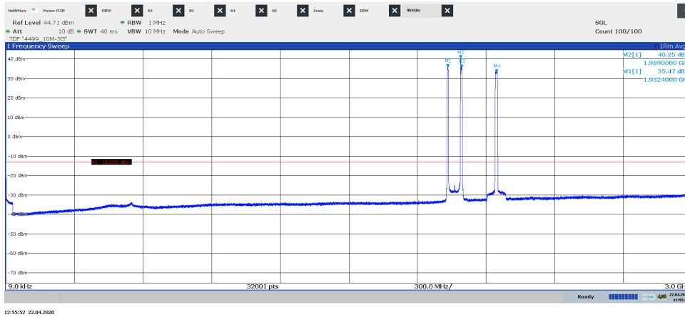
Diagram 3.8a, WCDMA: TM1, LTE: E-TM1.1, T_{imW+L+IoT} , 9 kHz – 3 GHz, Port A:
