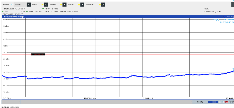
Diagram 3.3c, WCDMA TM1, LTE: E-TM1.1, BMT6, 3 GHz – 22 GHz, Port A:
