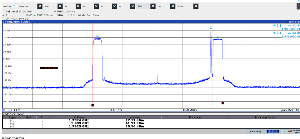
Diagram 3.8b, WCDMA: TM1, LTE: E-TM1.1, T_{imW+L+IoT} , 1.8875 GHz – 2.0375 GHz, Port A:
