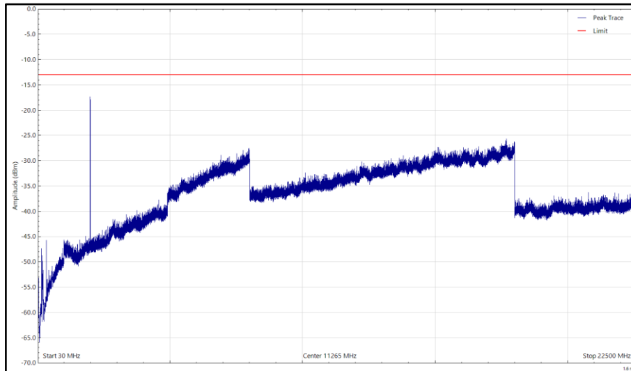
Top - NR&NB-IoT - B25, 1990MHz, 30 MHz to 22.5 GHz, Horizontal (Peak)
