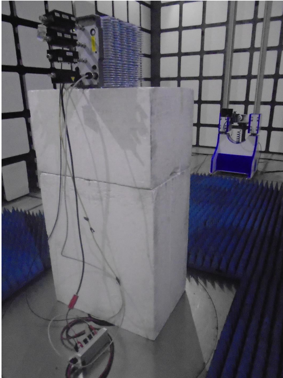
Radiated Testing 1GHz – 8GHz
