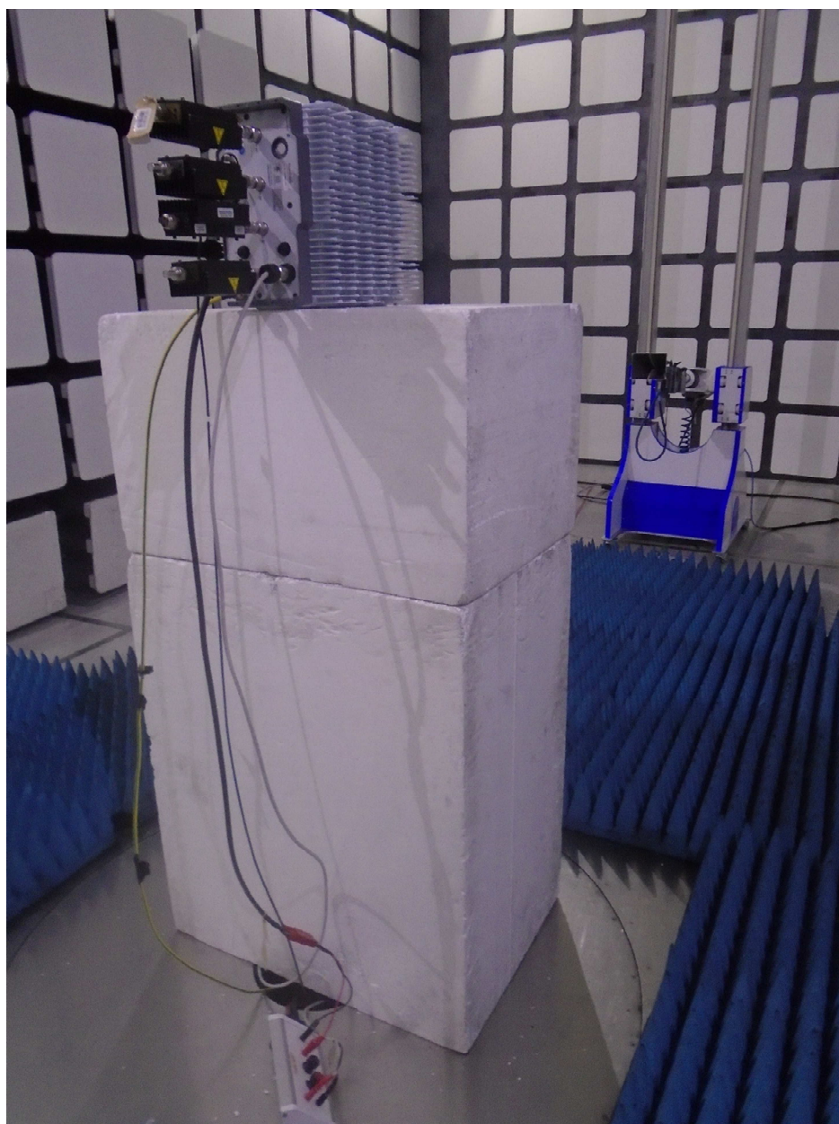
Radiated Testing 1GHz – 10GHz
