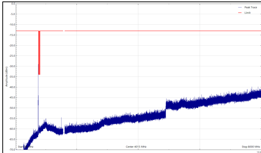
Mid - NR/ESS - B13 - BW10MHz_Po60W, 751MHz, 30 MHz to 8 GHz, Horizontal (Peak)
