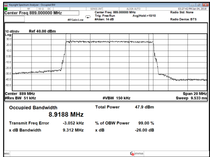
Figure 8.7-30: Occupied bandwidth, QPSK, Port D, high channel, configuration 2
