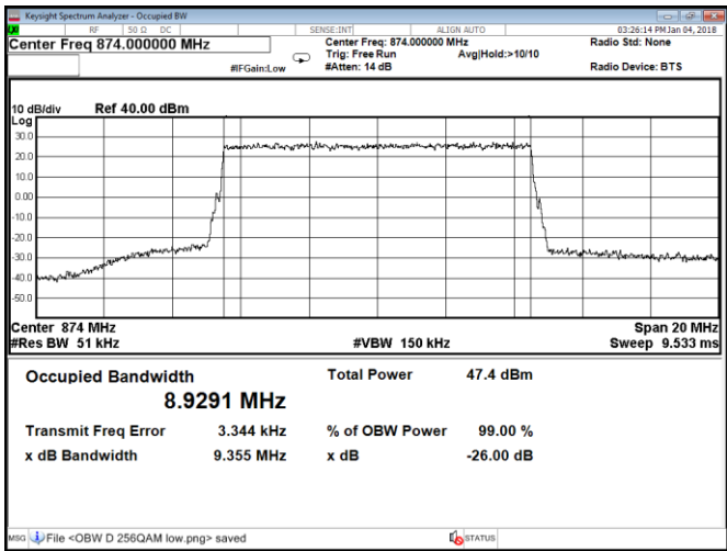
Figure 8.7-35: Occupied bandwidth, 256QAM, Port A, low channel, configuration 2
