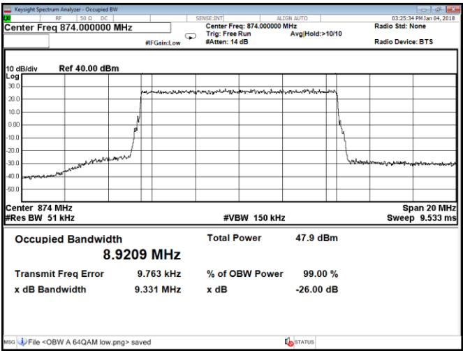
Figure 8.7-34: Occupied bandwidth, 64QAM, Port D, low channel, configuration 2
