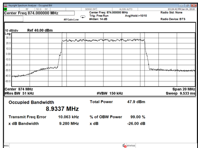
Figure 8.7-32: Occupied bandwidth, 16QAM, Port D, low channel, configuration 2
