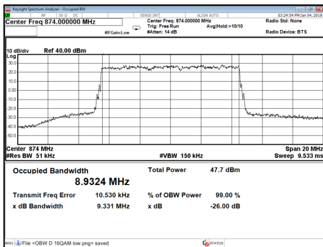
Figure 8.7-31: Occupied bandwidth, 16QAM, Port A, low channel, configuration 2
