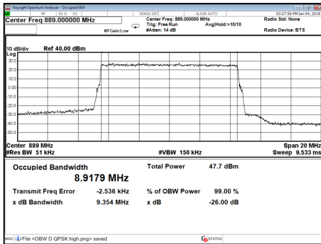
Figure 8.7-29: Occupied bandwidth, QPSK, Port A, high channel, configuration 2
