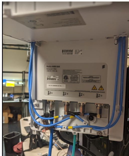
Figure 1.1-2: EUT photo
