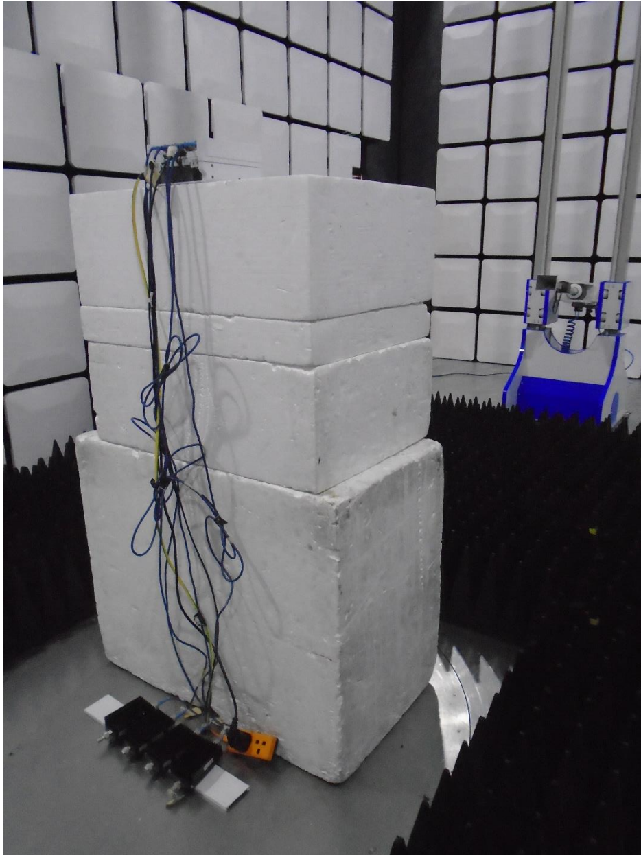
Radiated Emissions 8GHz-18GHz
