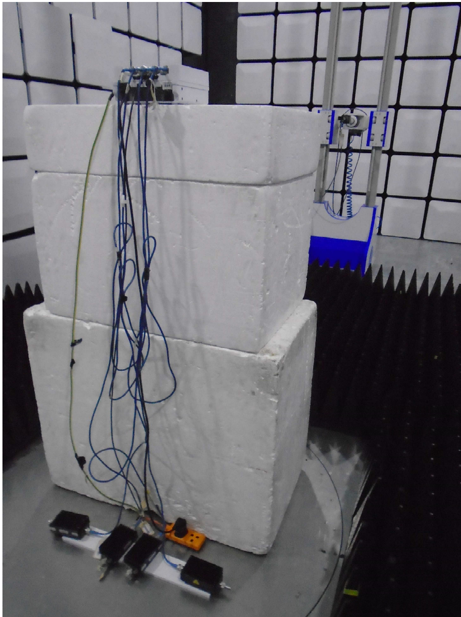
Radiated Emissions 18GHz-25GHz
