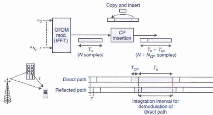
Figure 3 Cyclic-prefix insertion
