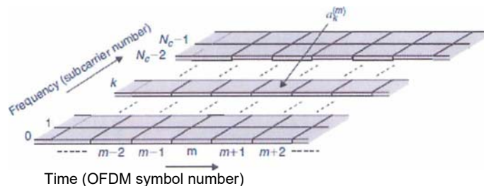
Figure 2 OFDM time-frequency grids
