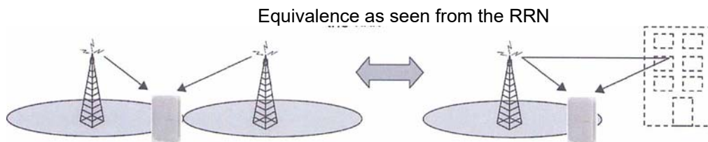
Figure 4 Equivalence between simulcast transmission and multi-path propagation
