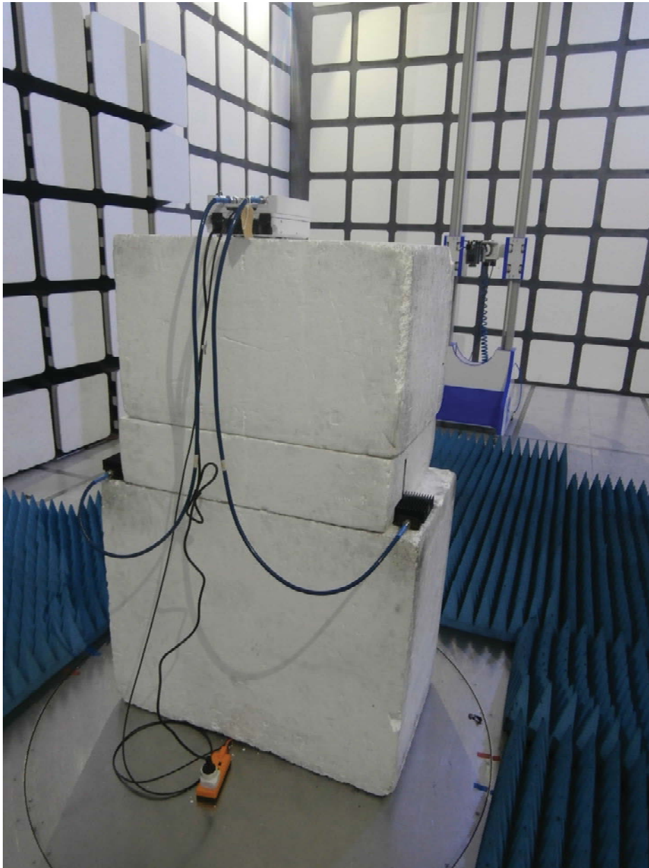
Radiated Emissions 18 GHz to 40 GHz
