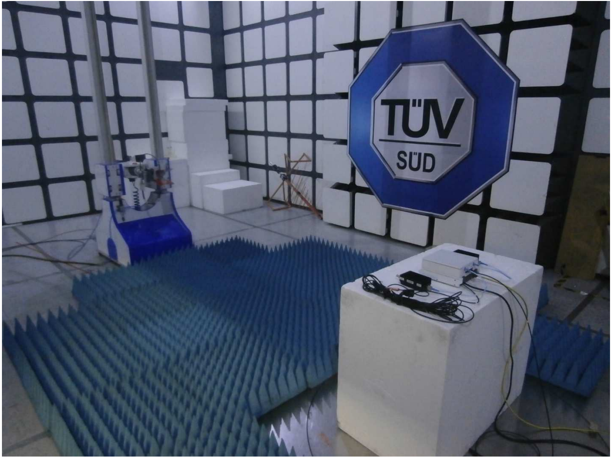
Radiated Emissions 1 GHz to 18 GHz
