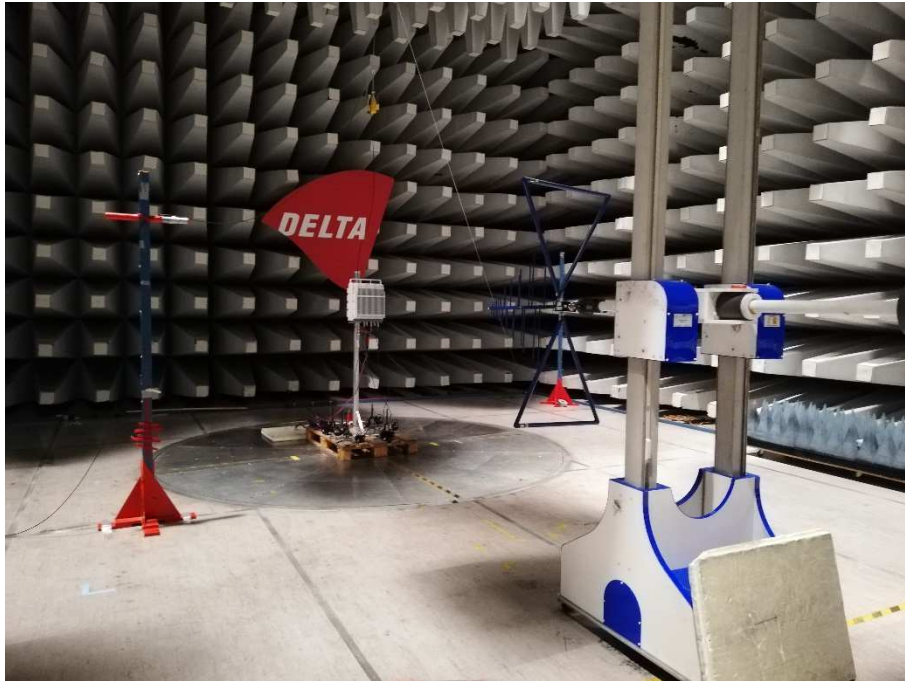
Radiated Emissions 30MHz- 1GHz Testing
