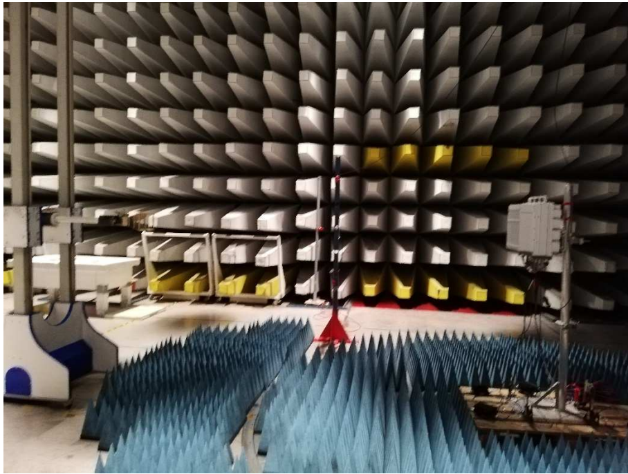
Radiated Emissions 8GHz- 18GHz Testing
