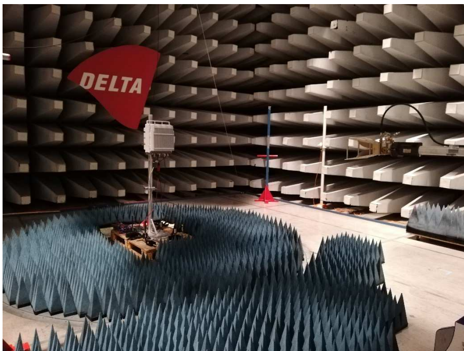
Radiated Emissions 1GHz- 8GHz Testing
