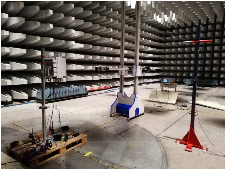
Radiated Emissions 18GHz- 22GHz Testing
