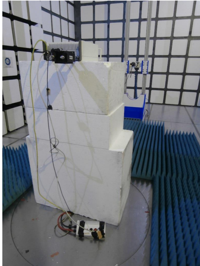
Radiated Emissions 18 GHz to 20 GHz
