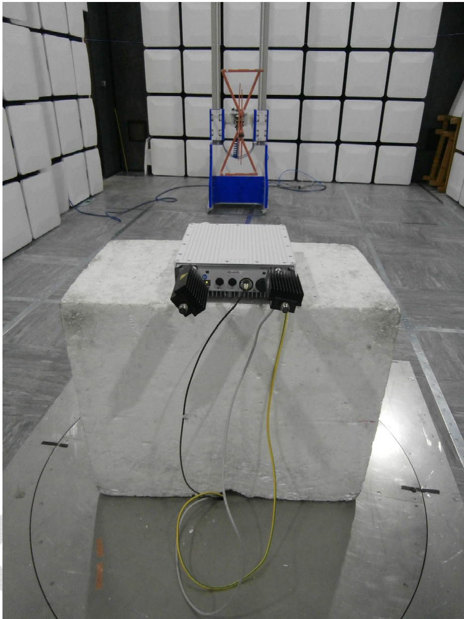
FCC Part 27 - Radiated Testing – 30MHz – 1GHz
