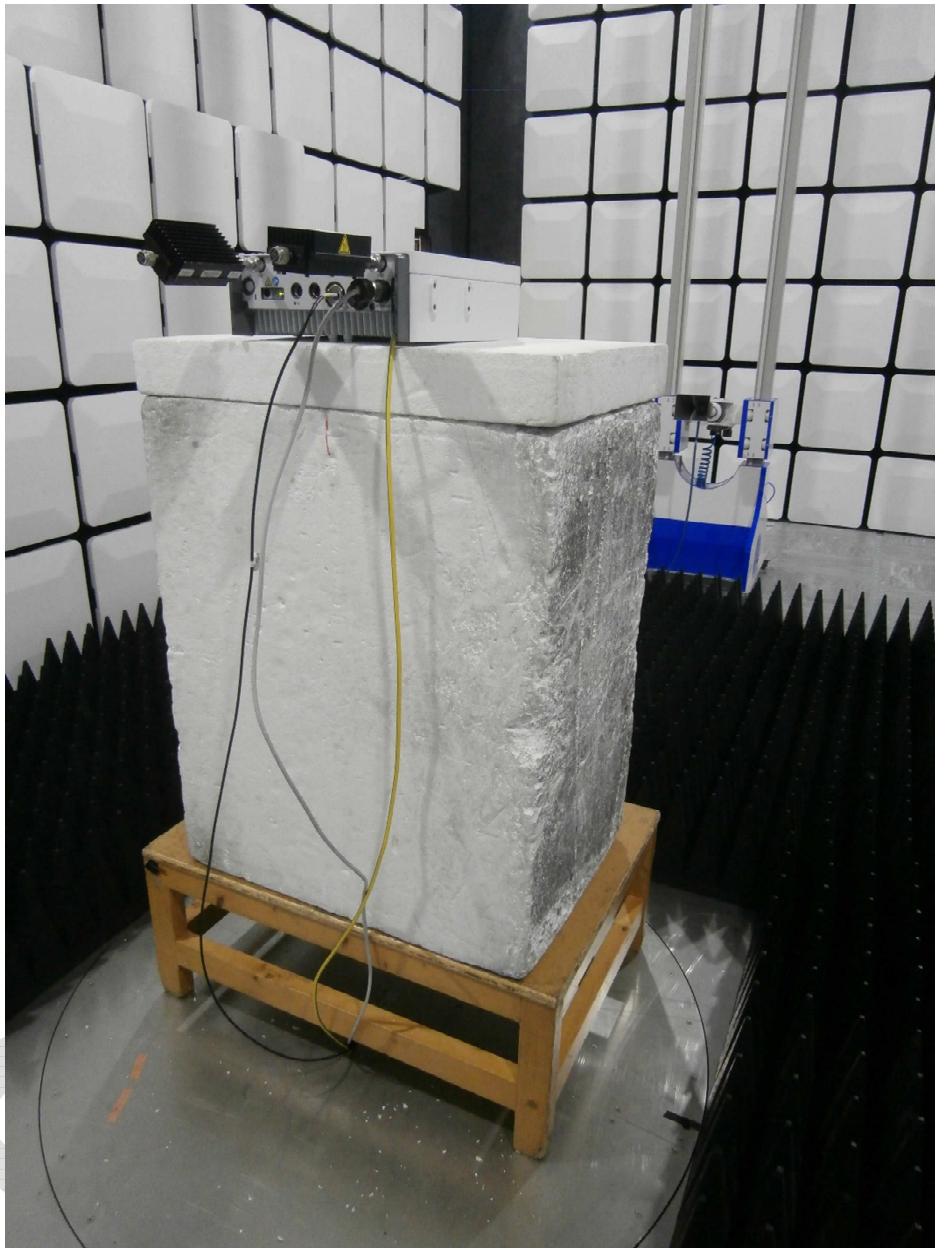
FCC Part 27 - Radiated Testing – 1GHz – 10GHz
