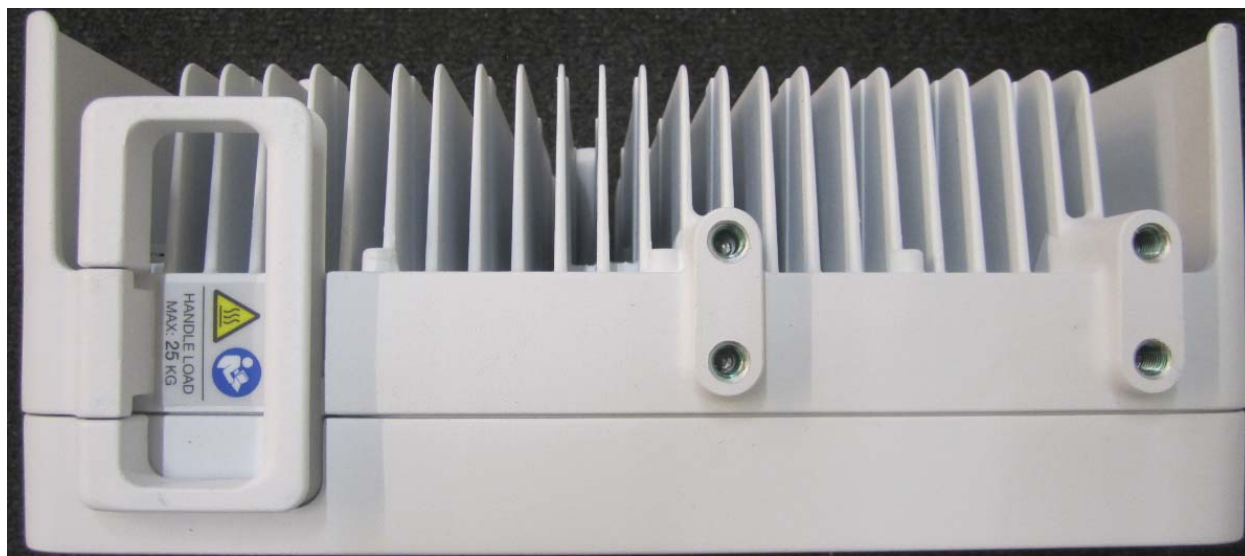
Figure 4: Radio 4415 B66A Top View
