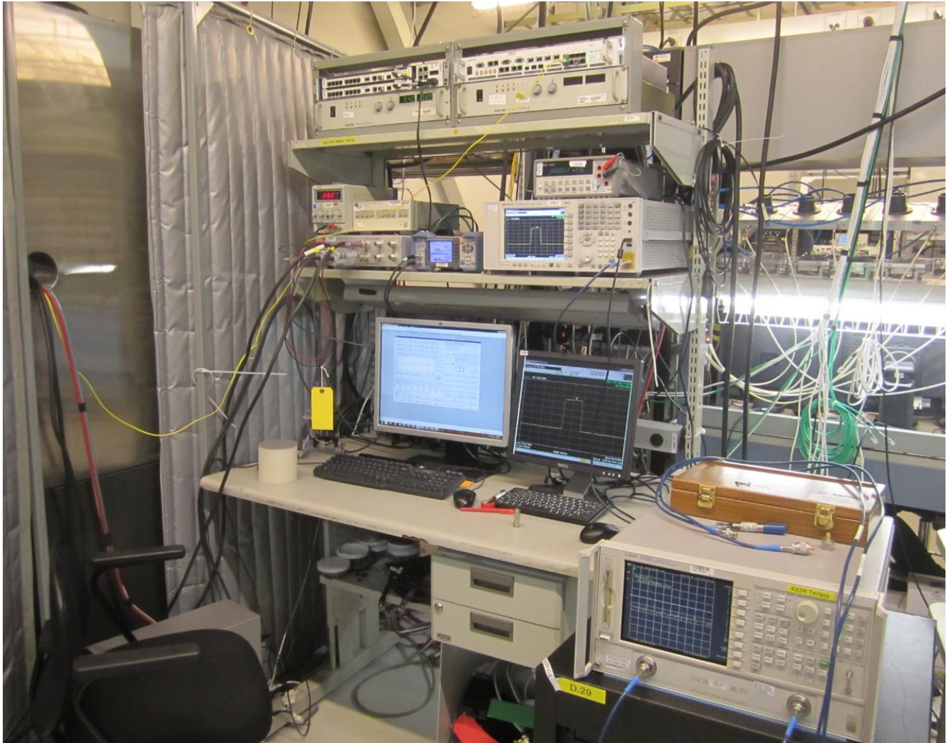
Test / Measurement Equipment - Set up for Radio Compliance Testing
